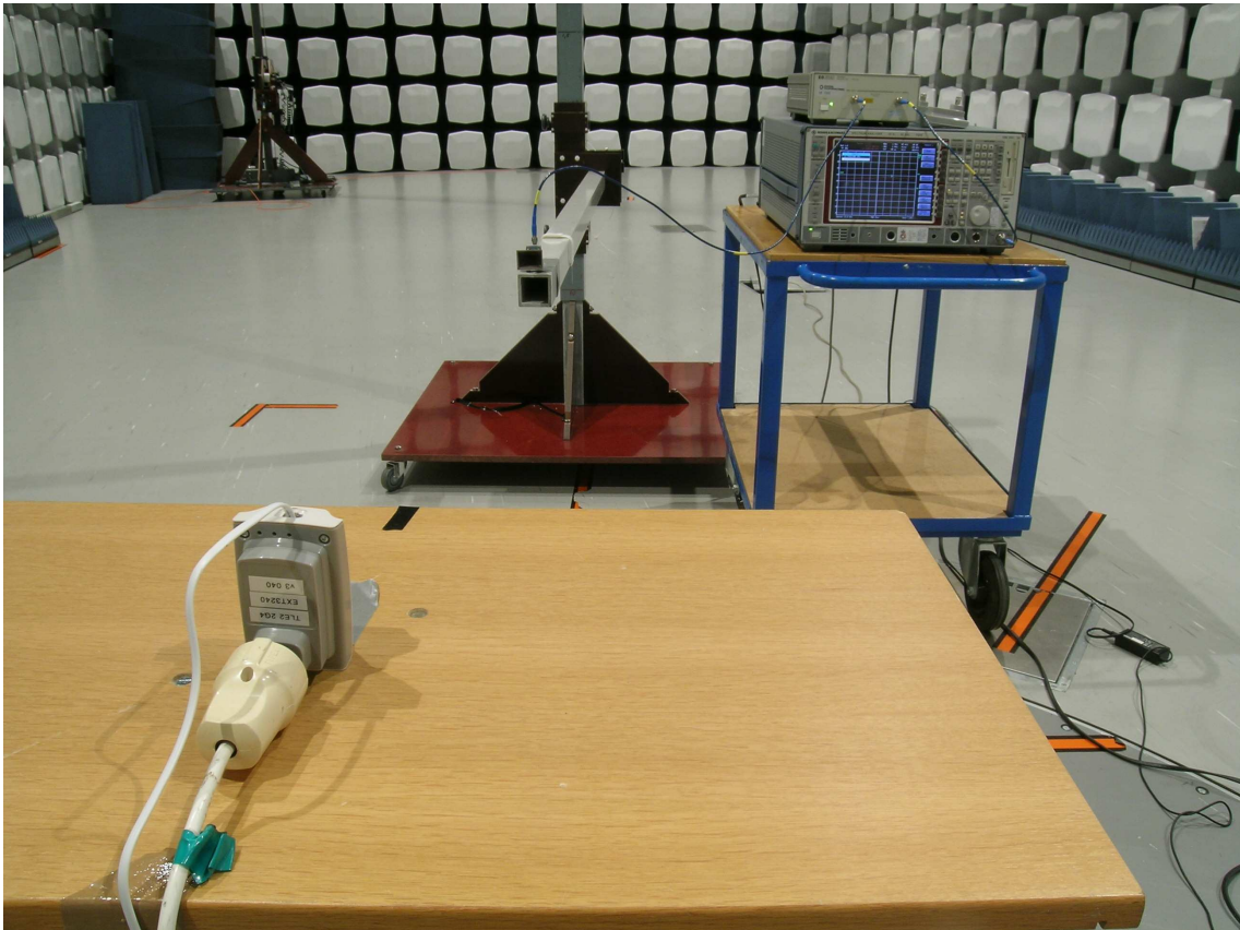
Radiated Emissions 18-25 GHz
