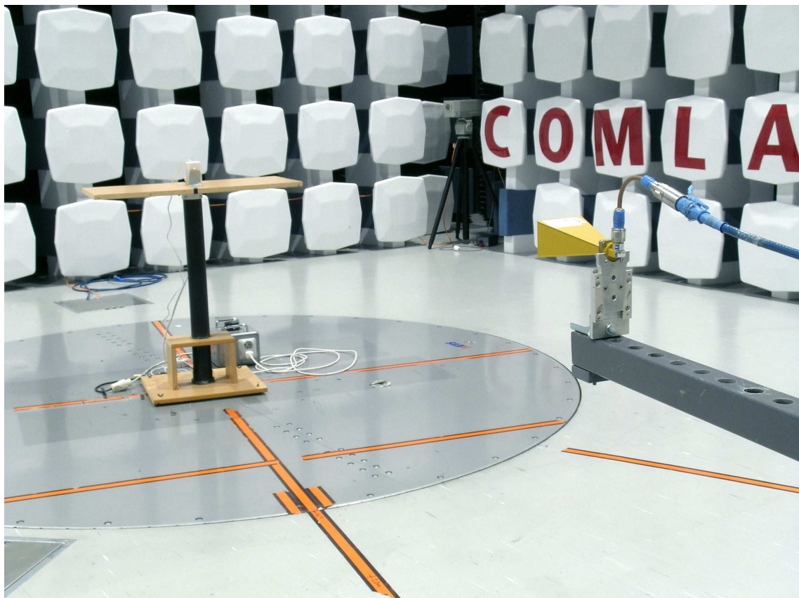
Radiated emissions above 1 GHz
