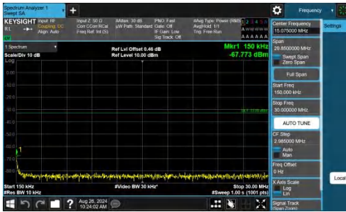
Band2-15MHz-QPSK-19125-1RB#74-0.15~30-PASS
