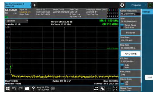
Band2-10MHz-QPSK-18650-1RB#0-0.15~30-PASS
