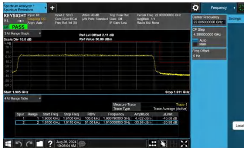
Band2-5MHz-QPSK-19175-25RB#0-PASS
