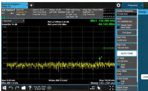
Band2-1.4MHz-QPSK-18607-1RB#0-0.009~0.15-PASS
