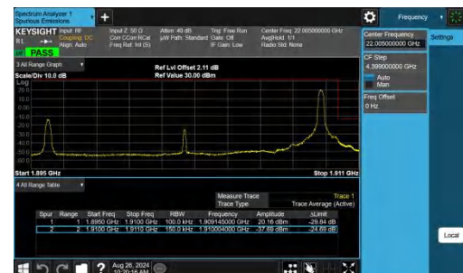
Band2-15MHz-QPSK-19125-1RB#74-PASS
