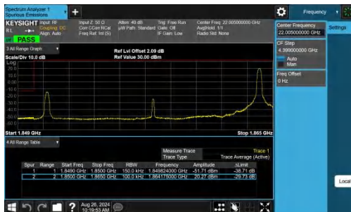
Band2-15MHz-QPSK-18675-1RB#74-PASS
