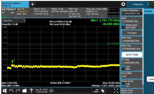
Band2-15MHz-QPSK-19125-1RB#0-3000~20000-PASS
