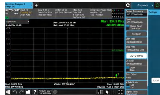
Band2-10MHz-QPSK-19150-1RB#49-30~1000-PASS
