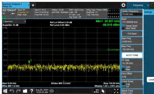
Band2-15MHz-QPSK-19125-1RB#0-0.009~0.15-PASS
