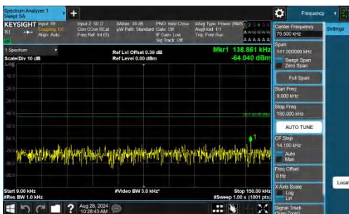
Band2-20MHz-QPSK-18700-1RB#0-0.009~0.15-PASS
