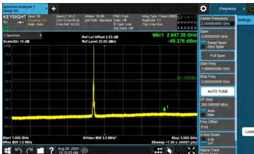
Band2-10MHz-QPSK-18900-1RB#49-1000~3000-PASS
