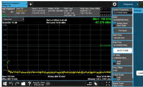
Band2-1.4MHz-QPSK-19193-1RB#5-0.15~30-PASS
