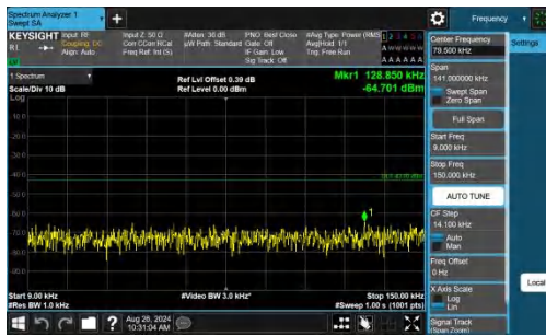
Band2-20MHz-QPSK-19100-1RB#0-0.009~0.15-PASS
