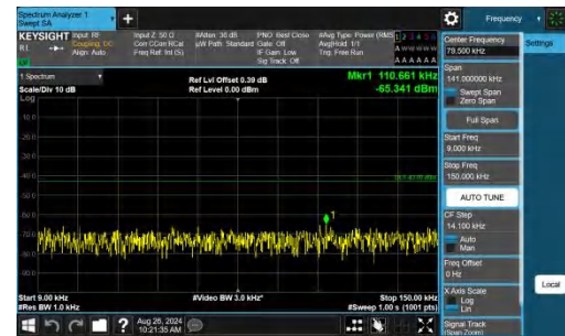
Band2-15MHz-QPSK-18675-1RB#74-0.009~0.15-PASS
