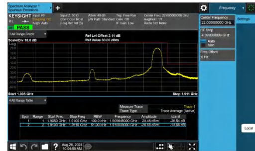
Band2-5MHz-QPSK-19175-1RB#24-PASS
