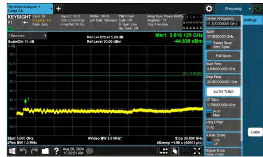
Band2-20MHz-QPSK-19100-1RB#99-3000~20000-PASS
