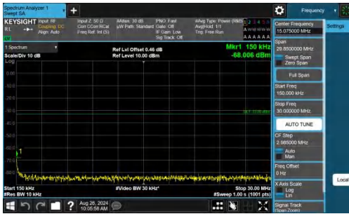
Band2-5MHz-QPSK-18625-1RB#24-0.15~30-PASS
