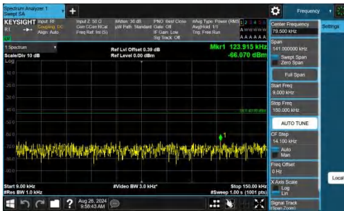
Band2-3MHz-QPSK-18900-1RB#0-0.009~0.15-PASS
