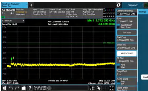
Band2-20MHz-QPSK-18900-1RB#0-3000~20000-PASS
