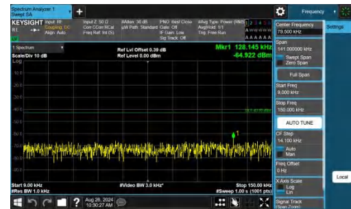
Band2-20MHz-QPSK-18900-1RB#99-0.009~0.15-PASS
