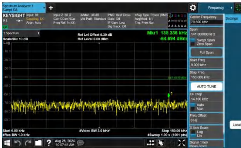
Band2-5MHz-QPSK-19175-1RB#0-0.009~0.15-PASS
