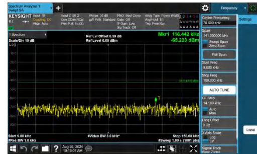
Band2-10MHz-QPSK-18900-1RB#49-0.009~0.15-PASS
