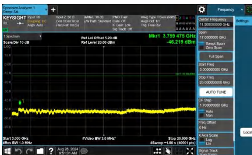
Band2-1.4MHz-QPSK-18900-1RB#0-3000~20000-PASS
