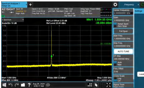
Band2-1.4MHz-QPSK-18607-1RB#5-1000~3000-PASS
