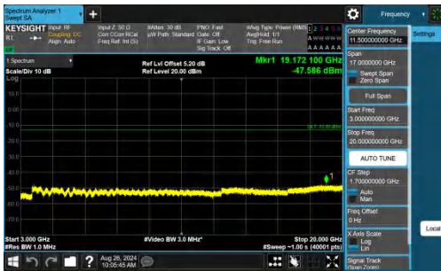
Band2-5MHz-QPSK-18625-1RB#0-3000~20000-PASS
