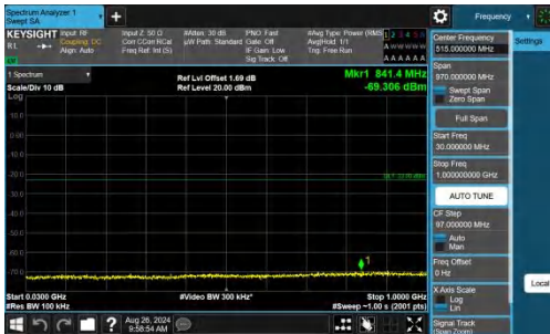
Band2-3MHz-QPSK-18900-1RB#0-30~1000-PASS
