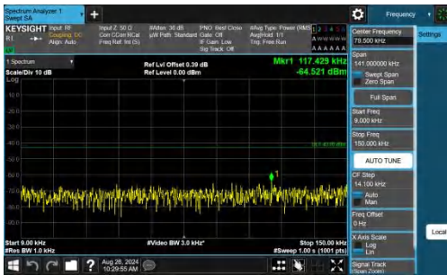
Band2-20MHz-QPSK-18900-1RB#0-0.009~0.15-PASS
