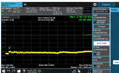
Band2-15MHz-QPSK-18900-1RB#0-3000~20000-PASS
