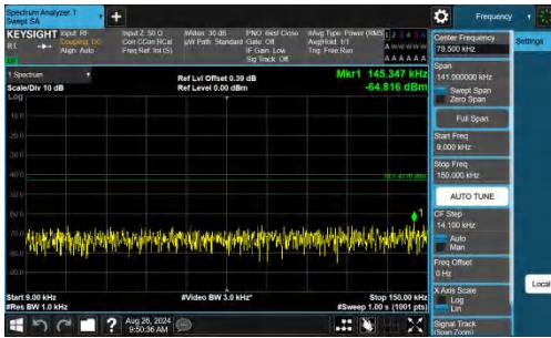
Band2-1.4MHz-QPSK-18900-1RB#0-0.009~0.15-PASS
