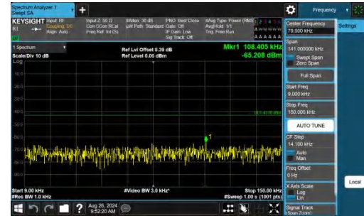
Band2-1.4MHz-QPSK-19193-1RB#5-0.009~0.15-PASS
