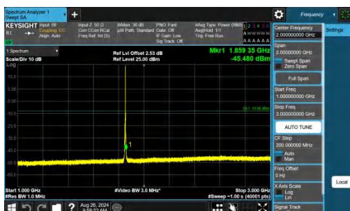
Band2-3MHz-QPSK-18615-1RB#14-1000~3000-PASS
