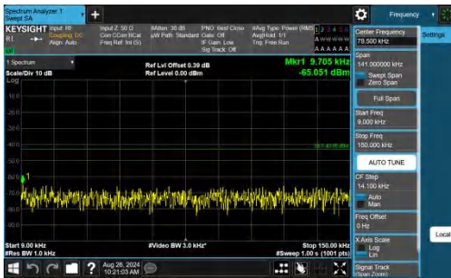
Band2-15MHz-QPSK-18675-1RB#0-0.009~0.15-PASS
