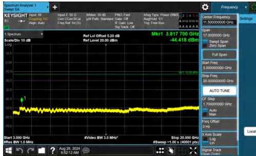
Band2-1.4MHz-QPSK-19193-1RB#0-3000~20000-PASS
