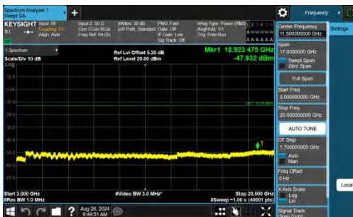
Band2-1.4MHz-QPSK-18607-1RB#0-3000~20000-PASS
