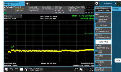
Band2-15MHz-QPSK-18900-1RB#74-3000~20000-PASS
