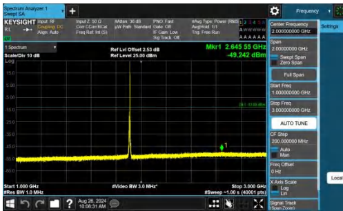
Band2-5MHz-QPSK-19175-1RB#24-1000~3000-PASS
