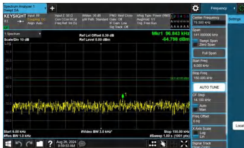
Band2-3MHz-QPSK-19185-1RB#0-0.009~0.15-PASS
