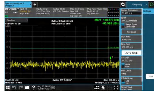
Band2-10MHz-QPSK-19150-1RB#49-0.009~0.15-PASS
