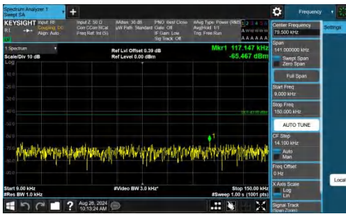
Band2-10MHz-QPSK-18650-1RB#0-0.009~0.15-PASS
