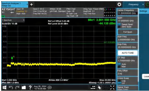
Band2-10MHz-QPSK-19150-1RB#0-3000~20000-PASS
