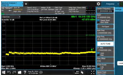
Band2-10MHz-QPSK-18900-1RB#0-3000~20000-PASS
