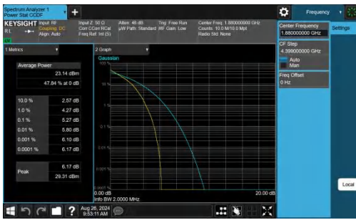
Band2-1.4MHz-QPSK-18900-6RB#0-PASS
