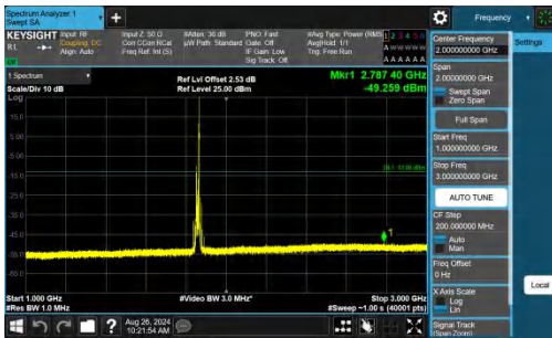
Band2-15MHz-QPSK-18675-1RB#74-1000~3000-PASS
