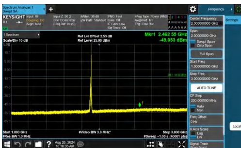
Band2-10MHz-QPSK-19150-1RB#49-1000~3000-PASS
