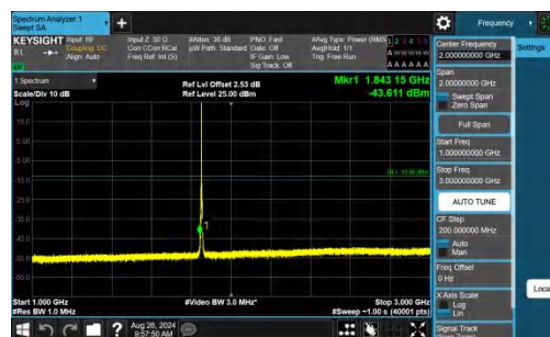
Band2-3MHz-QPSK-18615-1RB#0-1000~3000-PASS
