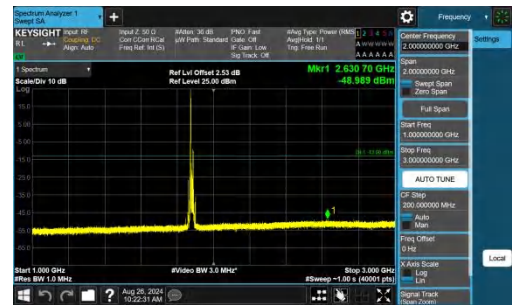
Band2-15MHz-QPSK-18900-1RB#0-1000~3000-PASS
