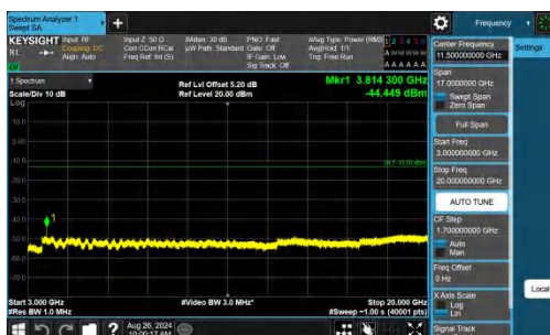
Band2-3MHz-QPSK-19185-1RB#0-3000~20000-PASS
