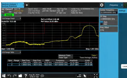
Band2-1.4MHz-QPSK-18607-1RB#5-PASS
