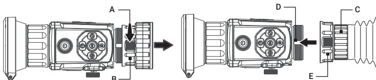
FIGURE 2-10. EYEPiece REPLACEMENT
