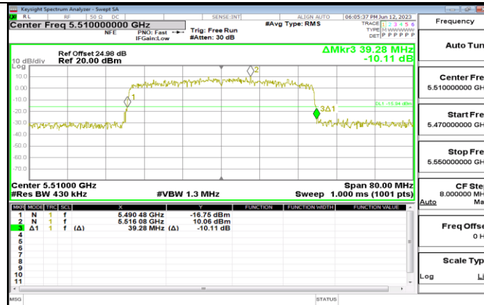
11AX40-TX BEAMFORMING Ant1 5510
