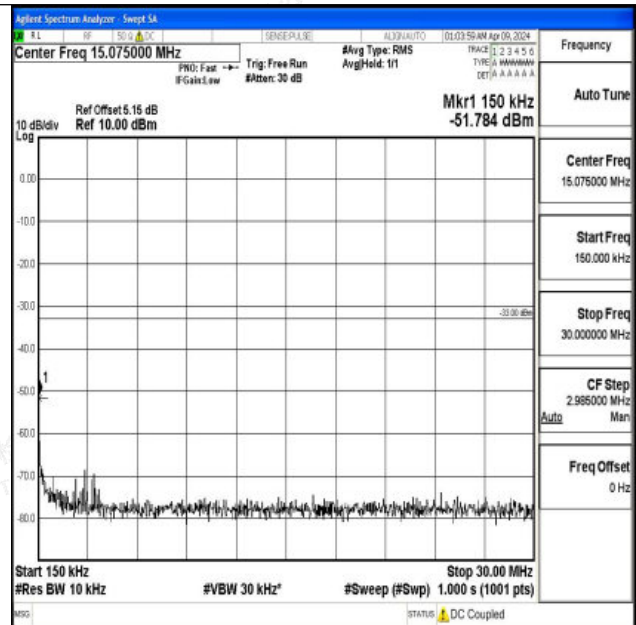
Band2_15MHz_QPSK_18675_1RB#0_0.15~30_0.15~30
