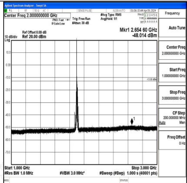
Band2_15MHz_QPSK_19125_1RB#0_1000~3000_1000~3000
