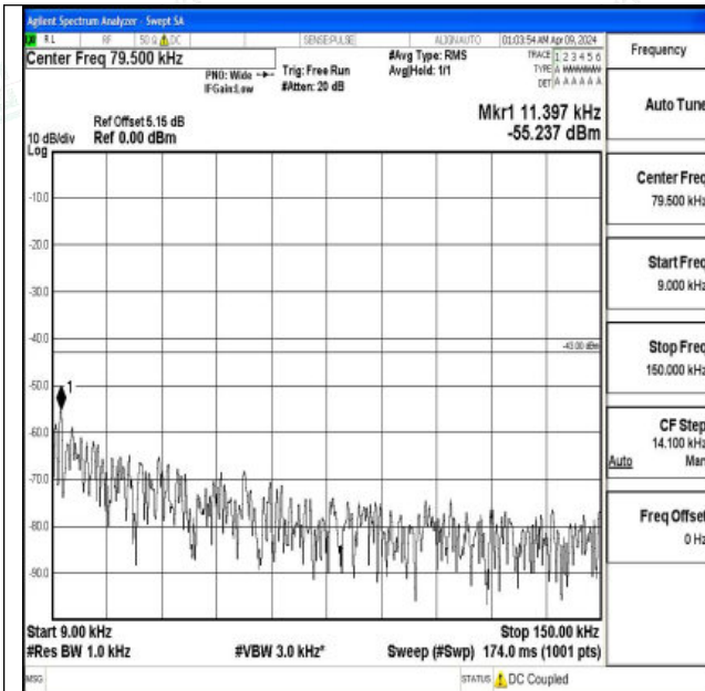
Band2_15MHz_QPSK_18675_1RB#0_0.009~0.15_0.009~0.15
