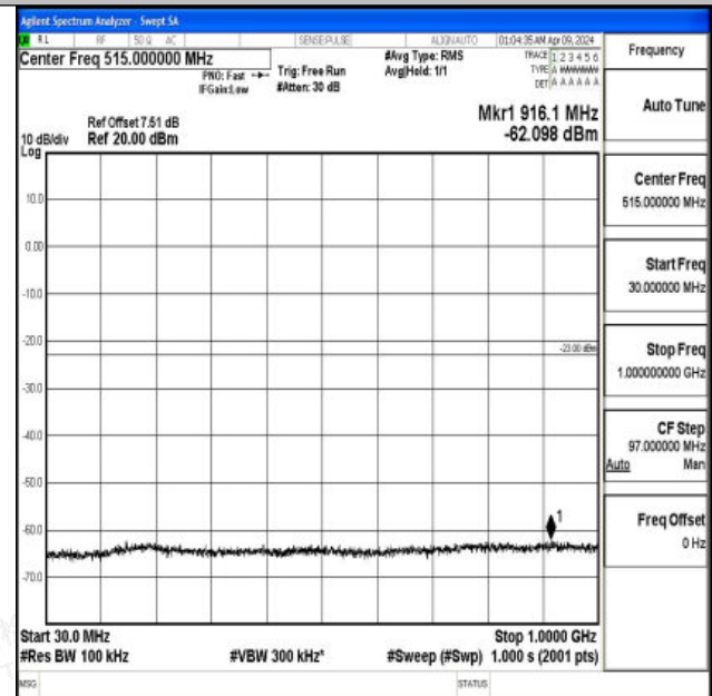
Band2_15MHz_16QAM_18675_1RB#0_30~1000_30~1000
