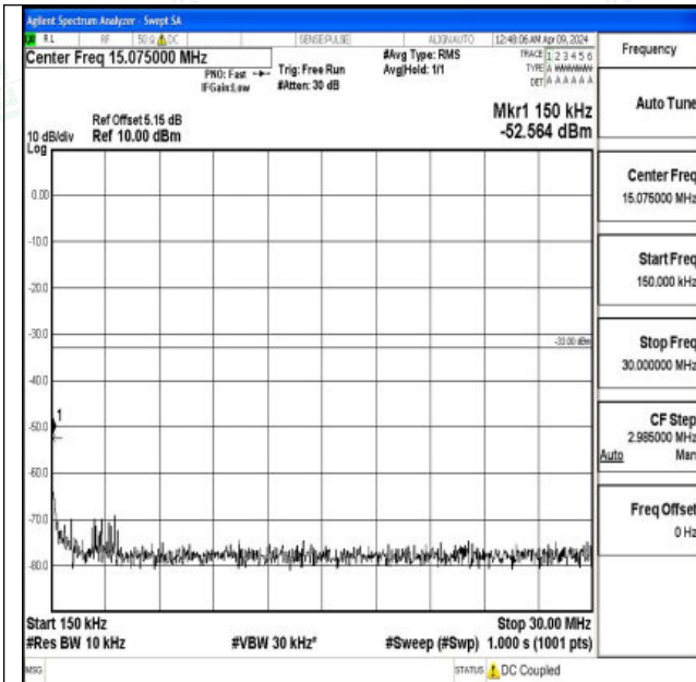
Band2_10MHz_16QAM_18650_1RB#0_0.15~30_0.15~30
