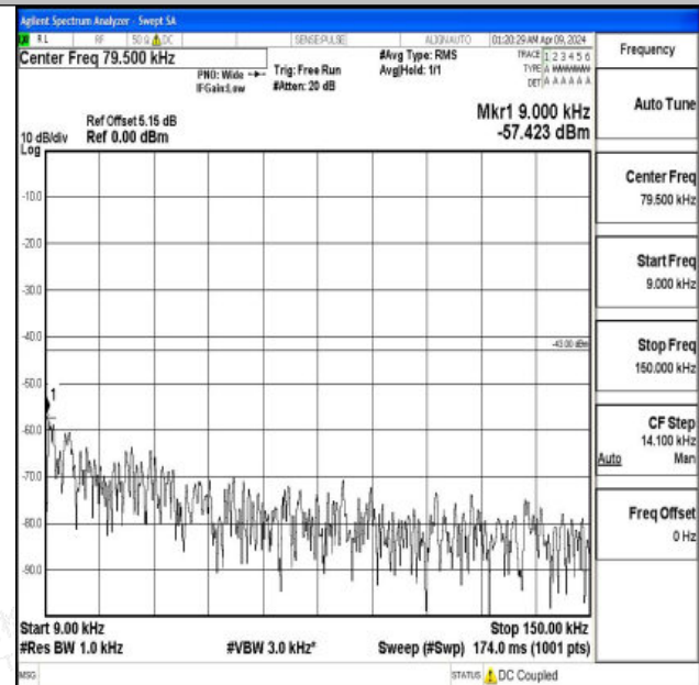
Band2_20MHz_16QAM_18700_1RB#0_0.009~0.15_0.009~0.15
