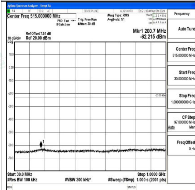
Band2_20MHz_QPSK_18900_1RB#0_30~1000_30~1000
