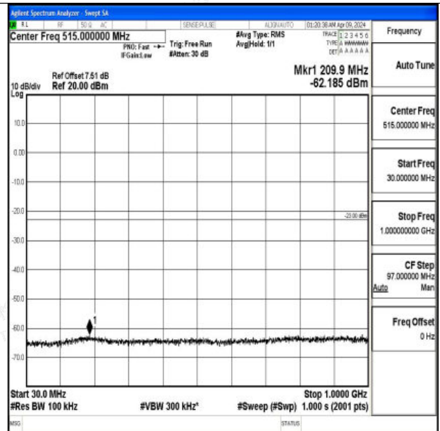
Band2_20MHz_16QAM_18700_1RB#0_30~1000_30~1000
