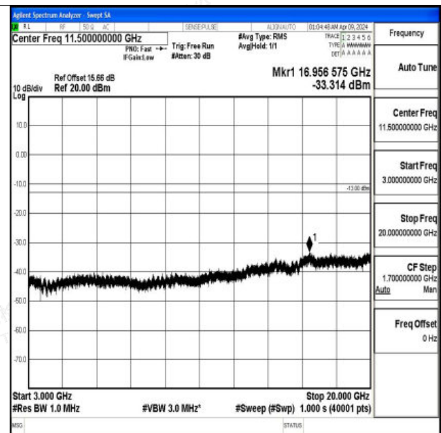
Band2_15MHz_16QAM_18675_1RB#0_3000~20000_3000 ~20000
