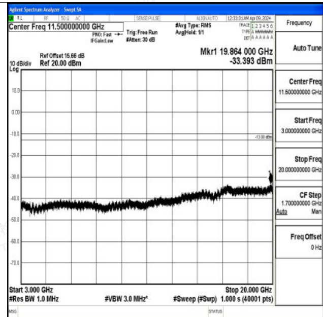
Band2_5MHz_16QAM_19175_1RB#0_3000~20000_3000~20000
