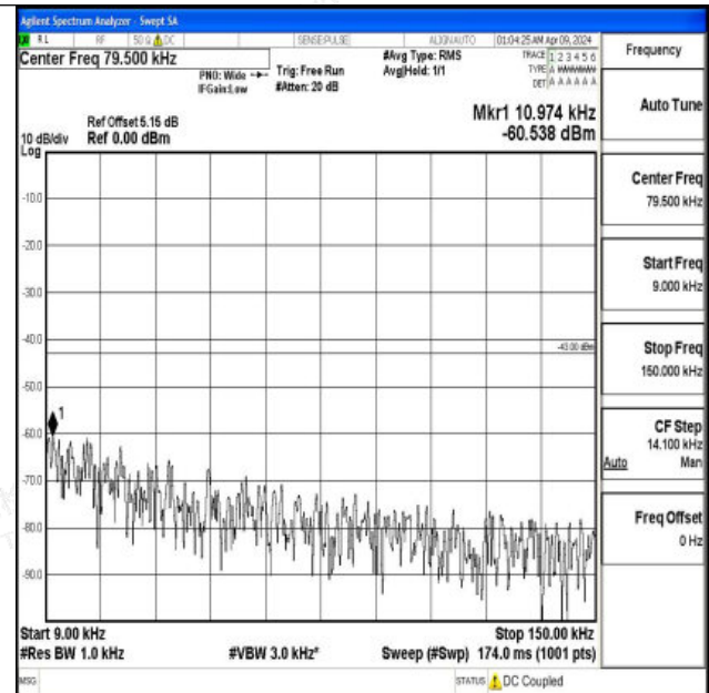
Band2_15MHz_16QAM_18675_1RB#0_0.009~0.15_0.009~0.15
