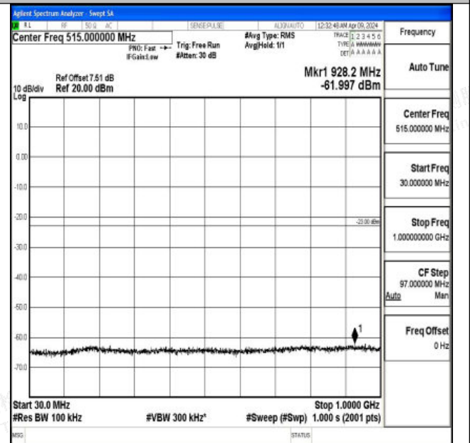
Band2_5MHz_16QAM_19175_1RB#0_30~1000_30~1000
