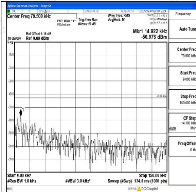
Band2_15MHz_QPSK_19125_1RB#0_0.009~0.15_0.009~0.15
