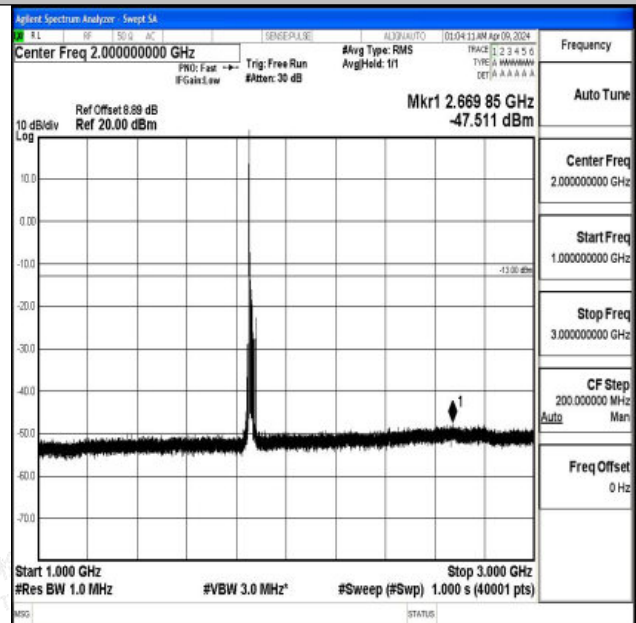
Band2_15MHz_QPSK_18675_1RB#0_1000~3000_1000~3000
