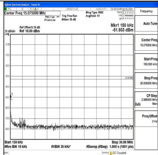
Band2_20MHz_QPSK_18700_1RB#0_0.15~30_0.15~30
