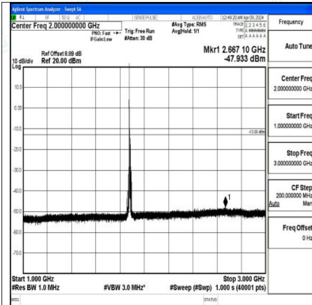
Band2_10MHz_16QAM_18900_1RB#0_1000~3000_1000 ~3000
