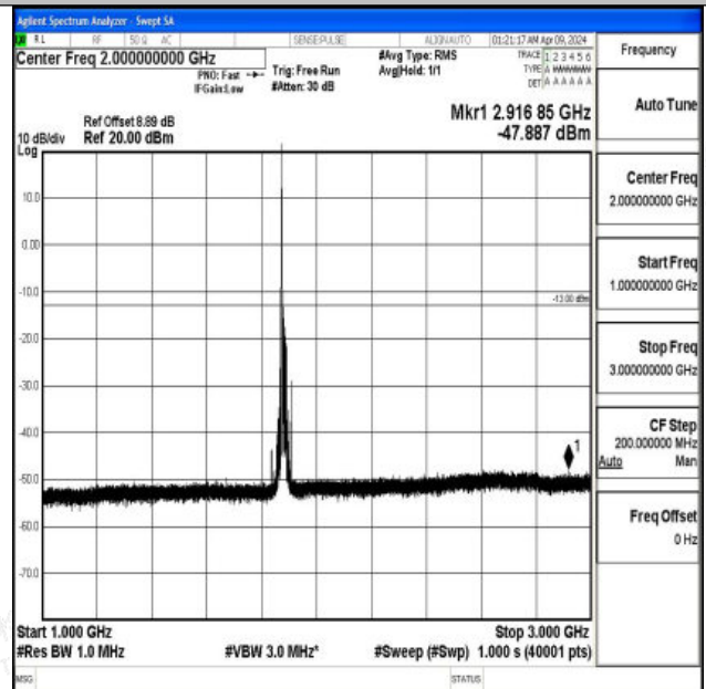
Band2_20MHz_QPSK_18900_1RB#0_1000~3000_1000~3000
