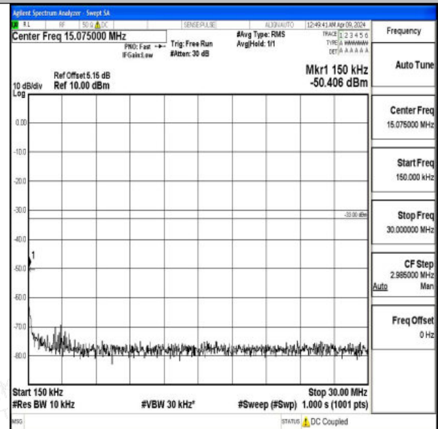
Band2_10MHz_QPSK_19150_1RB#0_0.15~30_0.15~30
