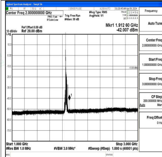
Band2_20MHz_16QAM_18700_1RB#0_1000~3000_1000 ~3000
