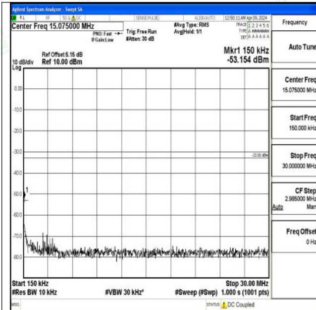
Band2_10MHz_16QAM_19150_1RB#0_0.15~30_0.15~30
