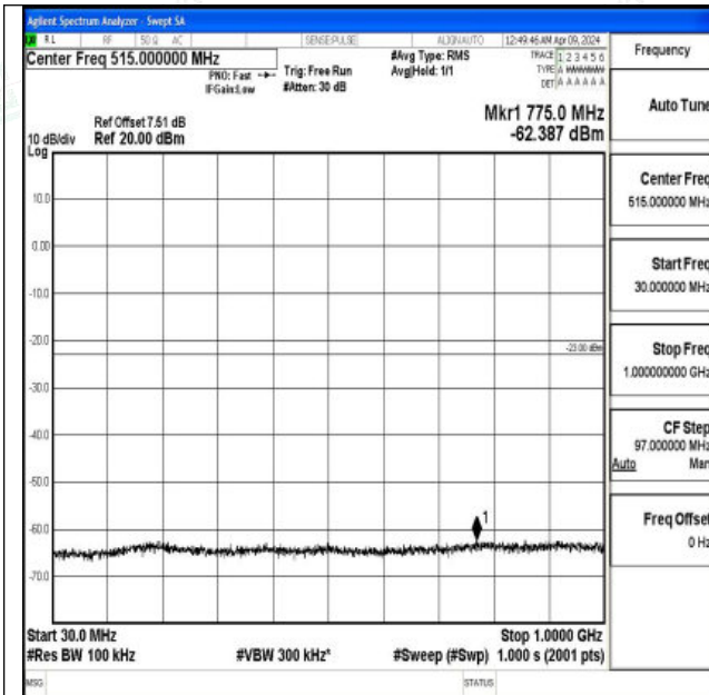
Band2_10MHz_QPSK_19150_1RB#0_30~1000_30~1000
