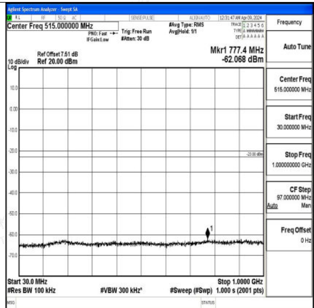
Band2_5MHz_16QAM_18900_1RB#0_30~1000_30~1000
