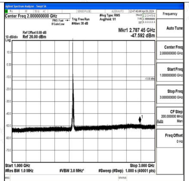
Band2_10MHz_QPSK_18650_1RB#0_1000~3000_1000~3000
