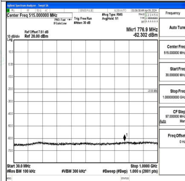
Band2_15MHz_QPSK_19125_1RB#0_30~1000_30~1000
