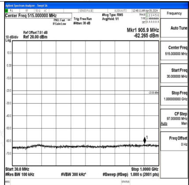
Band2_10MHz_16QAM_18650_1RB#0_30~1000_30~1000
