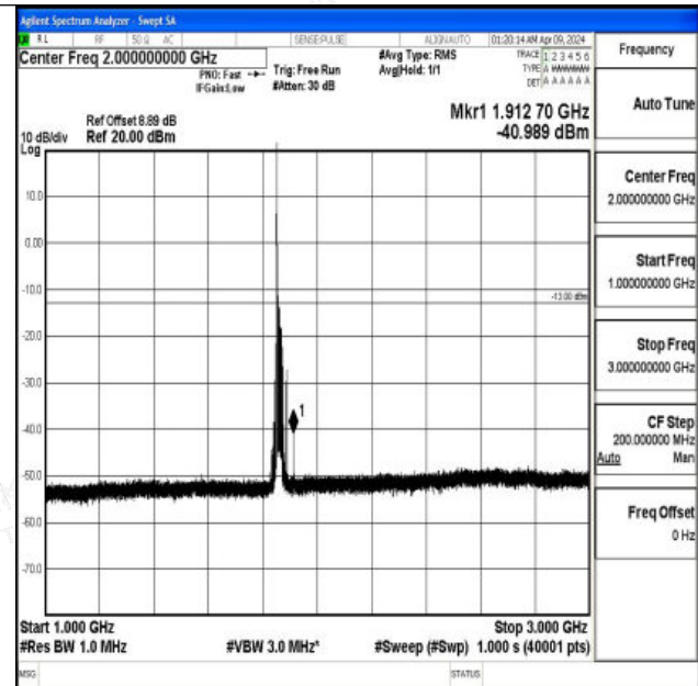
Band2_20MHz_QPSK_18700_1RB#0_1000~3000_1000~3000
