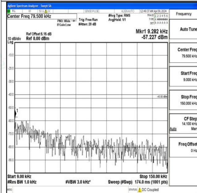
Band2_10MHz_QPSK_19150_1RB#0_0.009~0.15_0.009~ 0.15
