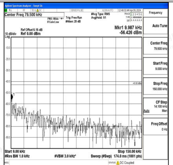
Band2_10MHz_16QAM_18650_1RB#0_0.009~0.15_0.009~0.15
