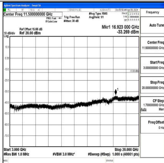
Band2_15MHz_16QAM_18900_1RB#0_3000~20000_3000 ~20000
