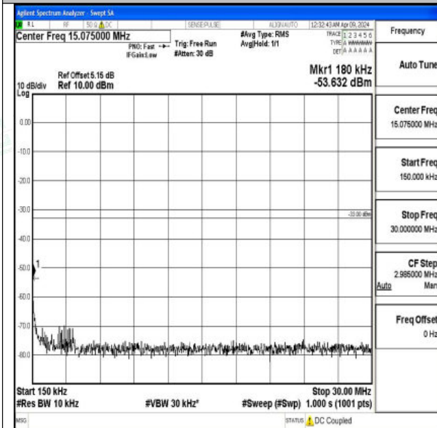
Band2_5MHz_16QAM_19175_1RB#0_0.15~30_0.15~30
