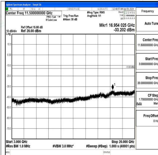
Band2_10MHz_QPSK_18900_1RB#0_3000~20000_3000~20000
