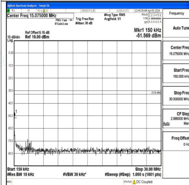
Band2_10MHz_16QAM_18900_1RB#0_0.15~30_0.15~30
