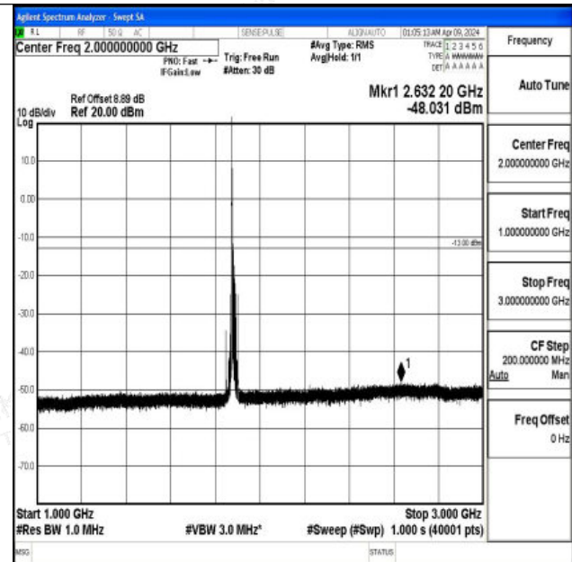
Band2_15MHz_QPSK_18900_1RB#0_1000~3000_1000~3000
