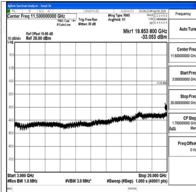
Band2_15MHz_QPSK_19125_1RB#0_3000~20000_3000~20000
