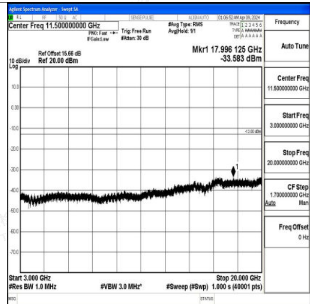
Band2_15MHz_16QAM_19125_1RB#0_3000~20000_3000 ~20000
