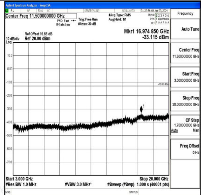
Band2_20MHz_16QAM_19100_1RB#0_3000~20000_3000~20000
