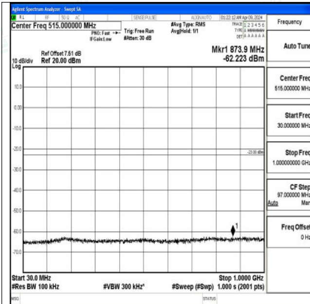
Band2_20MHz_QPSK_19100_1RB#0_30~1000_30~1000
