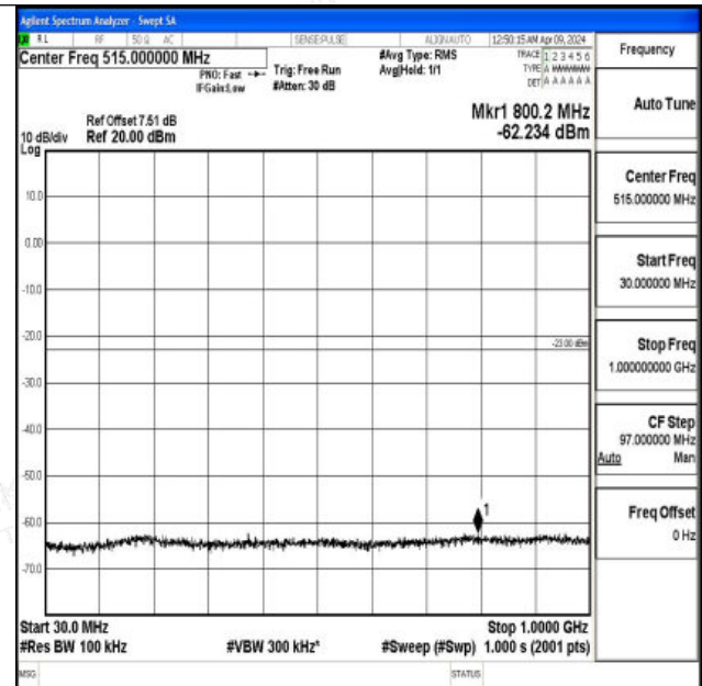
Band2_10MHz_16QAM_19150_1RB#0_30~1000_30~1000
