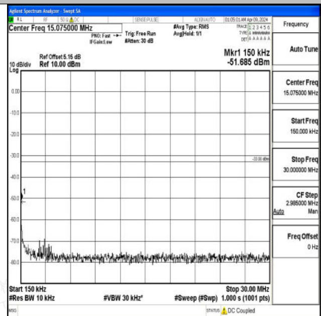
Band2_15MHz_QPSK_18900_1RB#0_0.15~30_0.15~30
