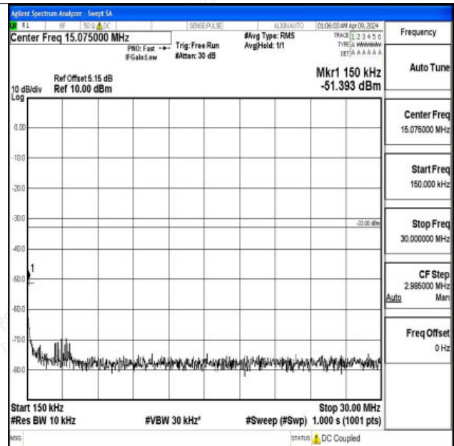
Band2_15MHz_QPSK_19125_1RB#0_0.15~30_0.15~30
