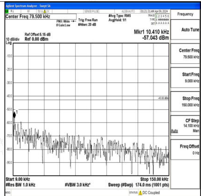
Band2_20MHz_16QAM_18900_1RB#0_0.009~0.15_0.009~0.15
