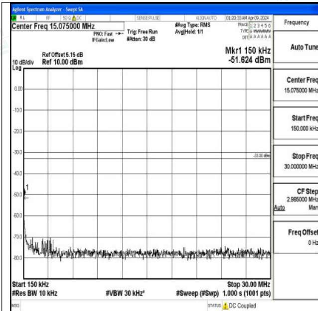
Band2_20MHz_16QAM_18700_1RB#0_0.15~30_0.15~30
