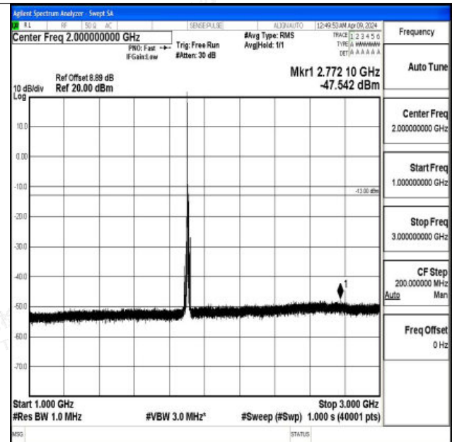
Band2_10MHz_QPSK_19150_1RB#0_1000~3000_1000~3000
