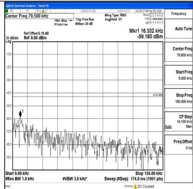
Band2_15MHz_16QAM_18900_1RB#0_0.009~0.15_0.009~0.15
