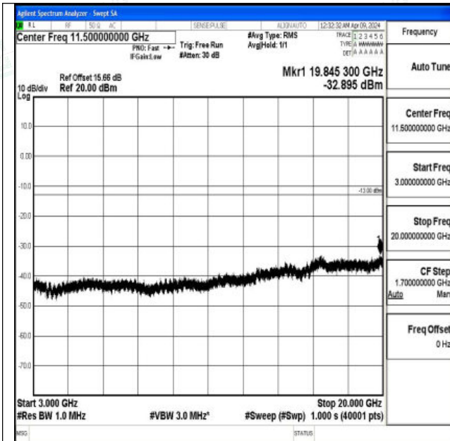
Band2_5MHz_QPSK_19175_1RB#0_3000~20000_3000~20000
