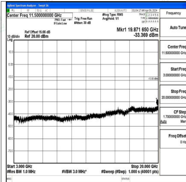
Band2_15MHz_QPSK_18675_1RB#0_3000~20000_3000~20000
