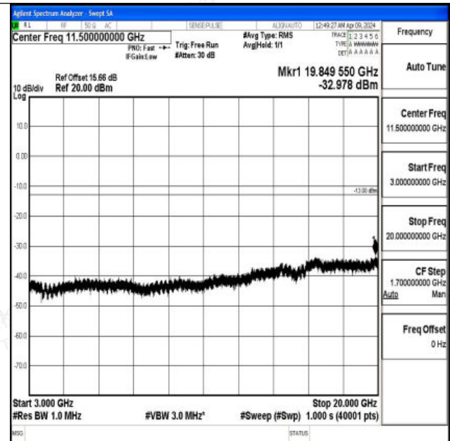
Band2_10MHz_16QAM_18900_1RB#0_3000~20000_3000 ~20000
