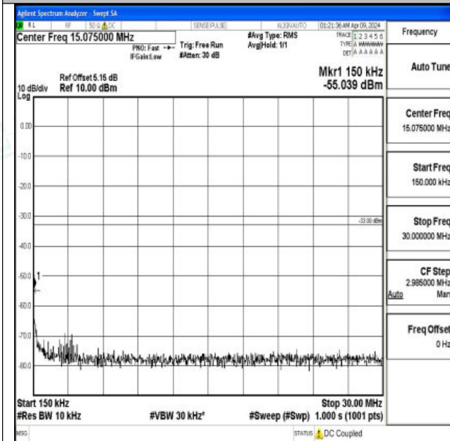
Band2_20MHz_16QAM_18900_1RB#0_0.15~30_0.15~30
