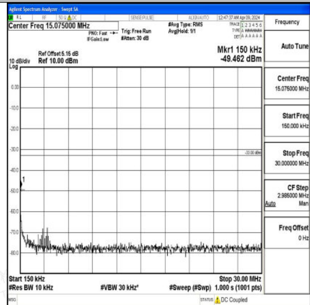
Band2_10MHz_QPSK_18650_1RB#0_0.15~30_0.15~30
