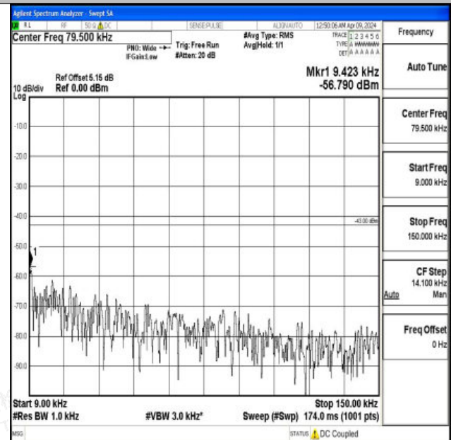
Band2_10MHz_16QAM_19150_1RB#0_0.009~0.15_0.009~0.15
