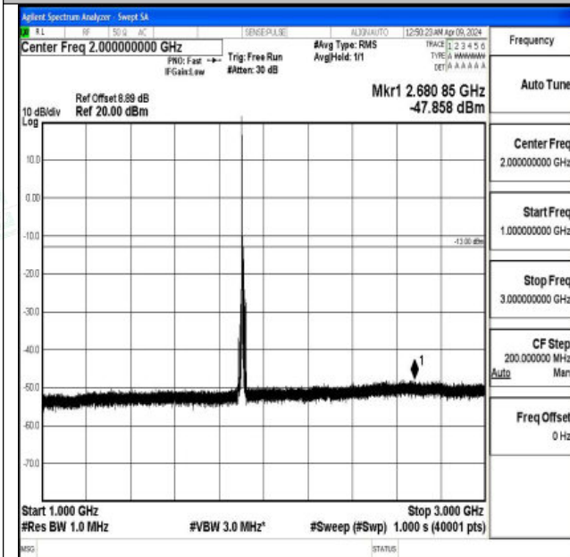
Band2_10MHz_16QAM_19150_1RB#0_1000~3000_1000~3000
