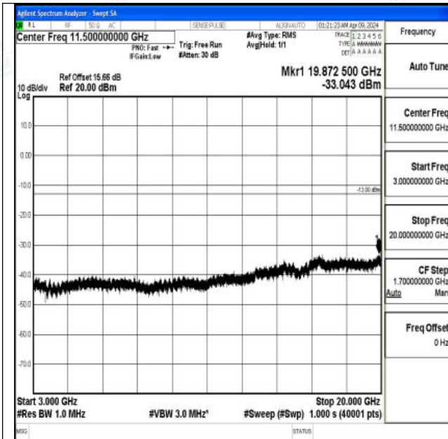
Band2_20MHz_QPSK_18900_1RB#0_3000~20000_3000~20000
