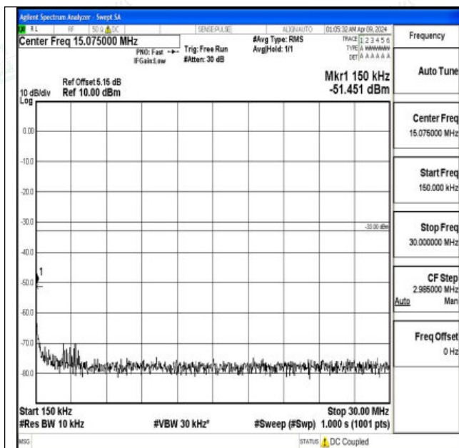
Band2_15MHz_16QAM_18900_1RB#0_0.15~30_0.15~30
