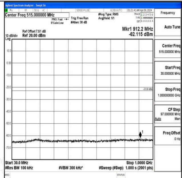
Band2_20MHz_16QAM_18900_1RB#0_30~1000_30~1000
