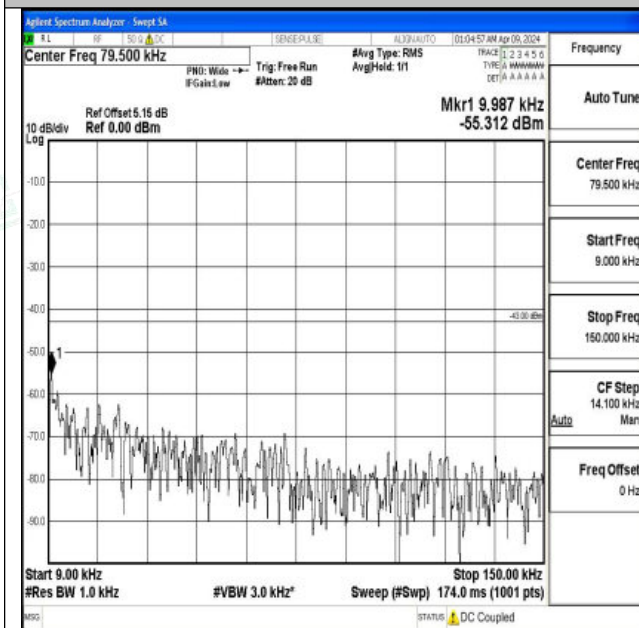
Band2_15MHz_QPSK_18900_1RB#0_0.009~0.15_0.009~ 0.15
