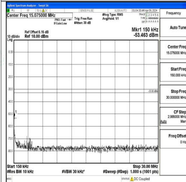
Band2_15MHz_16QAM_18675_1RB#0_0.15~30_0.15~30
