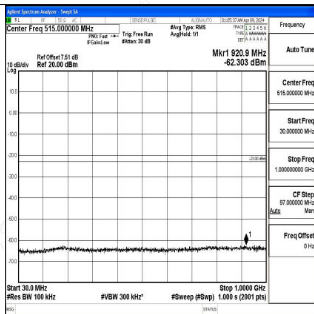
Band2_15MHz_16QAM_18900_1RB#0_30~1000_30~1000
