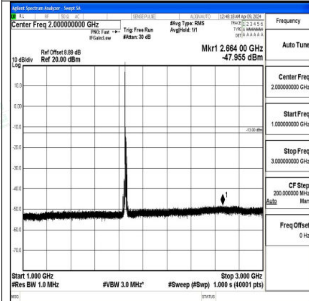
Band2_10MHz_16QAM_18650_1RB#0_1000~3000_1000 ~3000
