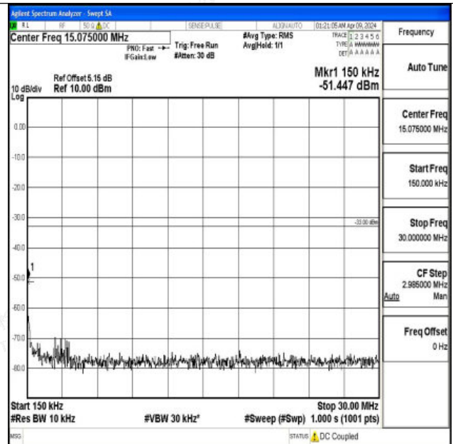
Band2_20MHz_QPSK_18900_1RB#0_0.15~30_0.15~30
