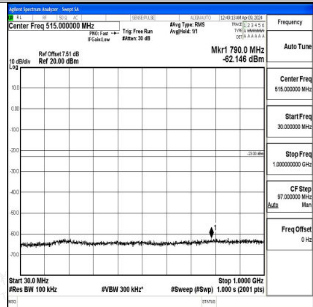
Band2_10MHz_16QAM_18900_1RB#0_30~1000_30~1000
