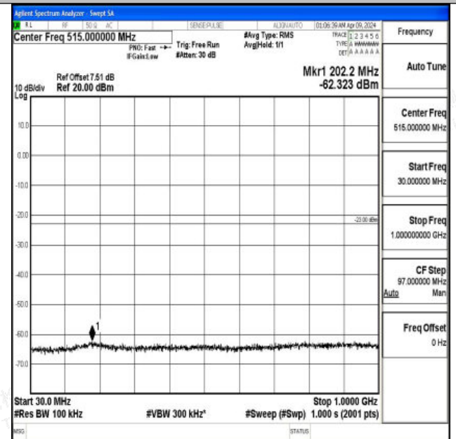
Band2_15MHz_16QAM_19125_1RB#0_30~1000_30~1000
