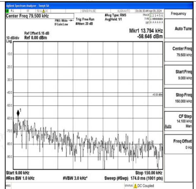
Band2_15MHz_16QAM_19125_1RB#0_0.009~0.15_0.009~0.15
