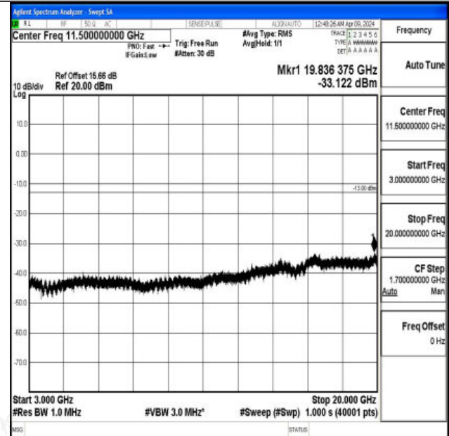
Band2_10MHz_16QAM_18650_1RB#0_3000~20000_3000 ~20000
