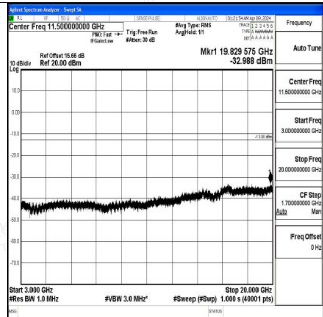
Band2_20MHz_16QAM_18900_1RB#0_3000~20000_3000 ~20000
