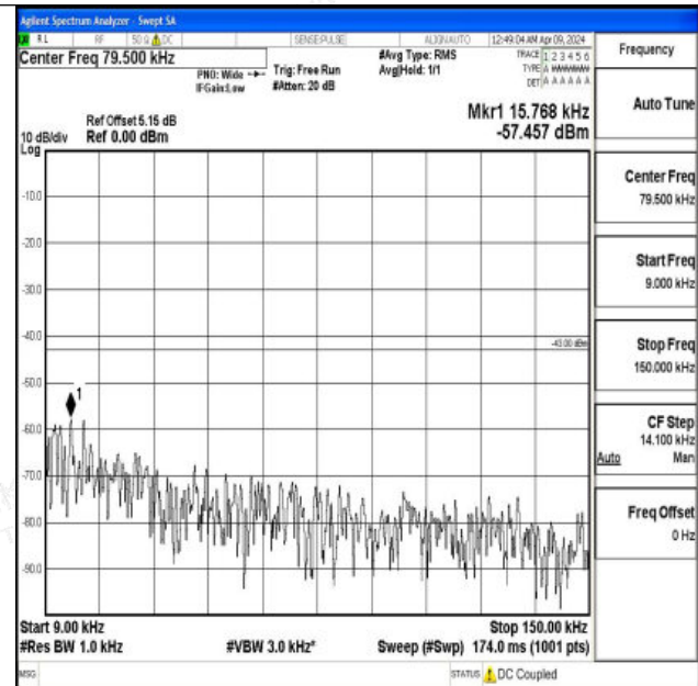
Band2_10MHz_16QAM_18900_1RB#0_0.009~0.15_0.009~0.15
