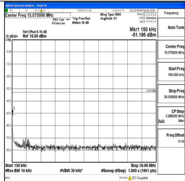
Band2_20MHz_QPSK_19100_1RB#0_0.15~30_0.15~30
