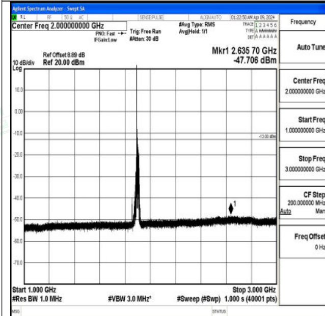
Band2_20MHz_16QAM_19100_1RB#0_1000~3000_1000~3000
