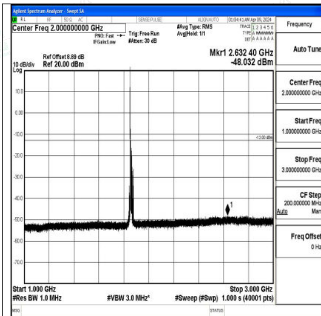
Band2_15MHz_16QAM_18675_1RB#0_1000~3000_1000 ~3000
