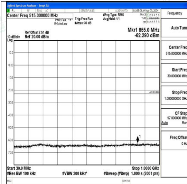
Band2_15MHz_QPSK_18900_1RB#0_30~1000_30~1000
