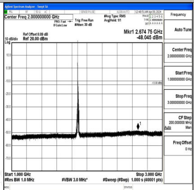
Band2_10MHz_QPSK_18900_1RB#0_1000~3000_1000~3000
