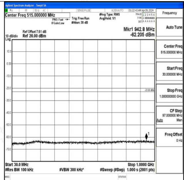
Band2_20MHz_16QAM_19100_1RB#0_30~1000_30~1000
