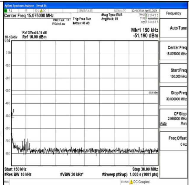
Band2_10MHz_QPSK_18900_1RB#0_0.15~30_0.15~30
