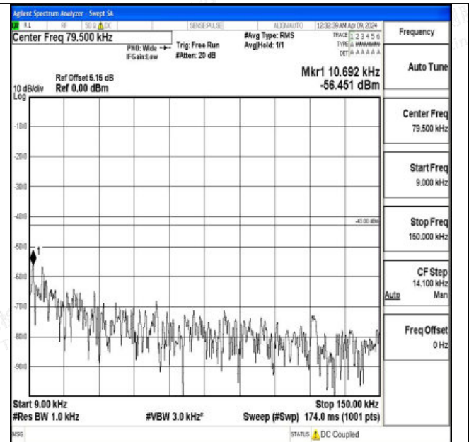
Band2_5MHz_16QAM_19175_1RB#0_0.009~0.15_0.009~0.15
