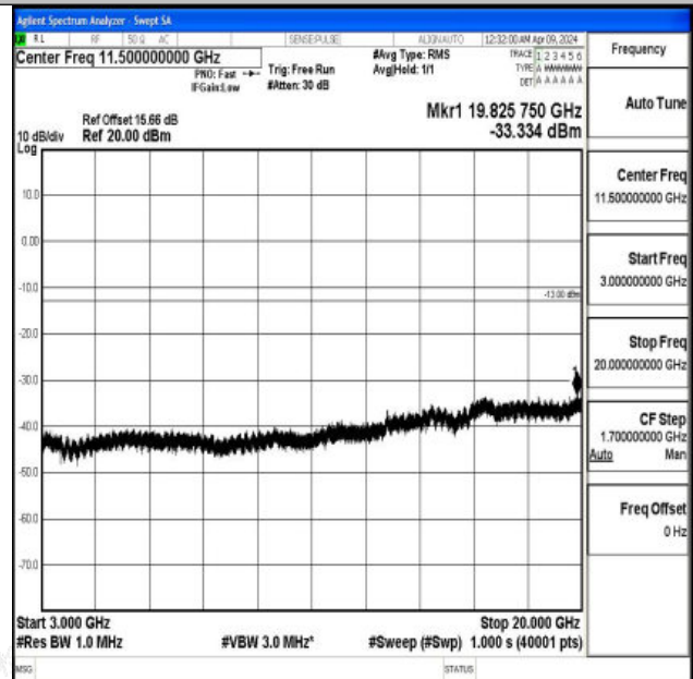
Band2_5MHz_16QAM_18900_1RB#0_3000~20000_3000~20000
