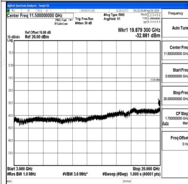
Band2_20MHz_QPSK_19100_1RB#0_3000~20000_3000~20000
