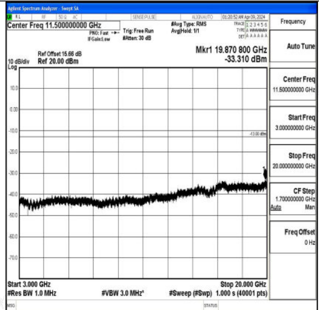
Band2_20MHz_16QAM_18700_1RB#0_3000~20000_3000 ~20000
