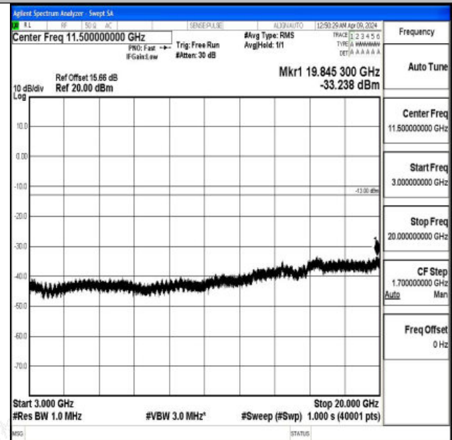
Band2_10MHz_16QAM_19150_1RB#0_3000~20000_3000~20000
