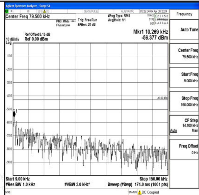
Band2_20MHz_16QAM_19100_1RB#0_0.009~0.15_0.009~0.15
