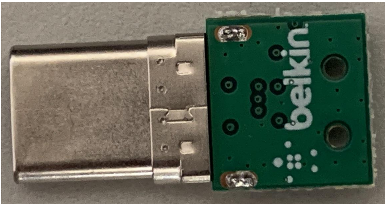
Bottom photo of PCB
