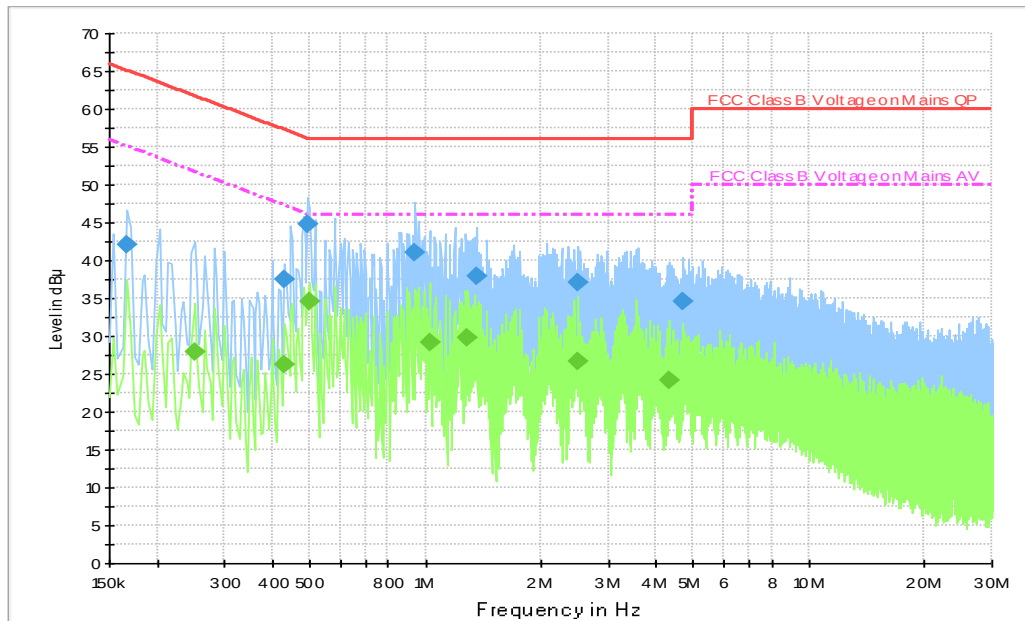
Fig.B.11.1 AC Powerline Conducted Emission- 802.11b, charger TN-050120U8
