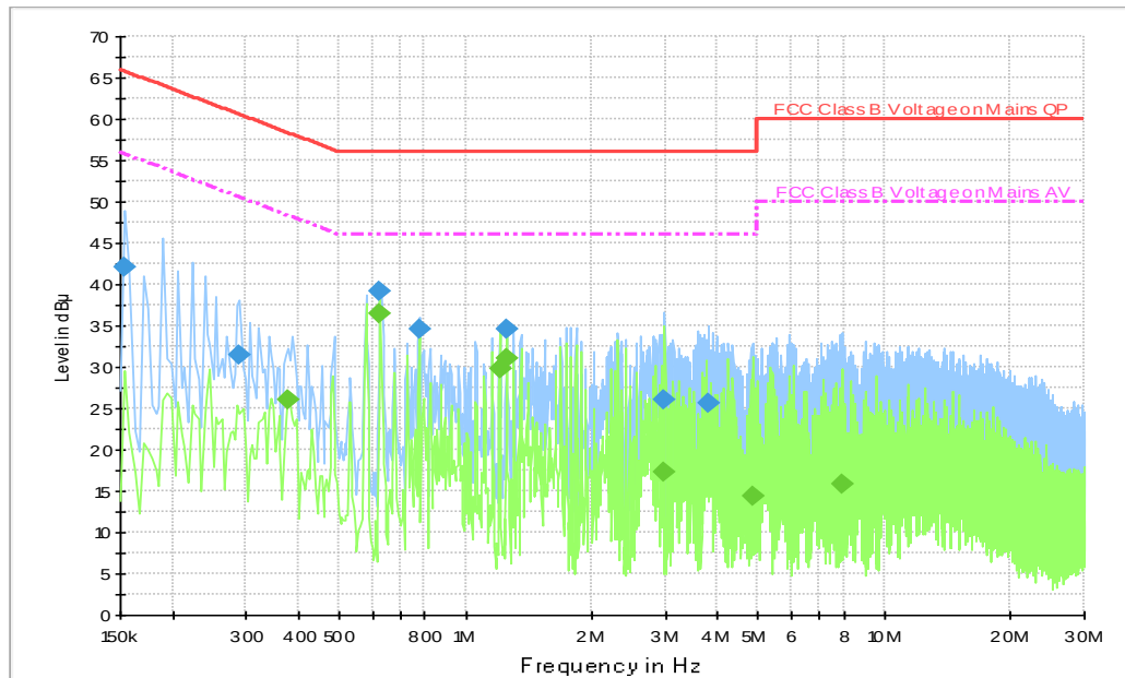
Fig.A.7.1 AC Powerline Conducted Emission- 802.11b, charger TN-050120U9
