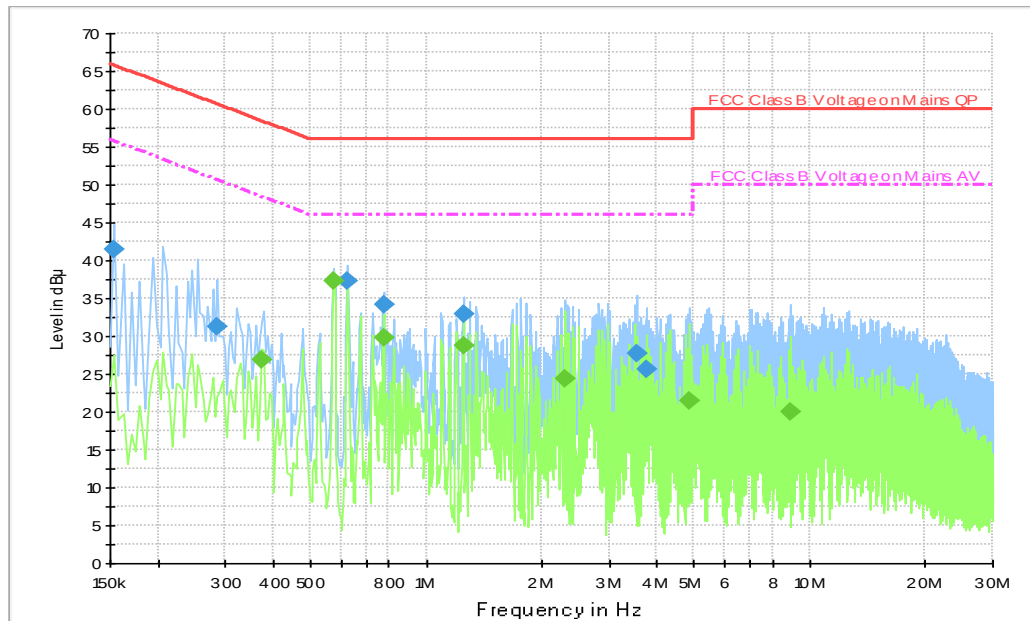
Fig.A.7.2 AC Powerline Conducted Emission-Idle, charger TN-050120U9
