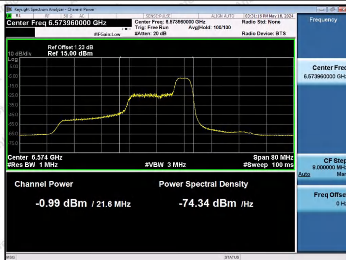
11AX40SISO-Ant1-6565-52Tone-RU44-PASS
