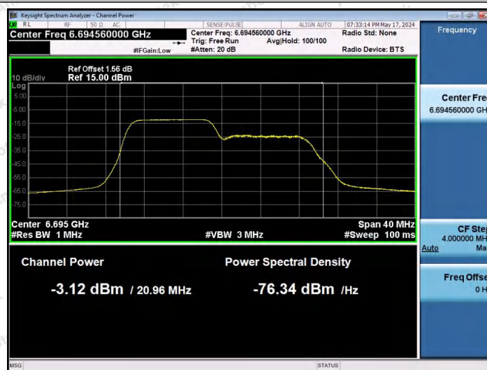
11AX20SISO-Ant1-6695-106Tone-RU53-PASS
