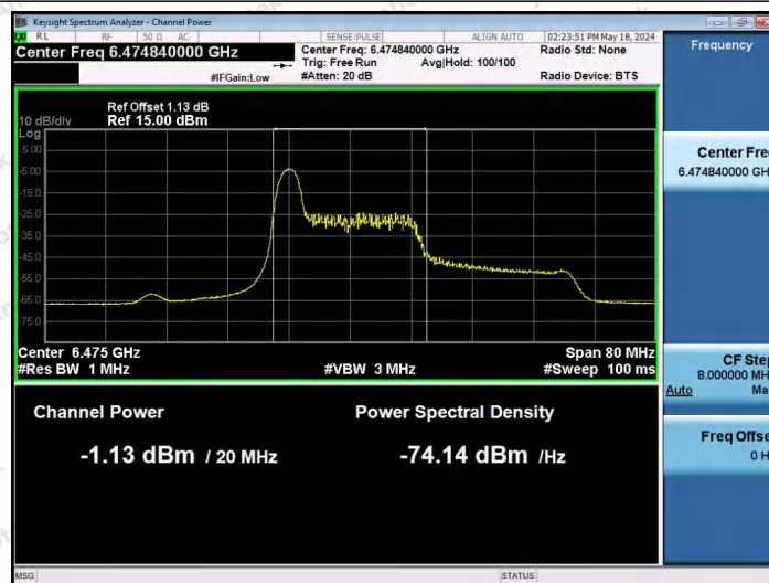
11AX40SISO-Ant1-6485-26Tone-RU0-PASS
