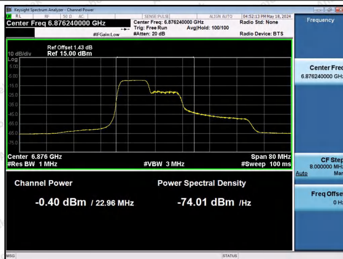
11AX40SISO-Ant1-6885-106Tone-RU53-PASS
