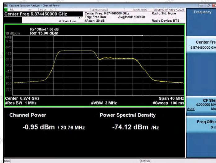
11AX20SISO-Ant1-6875-106Tone-RU53-PASS
