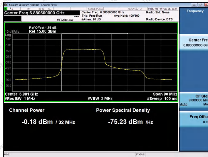
11AX40SISO-Ant1-6885-242Tone-RU61-PASS
