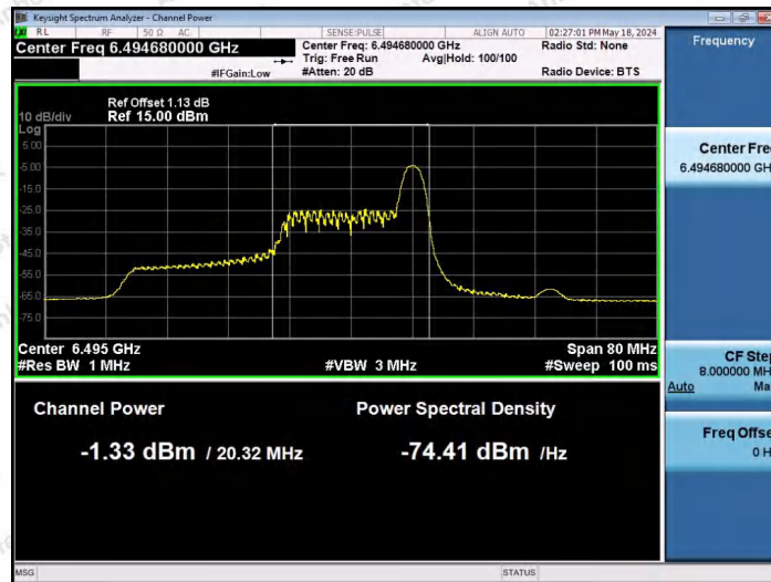
11AX40SISO-Ant1-6485-26Tone-RU17-PASS
