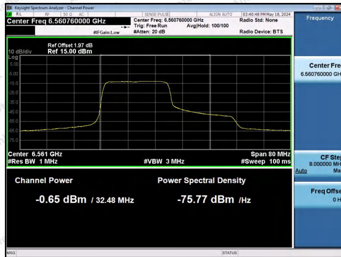
11AX40SISO-Ant1-6565-242Tone-RU61-PASS
