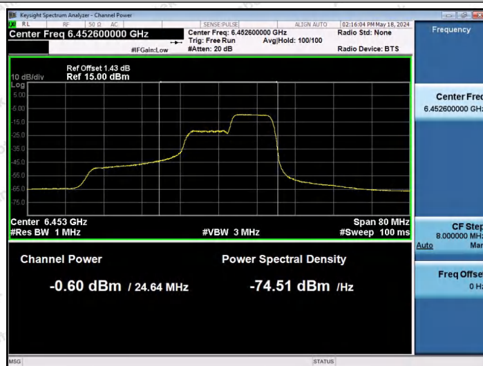
11AX40SISO-Ant1-6445-106Tone-RU56-PASS
