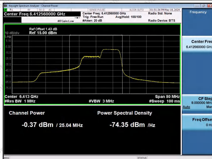
11AX40SISO-Ant1-6405-106Tone-RU56-PASS
