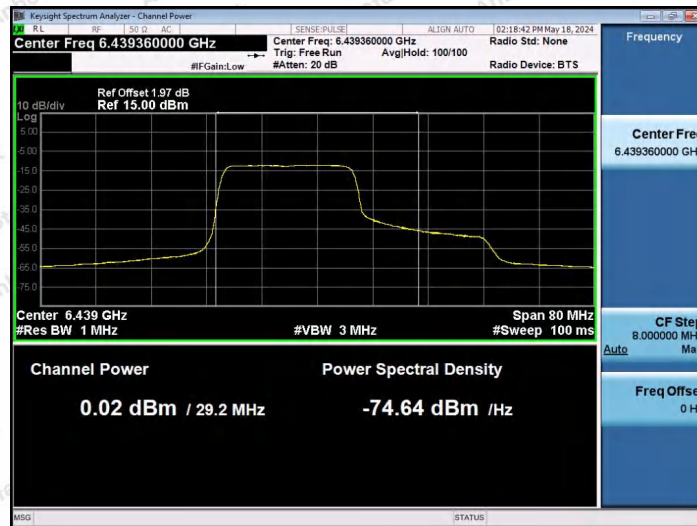
11AX40SISO-Ant1-6445-242Tone-RU61-PASS
