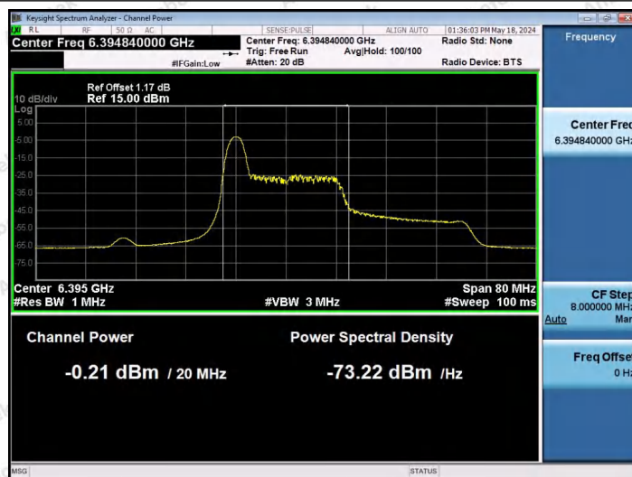
11AX40SISO-Ant1-6405-26Tone-RU0-PASS
