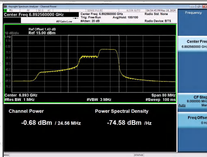
11AX40SISO-Ant1-6885-106Tone-RU56-PASS
