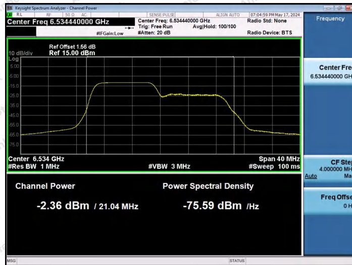
11AX20SISO-Ant1-6535-106Tone-RU53-PASS
