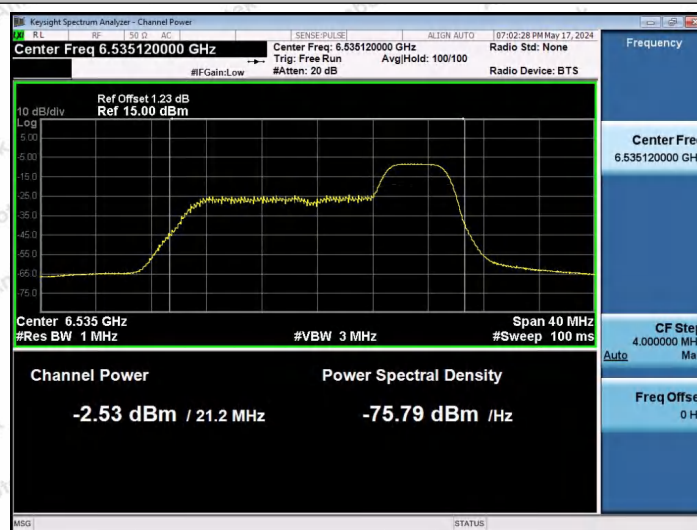
11AX20SISO-Ant1-6535-52Tone-RU40-PASS
