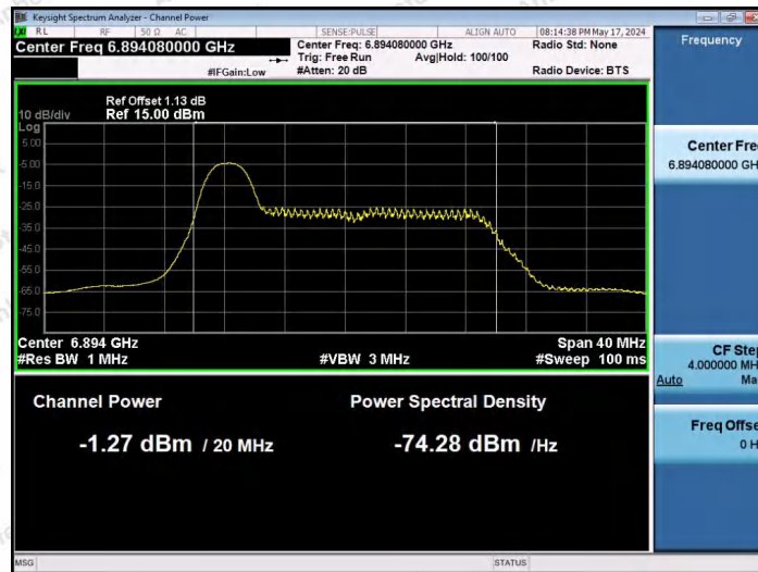
11AX20SISO-Ant1-6895-26Tone-RU0-PASS
