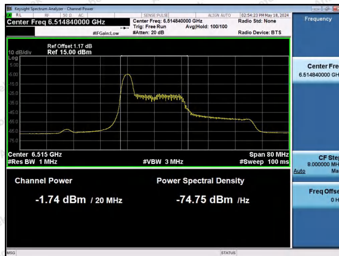
11AX40SISO-Ant1-6525-26Tone-RU0-PASS
