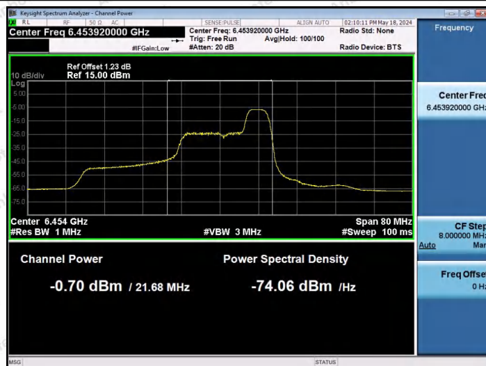
11AX40SISO-Ant1-6445-52Tone-RU44-PASS
