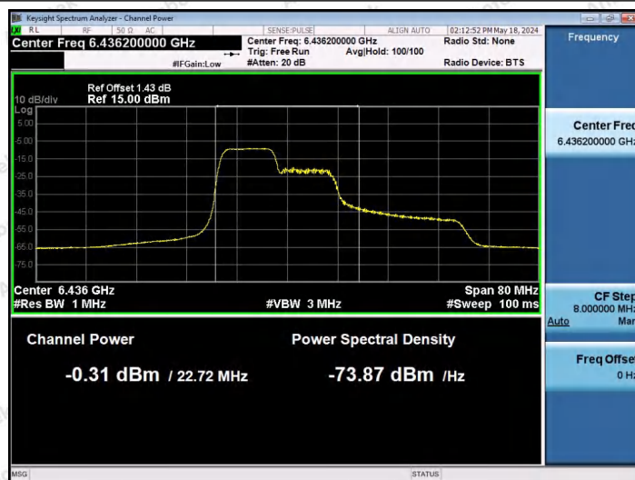
11AX40SISO-Ant1-6445-106Tone-RU53-PASS
