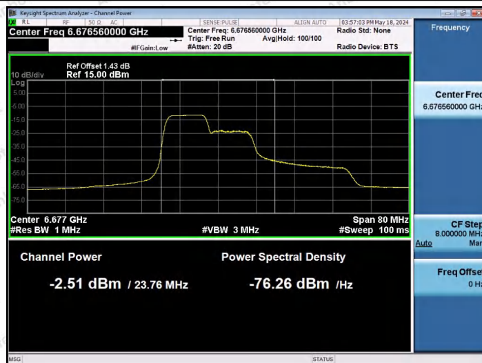
11AX40SISO-Ant1-6685-106Tone-RU53-PASS
