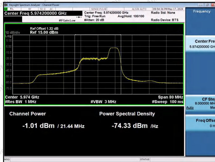
11AX40SISO-Ant1-5965-52Tone-RU44-PASS
