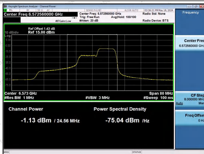
11AX40SISO-Ant1-6565-106Tone-RU56-PASS
