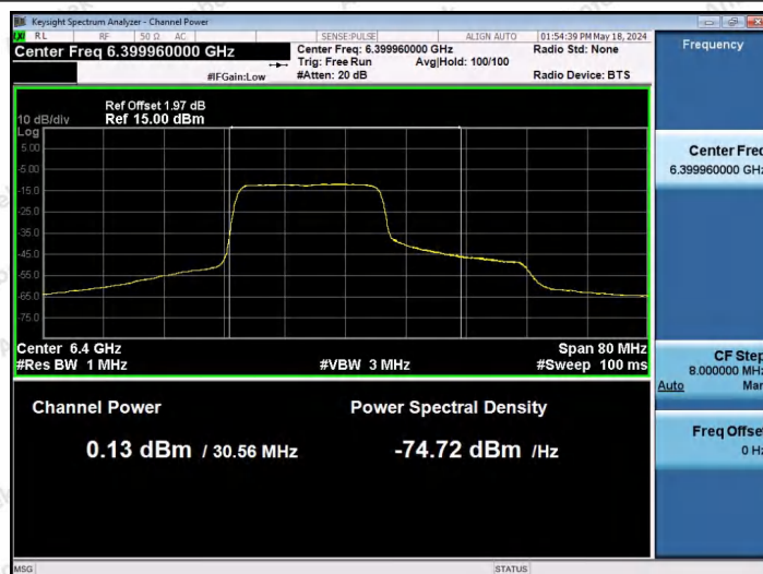
11AX40SISO-Ant1-6405-242Tone-RU61-PASS
