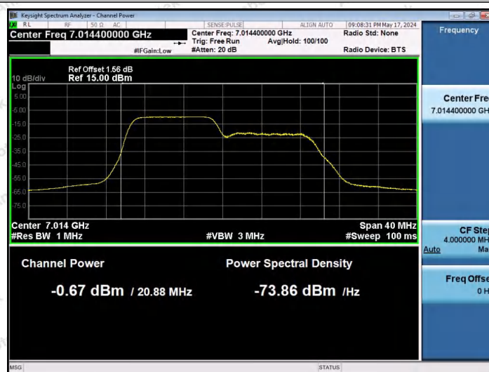
11AX20SISO-Ant1-7015-106Tone-RU53-PASS
