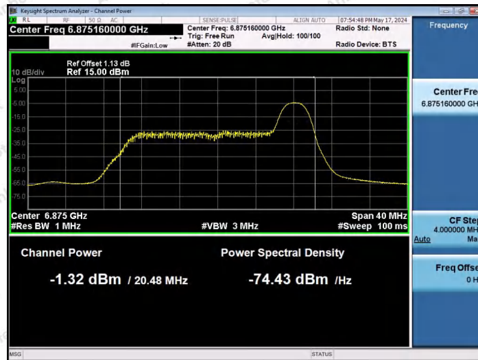
11AX20SISO-Ant1-6875-26Tone-RU8-PASS
