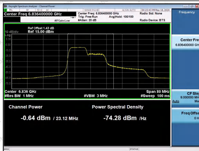
11AX40SISO-Ant1-6845-106Tone-RU53-PASS
