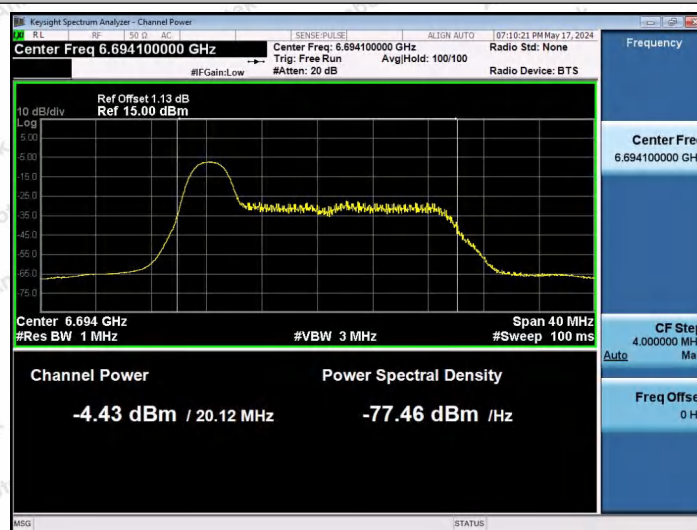
11AX20SISO-Ant1-6695-26Tone-RU0-PASS
