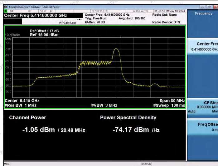
11AX40SISO-Ant1-6405-26Tone-RU17-PASS
