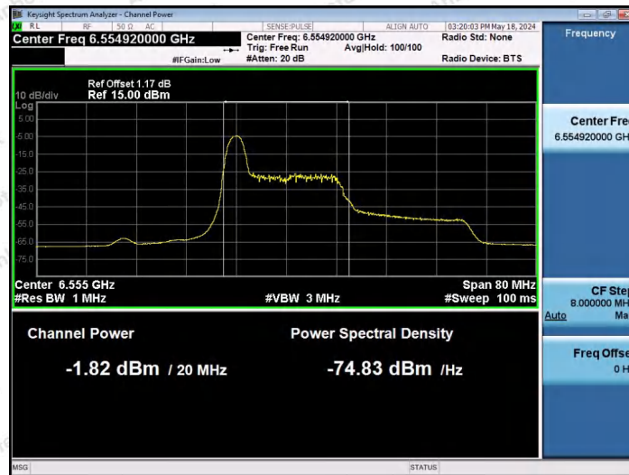
11AX40SISO-Ant1-6565-26Tone-RU0-PASS
