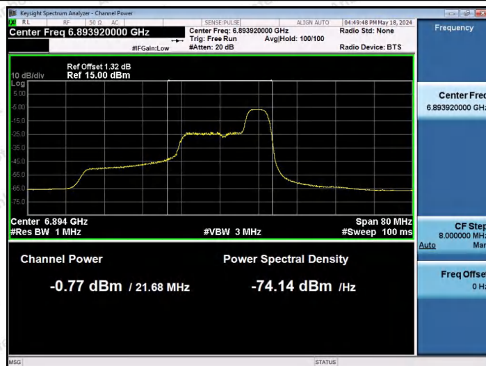
11AX40SISO-Ant1-6885-52Tone-RU44-PASS
