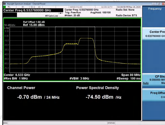
11AX40SISO-Ant1-6525-106Tone-RU56-PASS
