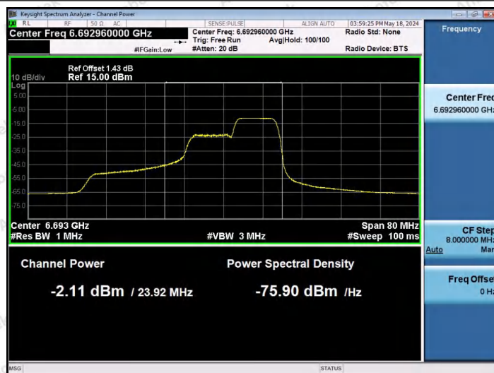
11AX40SISO-Ant1-6685-106Tone-RU56-PASS
