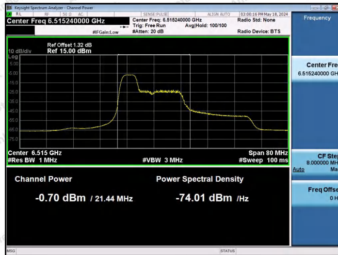
11AX40SISO-Ant1-6525-52Tone-RU37-PASS
