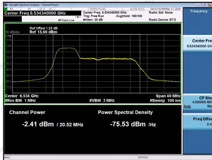
11AX20SISO-Ant1-6535-52Tone-RU37-PASS
