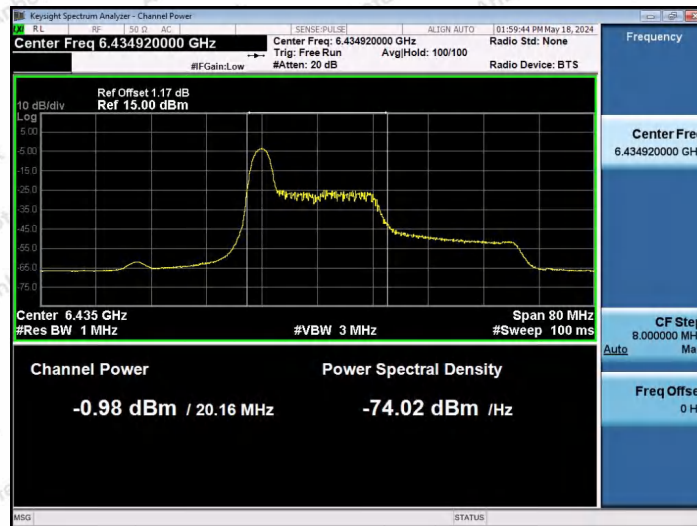
11AX40SISO-Ant1-6445-26Tone-RU0-PASS
