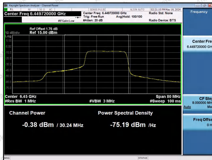
11AX40SISO-Ant1-6445-242Tone-RU62-PASS
