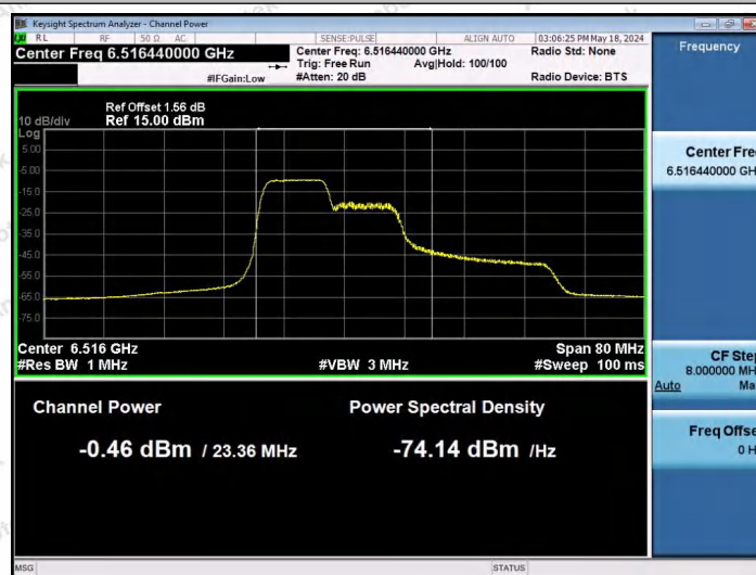
11AX40SISO-Ant1-6525-106Tone-RU53-PASS
