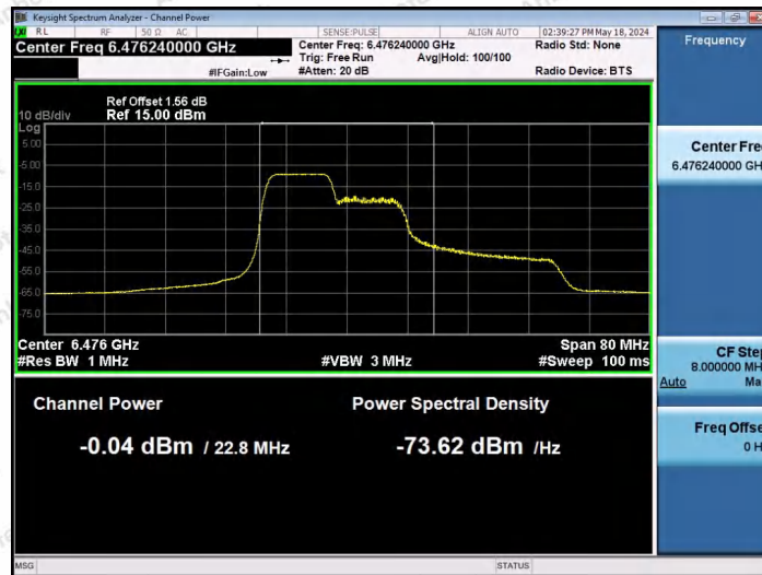
11AX40SISO-Ant1-6485-106Tone-RU53-PASS
