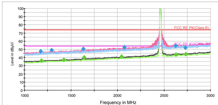
RE 1G-3GHz PK+AV
