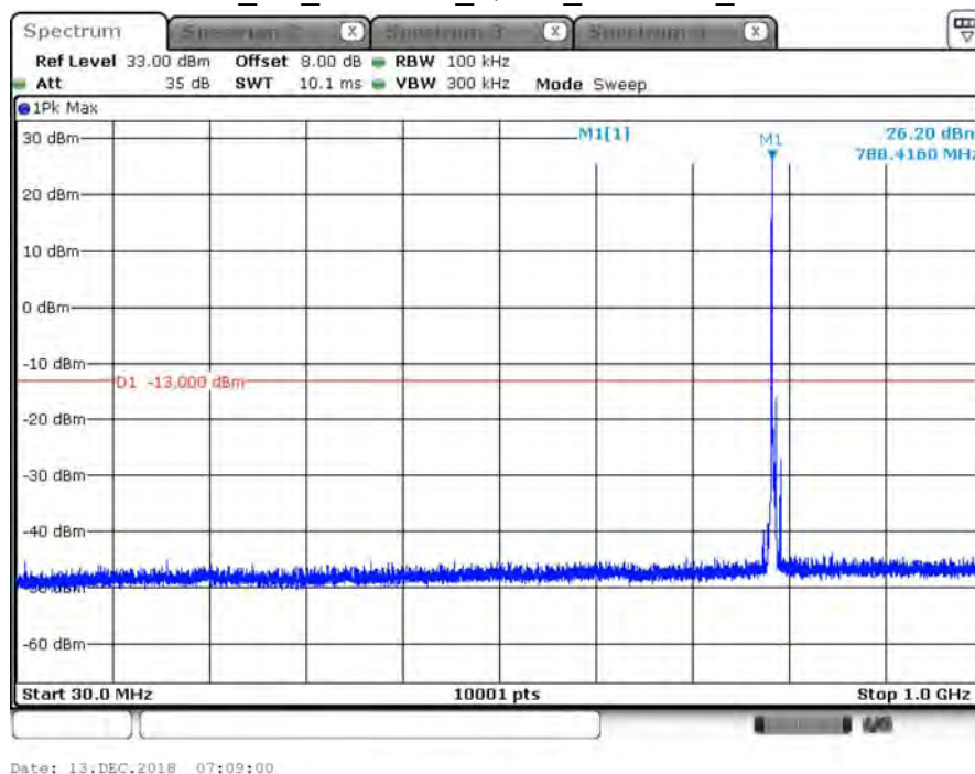
B14_5M_CH23305_QPSK_under 1G_1RB0
