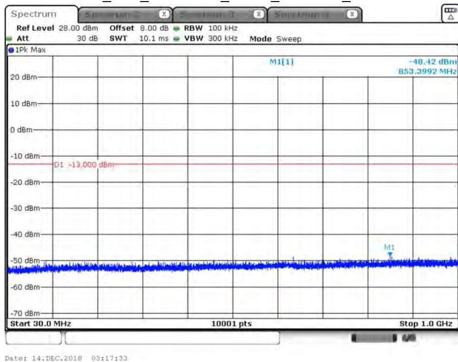
B66_20M_CH132322_QPSK_under 1G_1RB0
