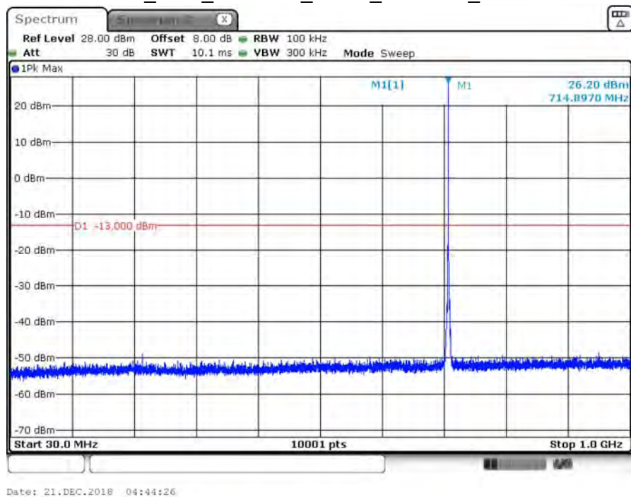
B12_1.4M_CH23173_QPSK_under 1G_1RB0
