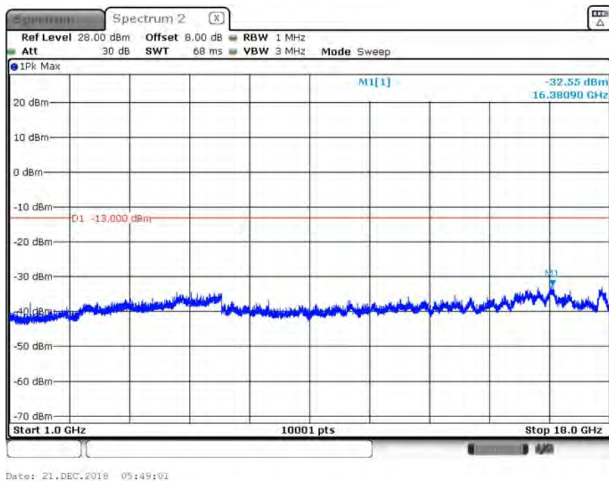
B14_5M_CH23355_QPSK_Above 1G_1RB0
