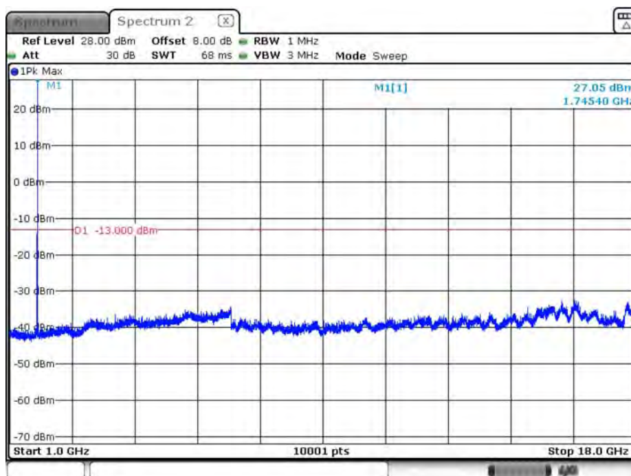
B66_1.4M_CH132322_16QAM_above 1G_1RB0
