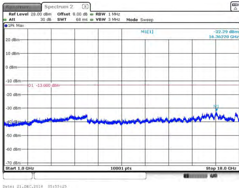
B14_10M_CH23330_16QAM_Above 1G_1RB0
