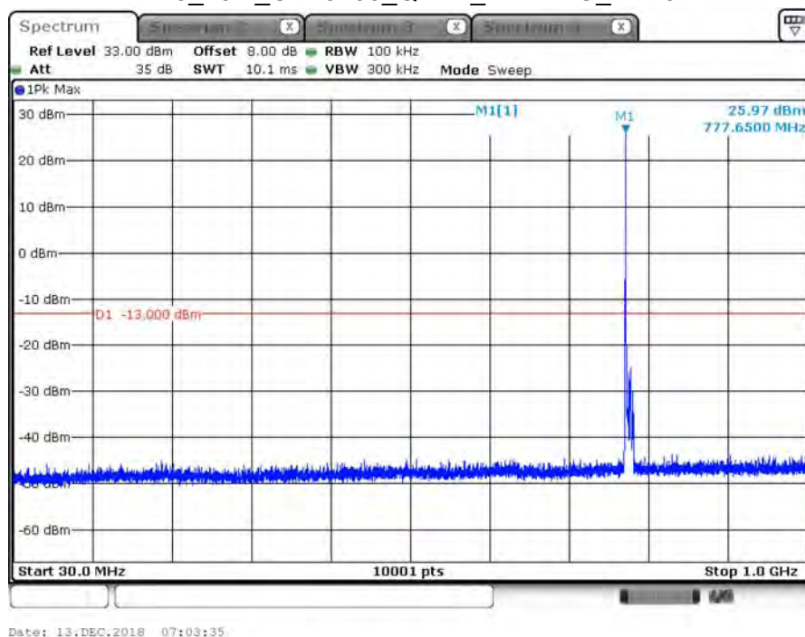
B13_10M_CH23230_QPSK_under 1G_1RB0
