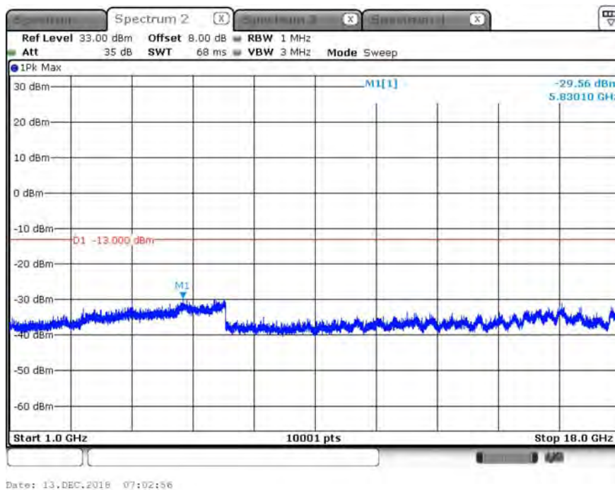
B13_10M_CH23230_QPSK_above 1G_1RB0
