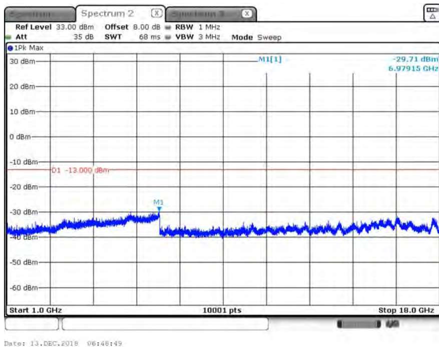
B17_5M_CH23790_QPSK_above 1G_1RB0
