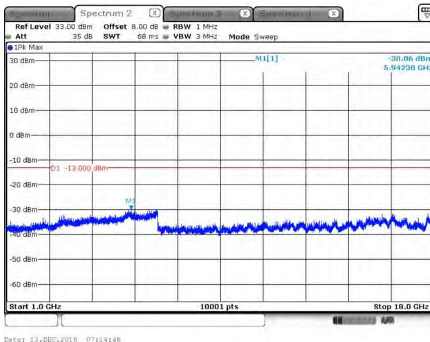
B14_10M_CH23330_QPSK_Above 1G_1RB0
