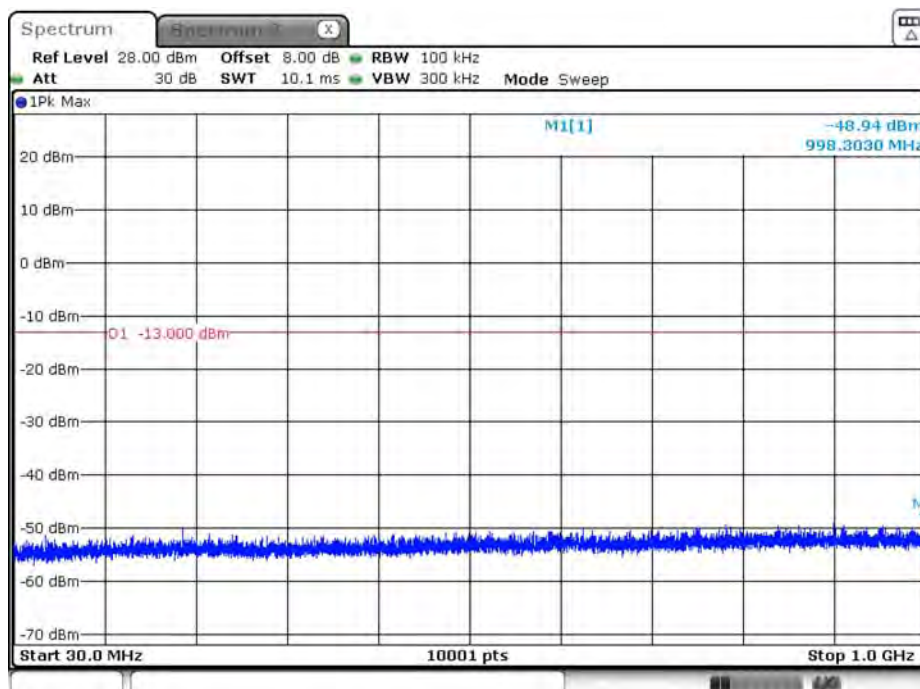
B66_1.4M_CH131979_16QAM_under 1G_1RB0
