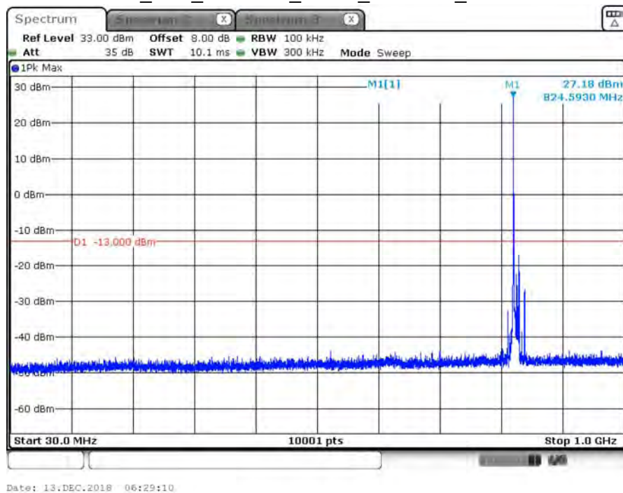
B5_10M_CH20450_QPSK_under 1G_1RB0
