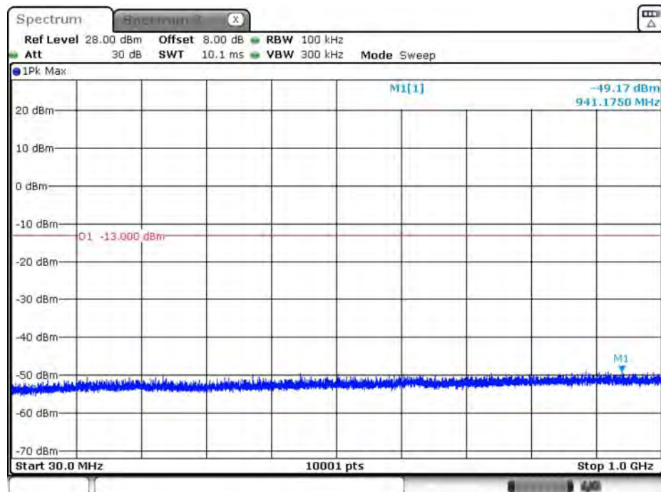
B66_1.4M_CH132665_16QAM_under 1G_1RB0
