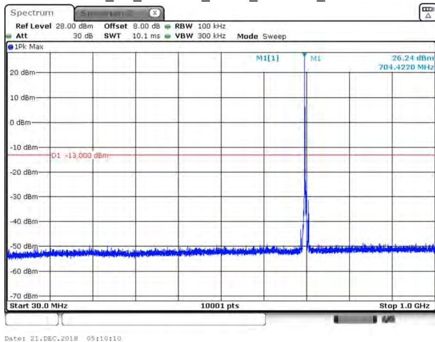
B17_5M_CH23755_QPSK_under 1G_1RB0
