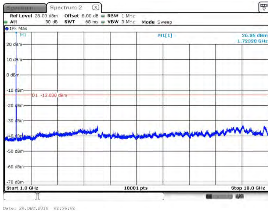
B4_20M_CH20175_QPSK_above 1G_1RB0
