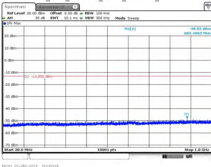
B4_1.4M_CH19957_QPSK_under 1G_1RB0
