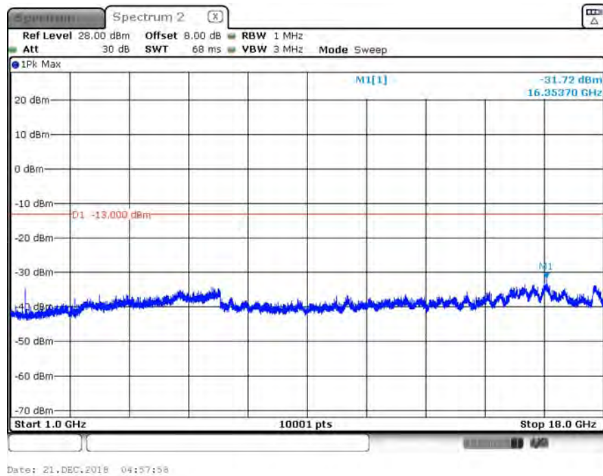
B12_10M_CH23130_QPSK_above 1G_1RB0
