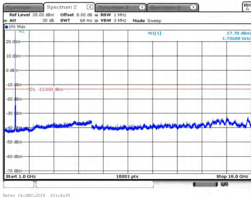
B66_20M_CH132322_QPSK_above 1G_1RB0
