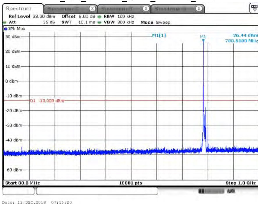
B14_10M_CH23330_QPSK_under 1G_1RB0
