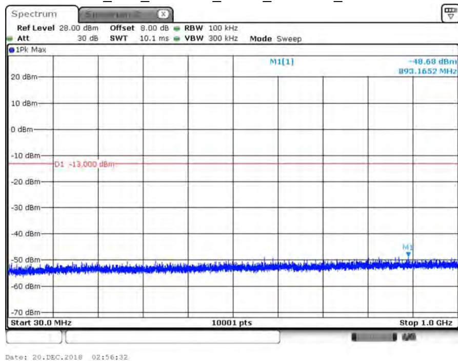
B4_20M_CH20175_QPSK_under 1G_1RB0
