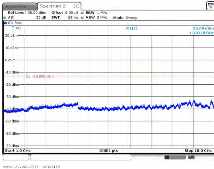
B4_1.4M_CH20175_16QAM_above 1G_1RB0
