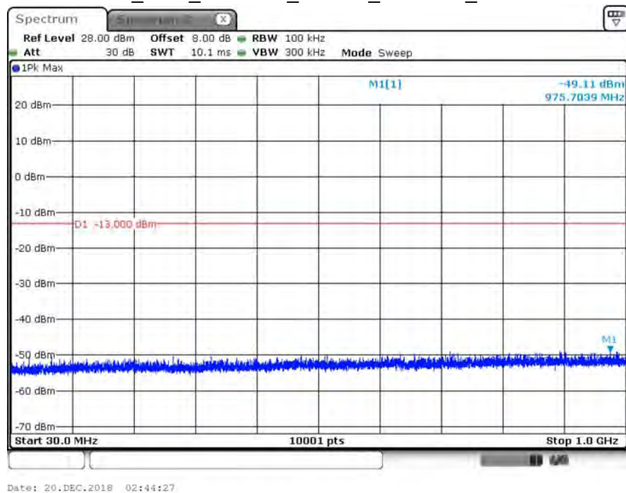
B4_1.4M_CH20175_16QAM_under 1G_1RB0
