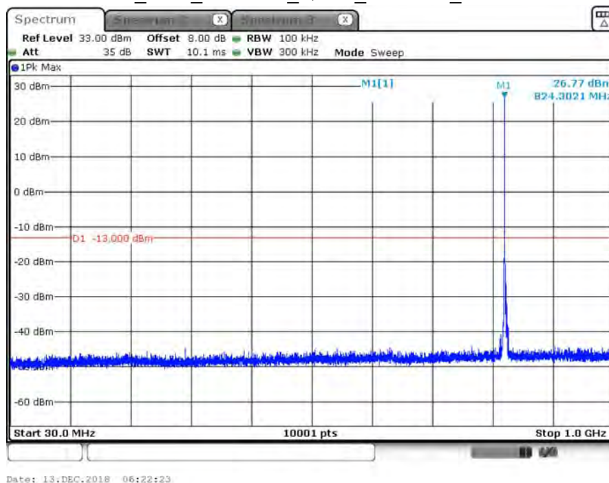
B5_1.4M_CH20407_QPSK_under 1G_1RB0
