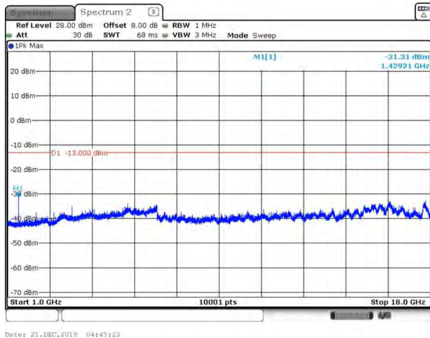
B12_1.4M_CH23173_QPSK_above 1G_1RB0
