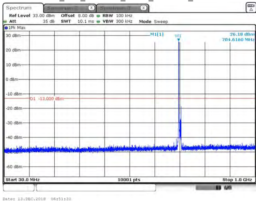
B17_10M_CH23780_QPSK_under 1G_1RB0
