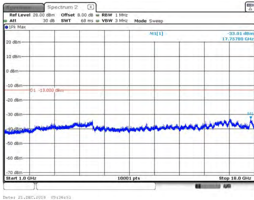
B13_5M_CH23230_QPSK_above 1G_1RB0
