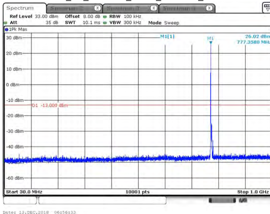
B13_5M_CH23205_QPSK_under 1G_1RB0
