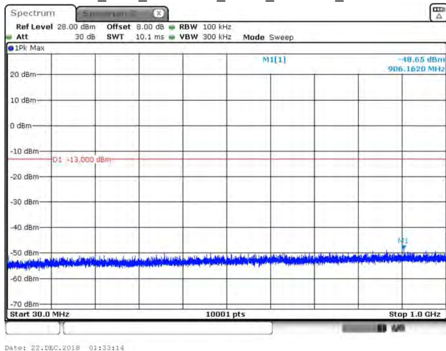
B66_1.4M_CH132322_QPSK_under 1G_1RB0
