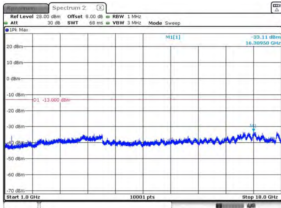
B17_10M_CH23790_16QAM_above 1G_1RB0
