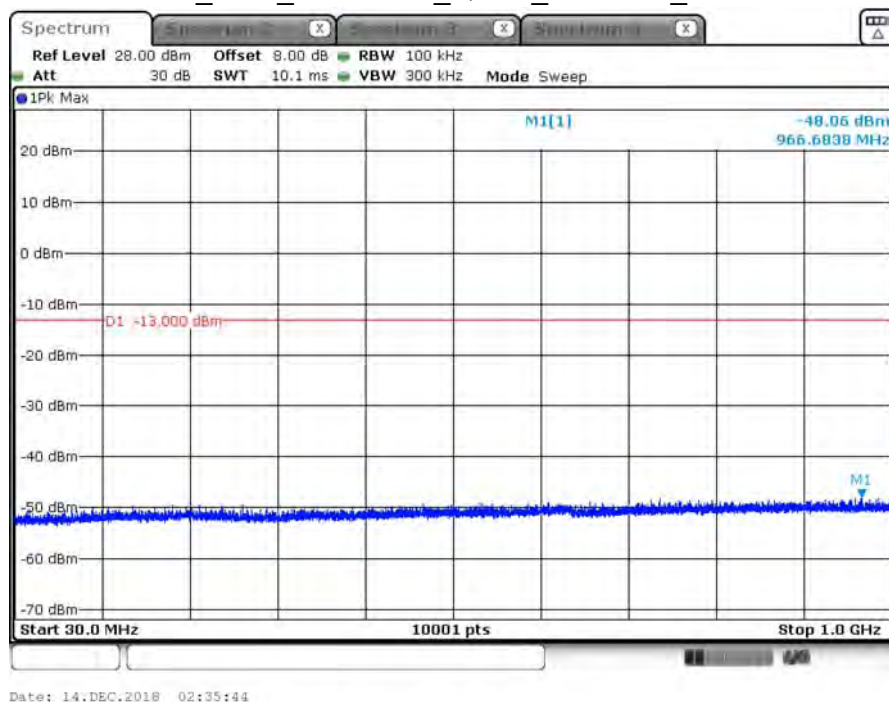
B66_1.4M_CH131979_QPSK_under 1G_1RB0
