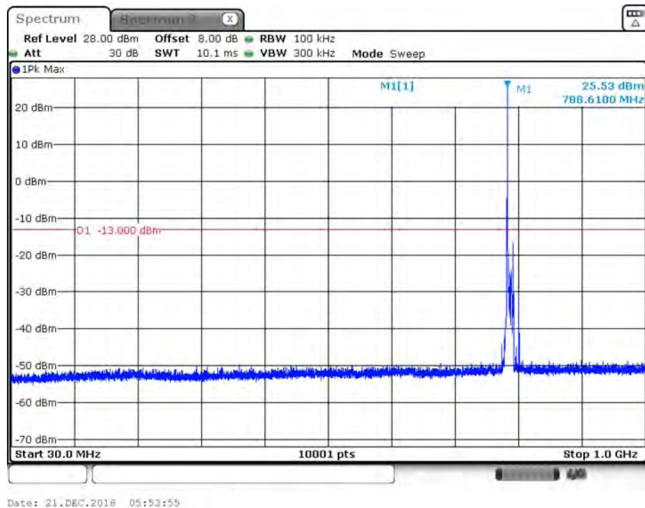
B14_10M_CH23330_16QAM_under 1G_1RB0
