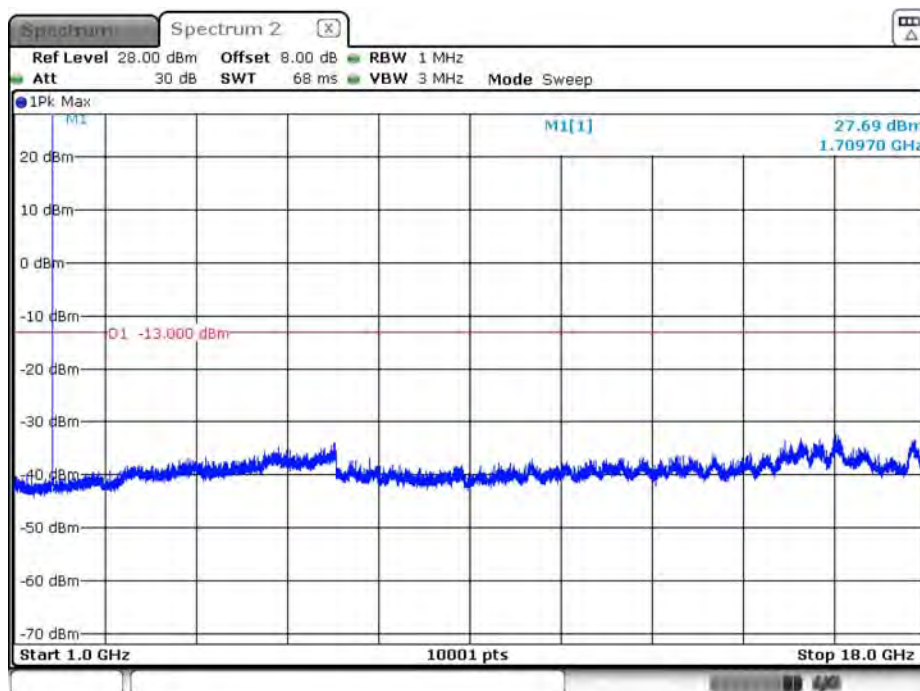
B66_1.4M_CH131979_16QAM_above 1G_1RB0
