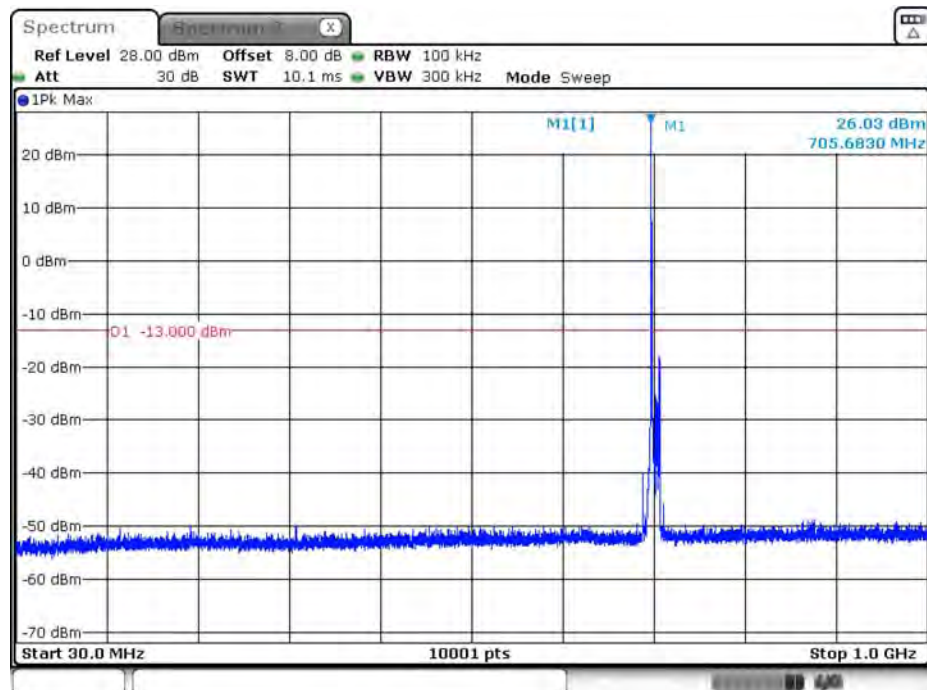
B17_10M_CH23790_16QAM_under 1G_1RB0
