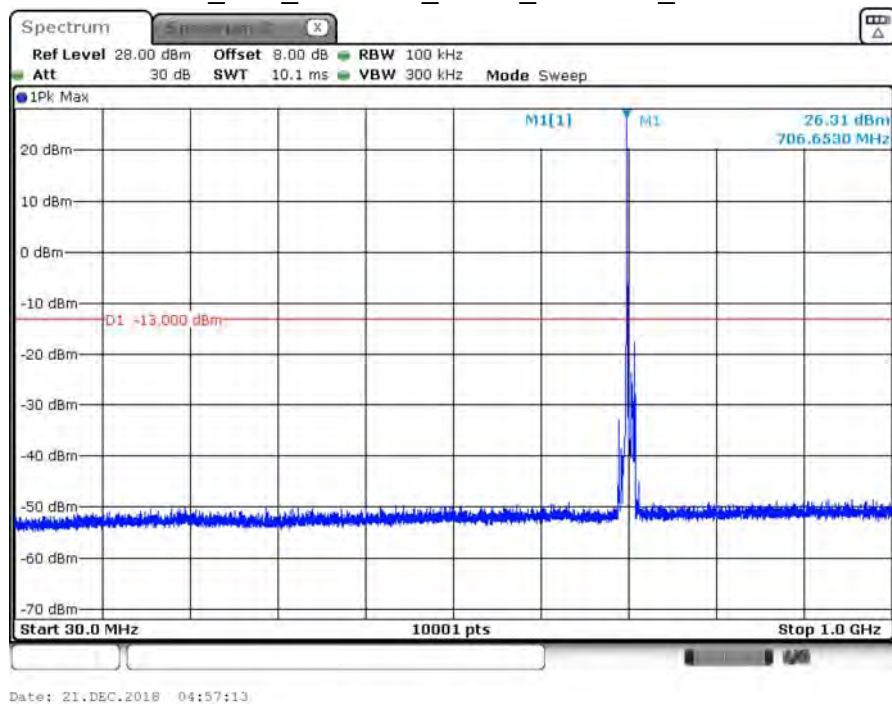
B12_10M_CH23130_QPSK_under 1G_1RB0
