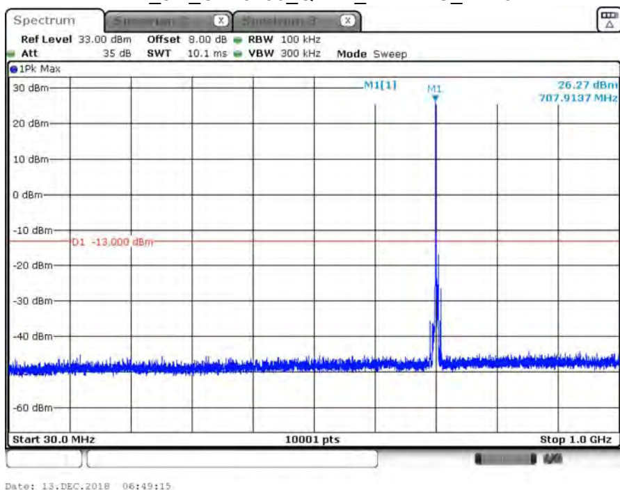
B17_5M_CH23790_QPSK_under 1G_1RB0
