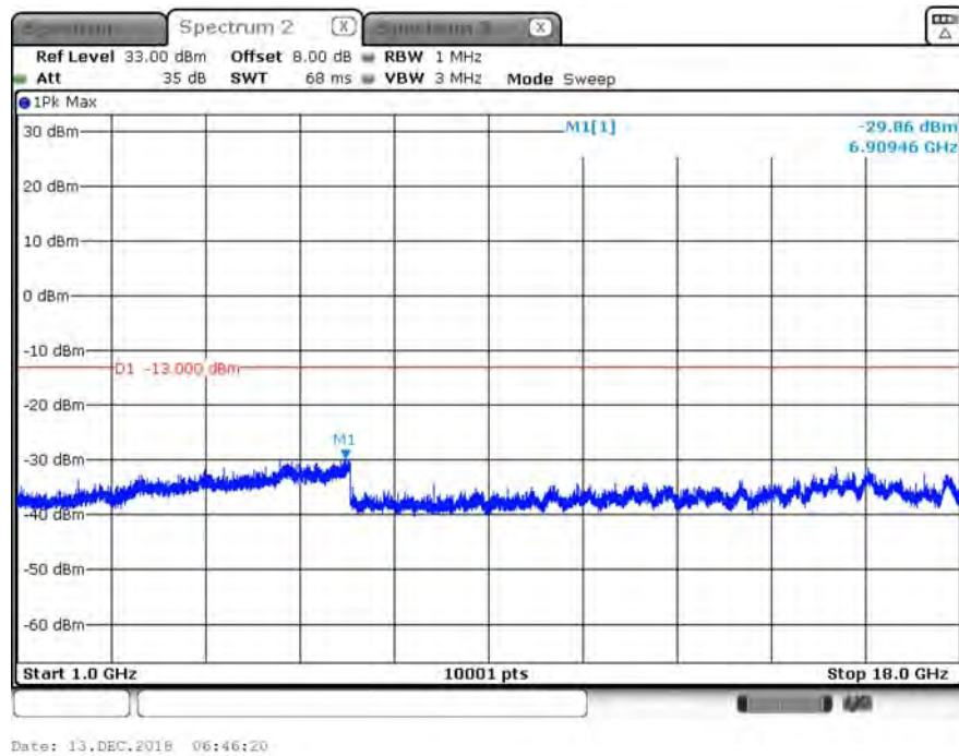
B12_10M_CH23060_QPSK_above 1G_1RB0
