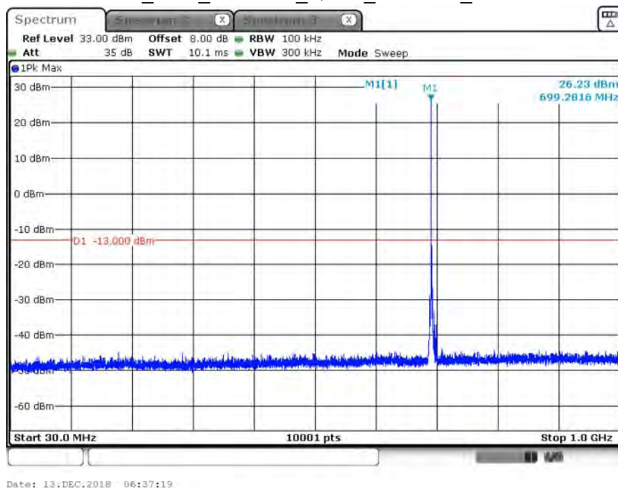
B12_1.4M_CH23017_QPSK_under 1G_1RB0
