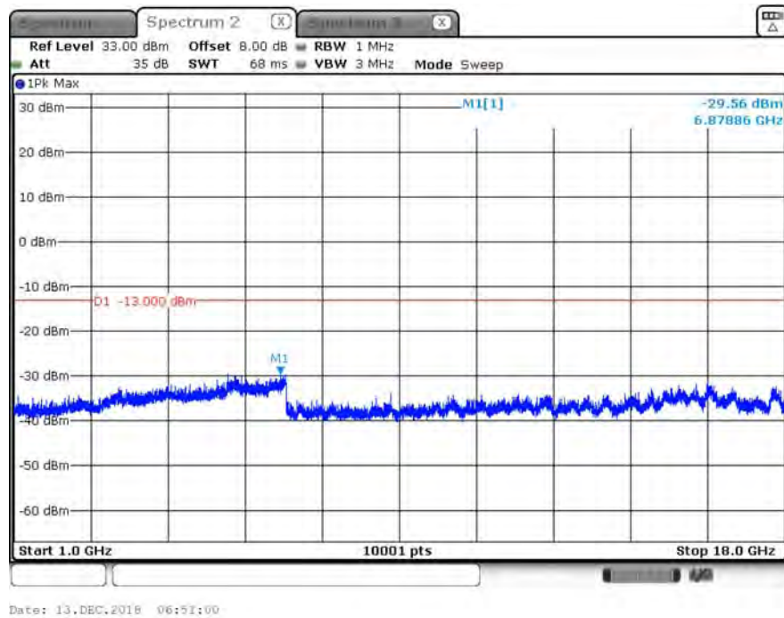
B17_10M_CH23780_QPSK_above 1G_1RB0
