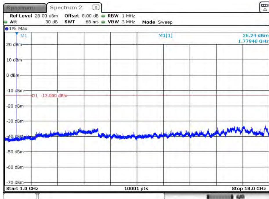
B66_1.4M_CH132665_16QAM_above 1G_1RB0
