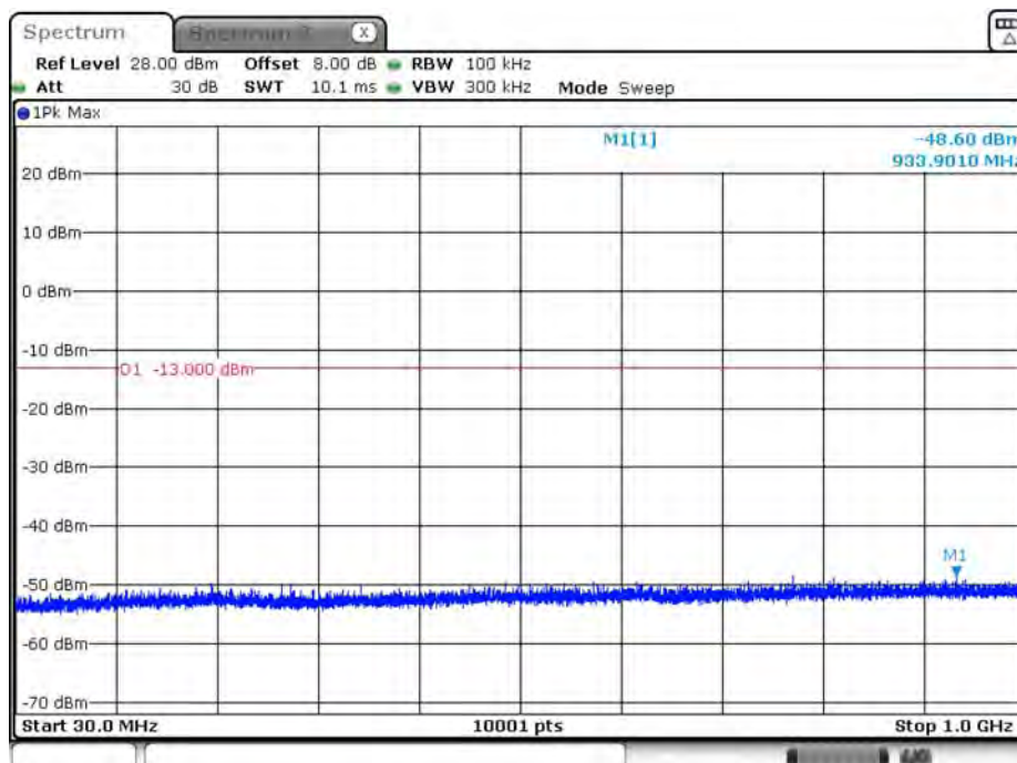
B66_1.4M_CH132322_16QAM_under 1G_1RB0
