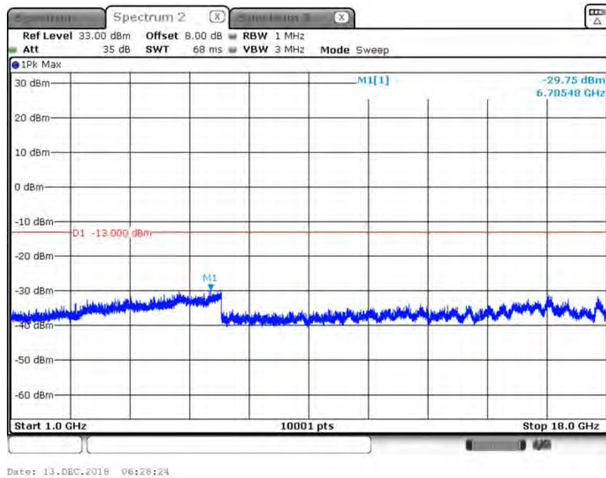
B5_10M_CH20450_QPSK_above 1G_1RB0
