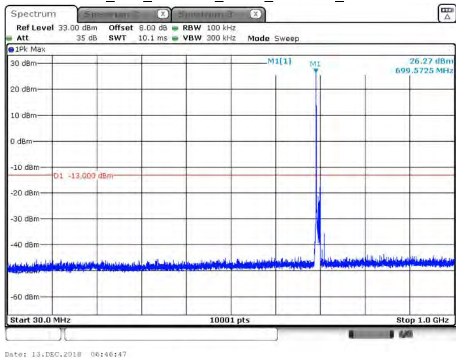
B12_10M_CH23060_QPSK_under 1G_1RB0
