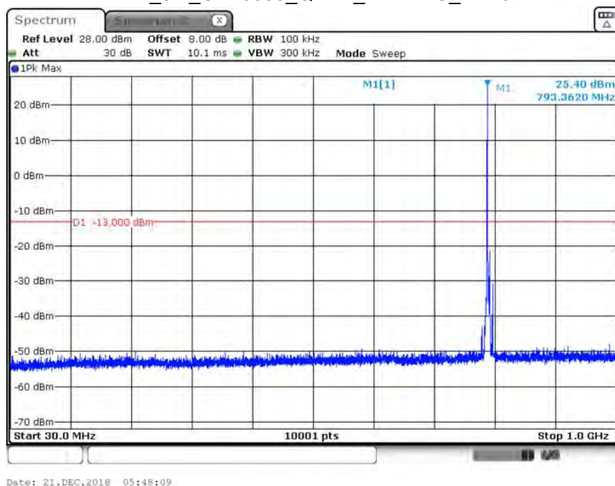
B14_5M_CH23355_QPSK_under 1G_1RB0
