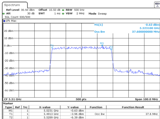
802.11ax40_5510MHz_RU_Full_Chain 1
