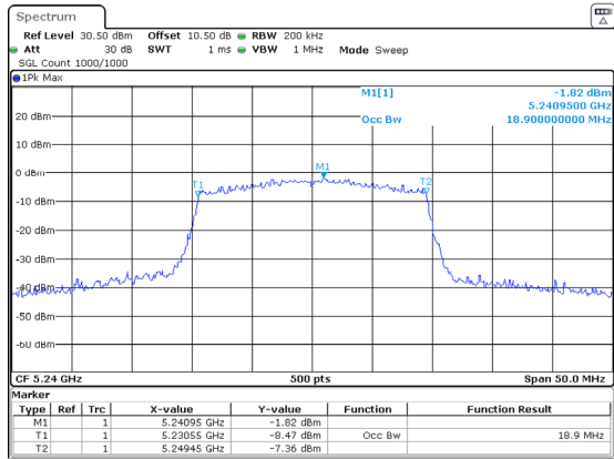
802.11ax20_5240MHz_RU_Full_Chain 1
