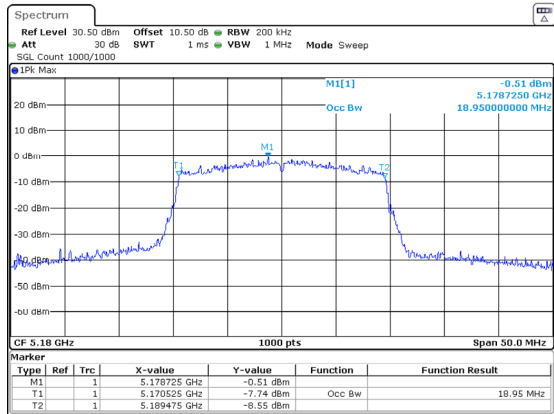
802.11ax20_5180MHz_RU_Full_Chain 1
