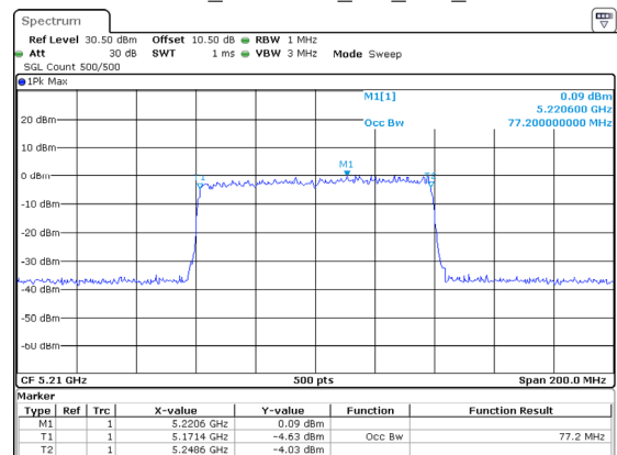
802.11ax80_5210MHz_RU_Full_Chain 2
