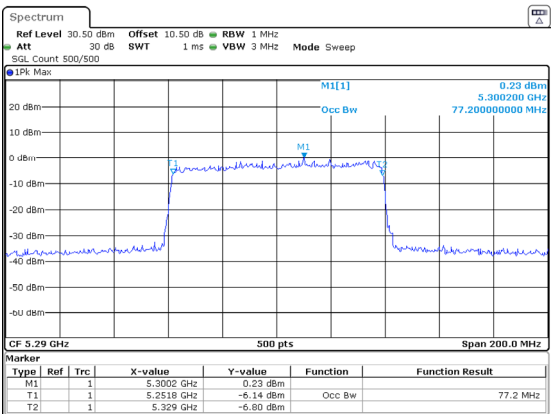
802.11ax80_5290MHz_RU_Full_Chain 1
