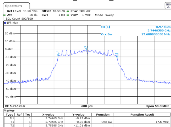
802.11ac20_5745MHz_Chain 1
