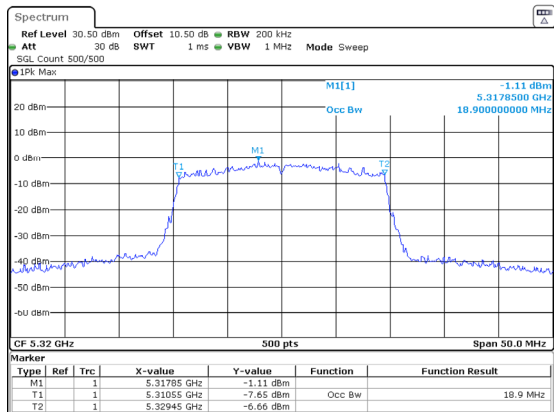
802.11ax20_5320MHz_RU_Full_Chain 1
