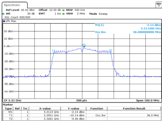
802.11ac40_5310MHz_Chain 2
