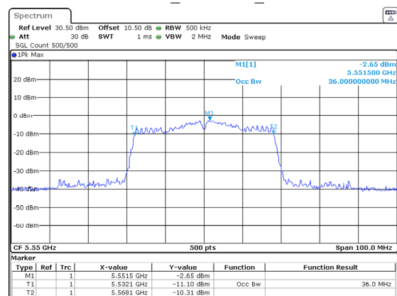
802.11ac40_5550MHz_Chain 1
