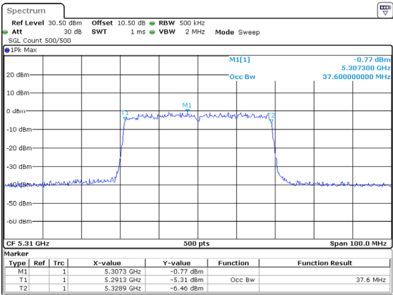
802.11ax40_5310MHz_RU_Full_Chain 2
