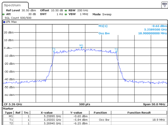
802.11ax20_5260MHz_RU_Full_Chain 2
