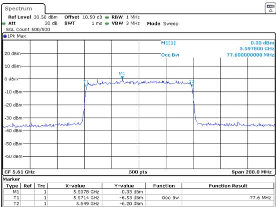
802.11ax80_5610MHz_RU_Full_Chain 1
