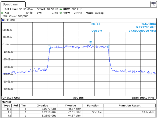
802.11ax40_5270MHz_RU_Full_Chain 1
