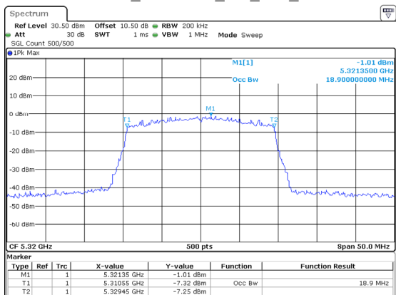
802.11ax20_5320MHz_RU_Full_Chain 2
