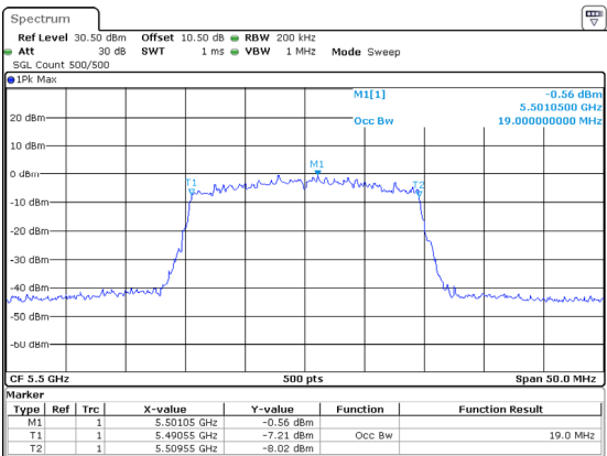
802.11ax20_5500MHz_RU_Full_Chain 2
