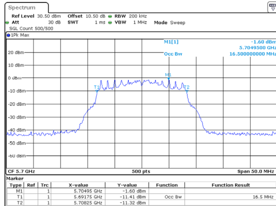
802.11a_5700MHz_Chain 2
