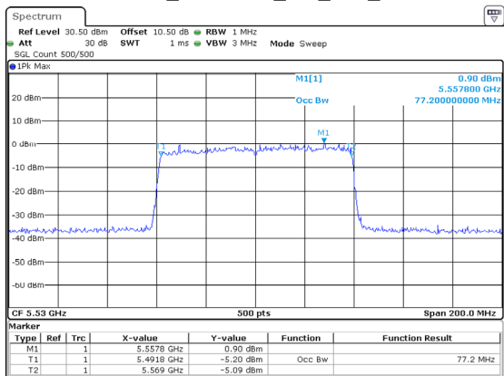
802.11ax80_5530MHz_RU_Full_Chain 2
