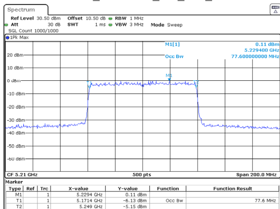
802.11ax80_5210MHz_RU_Full_Chain 1
