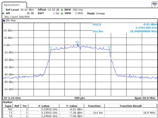
802.11ax20_5240MHz_RU_Full_Chain 2
