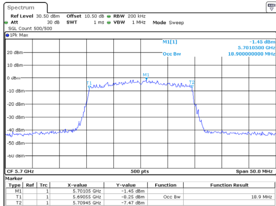
802.11ax20_5700MHz_RU_Full_Chain 2
