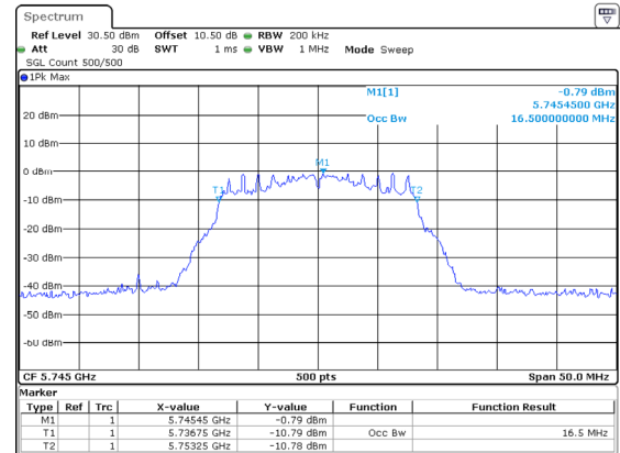
802.11a_5745MHz_Chain 2
