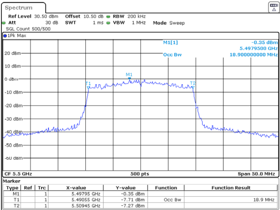
802.11ax20_5500MHz_RU_Full_Chain 1
