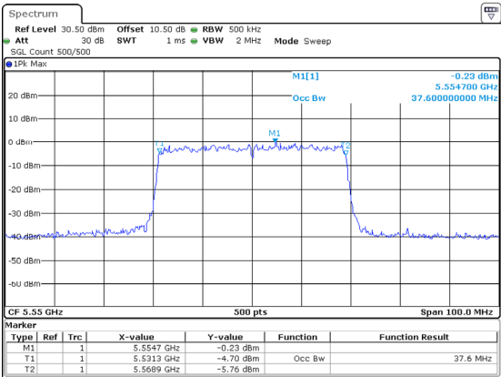
802.11ax40_5550MHz_RU_Full_Chain 2
