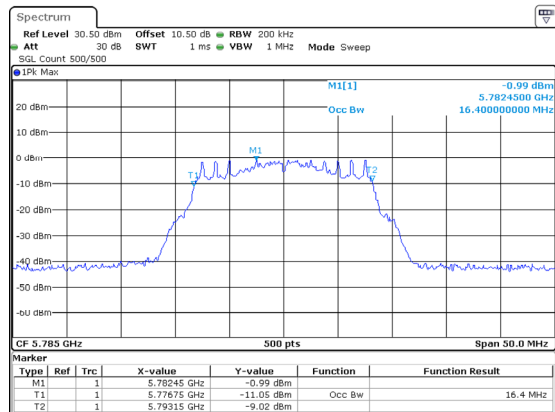
802.11a_5785MHz_Chain 2
