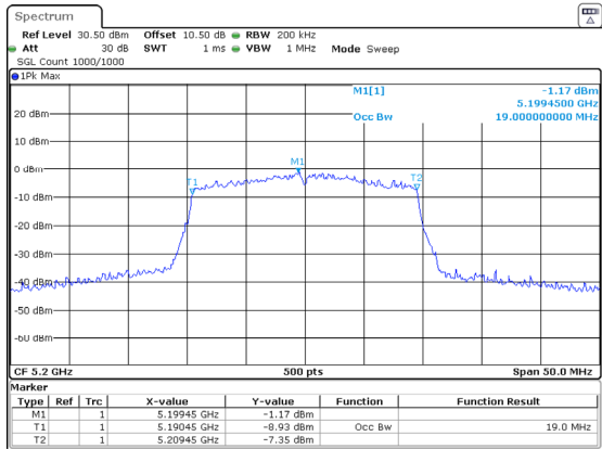
802.11ax20_5200MHz_RU_Full_Chain 1
