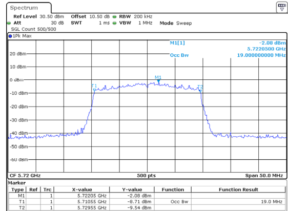
802.11ax20_5720MHz_RU_Full_Chain 2
