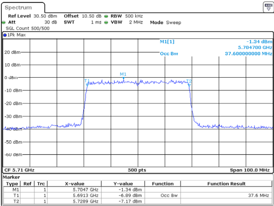
802.11ax40_5710MHz_RU_Full_Chain 2
