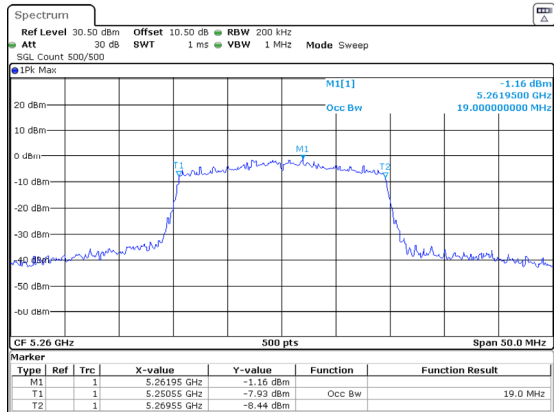
802.11ax20_5260MHz_RU_Full_Chain 1
