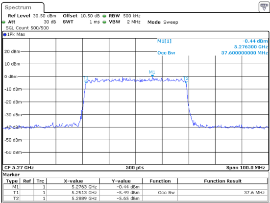
802.11ax40_5270MHz_RU_Full_Chain 2
