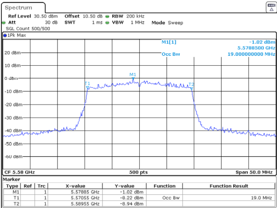
802.11ax20_5580MHz_RU_Full_Chain 1
