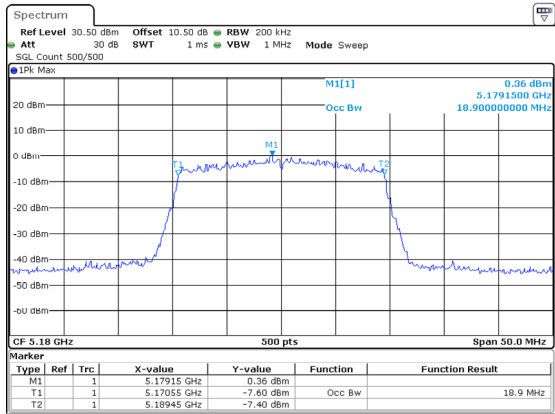
802.11ax20_5180MHz_RU_Full_Chain 2
