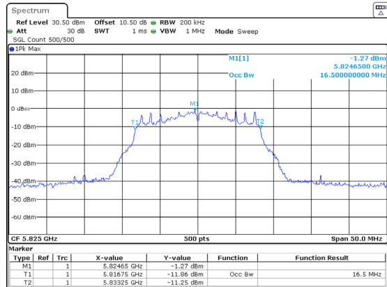
802.11a_5825MHz_Chain 1
