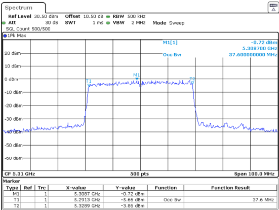
802.11ax40_5310MHz_RU_Full_Chain 1
