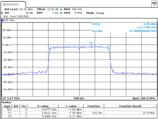
802.11ax40_5670MHz_RU_Full_Chain 2
