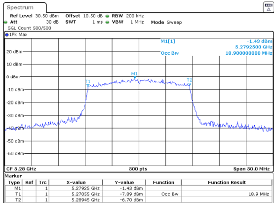
802.11ax20_5280MHz_RU_Full_Chain 1
