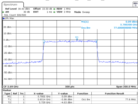
802.11ax80_5690MHz_RU_Full_Chain 1
