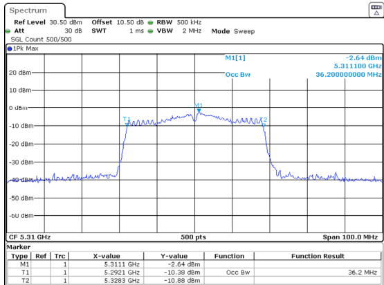
802.11ac40_5310MHz_Chain 1
