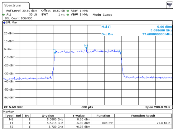
802.11ax80_5690MHz_RU_Full_Chain 2
