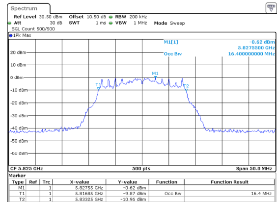
802.11a_5825MHz_Chain 2
