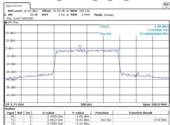
802.11ax40_5710MHz_RU_Full_Chain 1
