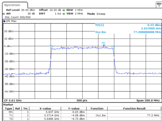
802.11ax80_5610MHz_RU_Full_Chain 2
