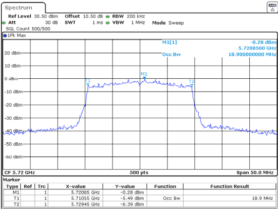
802.11ax20_5720MHz_RU_Full_Chain 1
