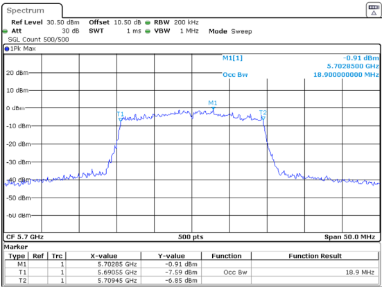
802.11ax20_5700MHz_RU_Full_Chain 1
