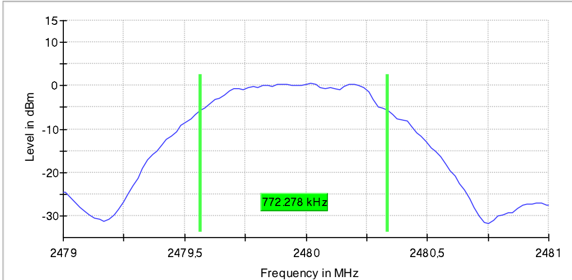
6 dB Bandwidth
