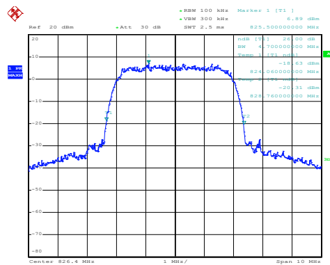
26dB Emission Bandwidth
