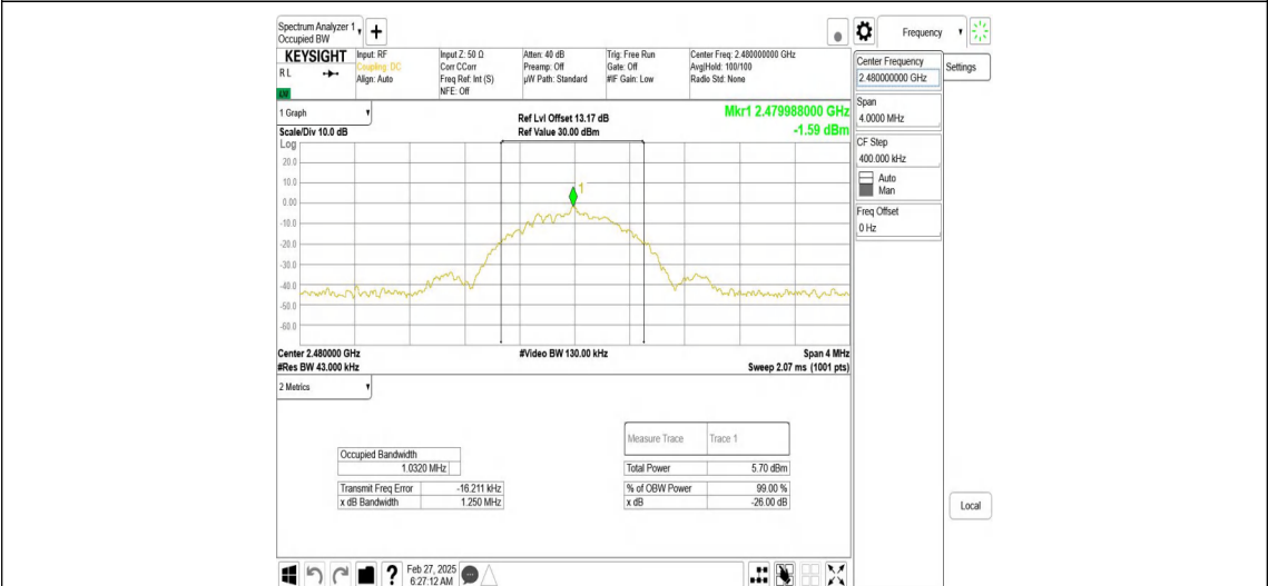
BLE_1M_Ant1_2480
