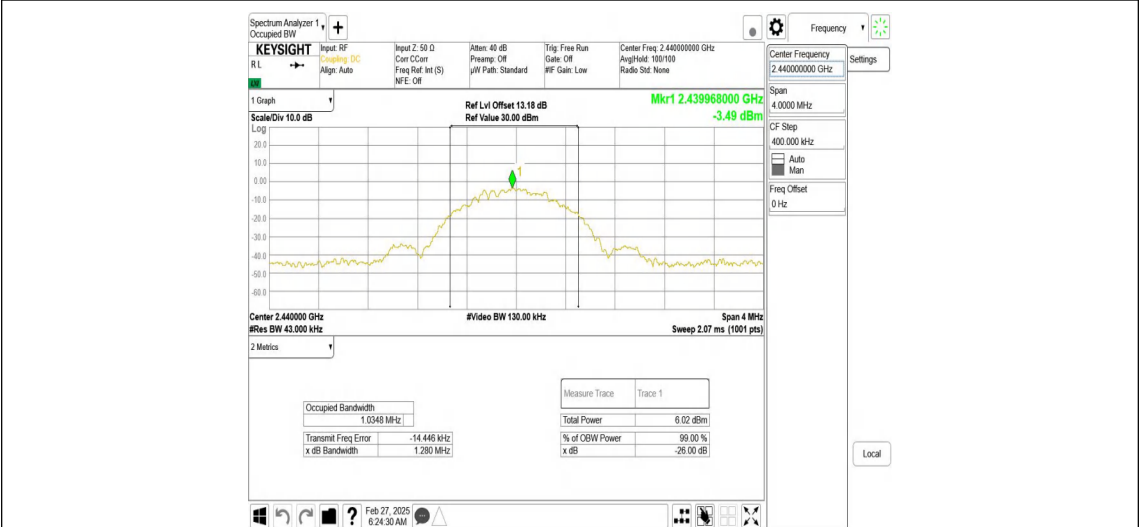
BLE_1M_Ant1_2440
