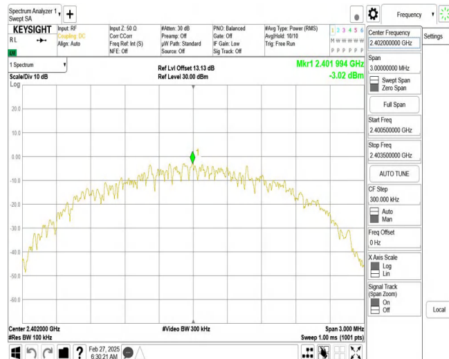
BLE_2M_Ant1_2402_0~Reference
