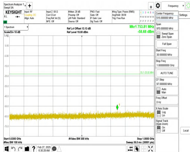
BLE_2M_Ant1_2402_30~1000
