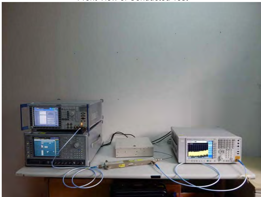
Front View of Conducted Test
