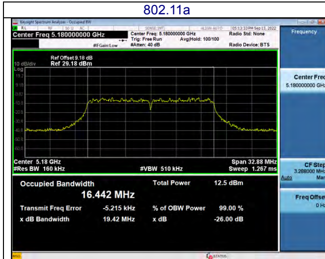
CH36-5180MHz
