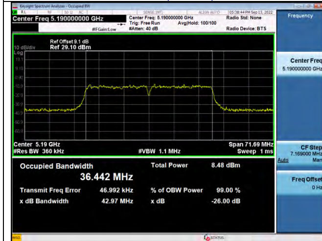
CH38-5190MHz
