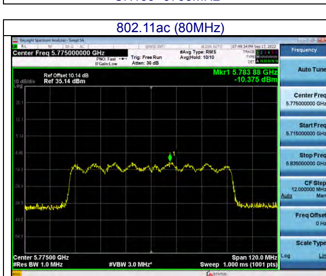
CH155 -5775MHz
