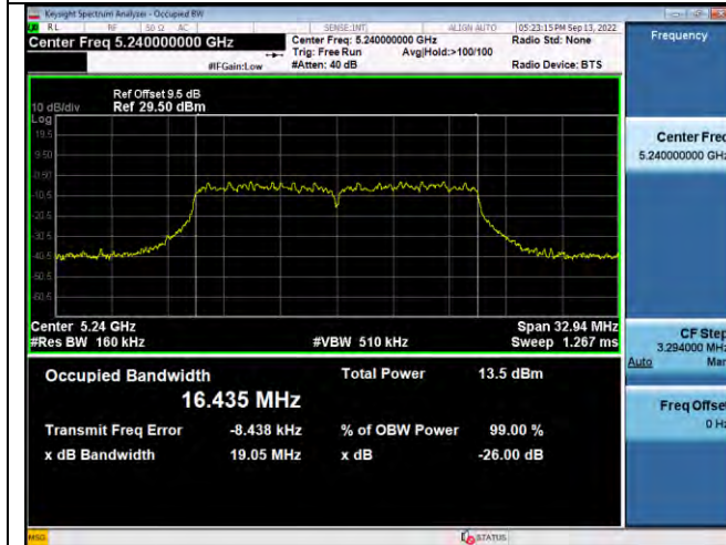
CH48-5240MHz
