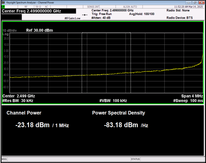
Band7 16QAM BW=20MHz Channel=20850 RB Size=27 Position=#0 Normal
