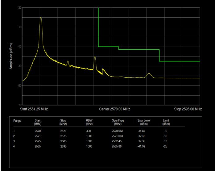
Band7 16QAM BW=15MHz Channel=21375 RB Size=27 Position=#0 Extended
