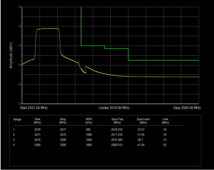
Band7 16QAM BW=10MHz Channel=21400 RB Size=27 Position=#0 Normal
