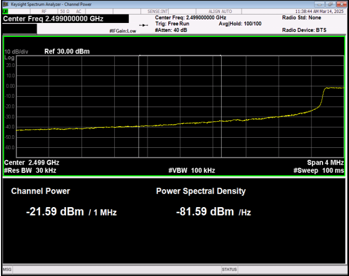
Band7 16QAM BW=15MHz Channel=20825 RB Size=27 Position=#0 Normal
