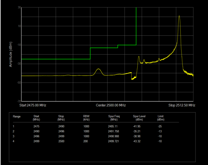
Band7 16QAM BW=10MHz Channel=20800 RB Size=27 Position=#0 Extended
