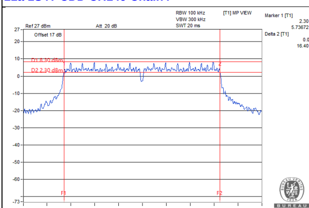
11a 1S4T CDD CH149 Chain4
