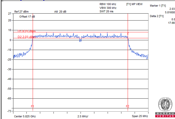
11ac (20MHz) 1S4T CDD CH165 Chain3
