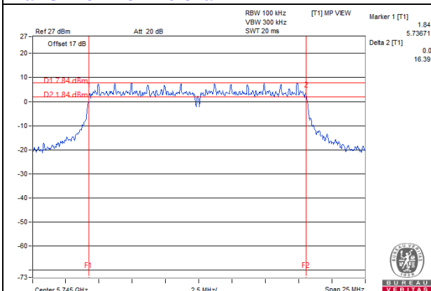
11a 1S4T CDD CH149 Chain2
