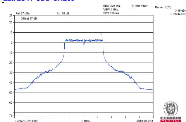
11a 1S4T CDD CH165
