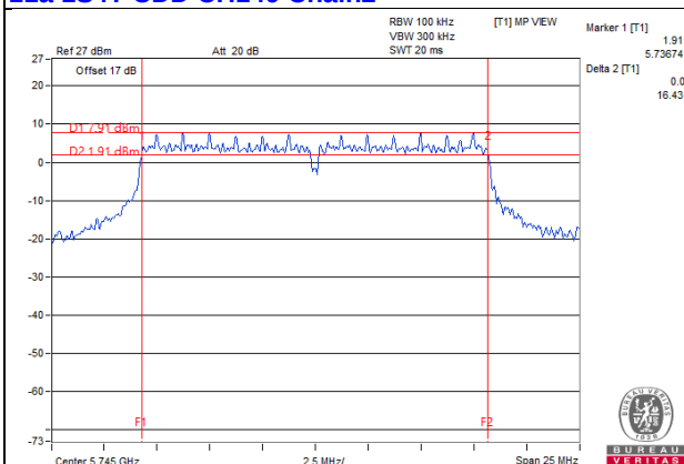
11a 1S4T CDD CH149 Chain3
