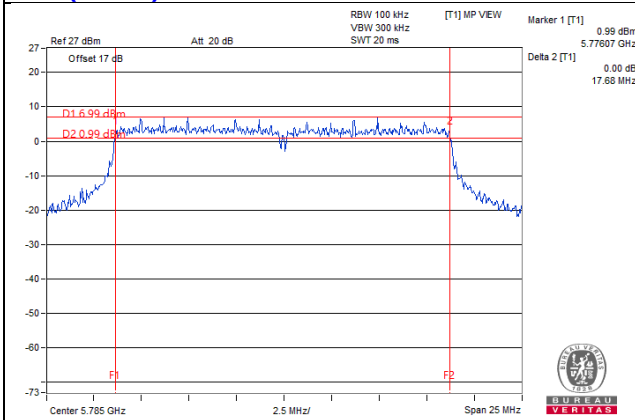
11ac (20MHz) 1S4T TxBF CH157 Chain3
