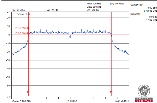
11ac (20MHz) 1S4T TxBF CH157 Chain4
