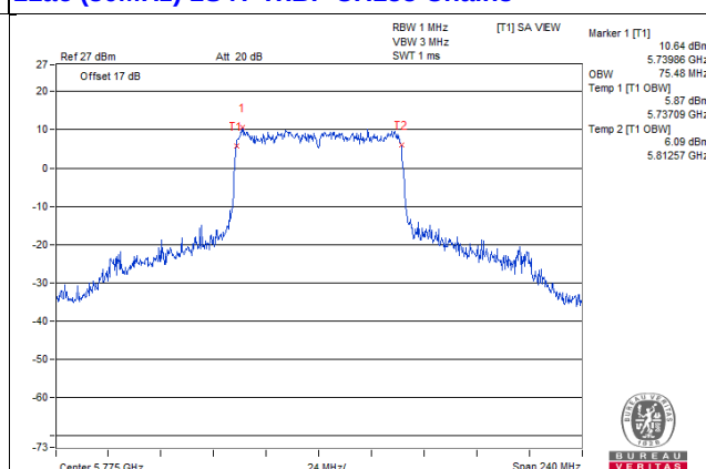
11ac (80MHz) 1S4T TxBF CH155 Chain4
