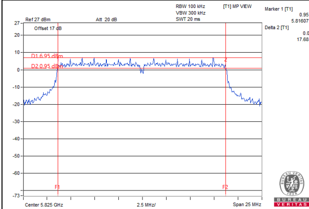
11ac (20MHz) 1S4T CDD CH165 Chain2
