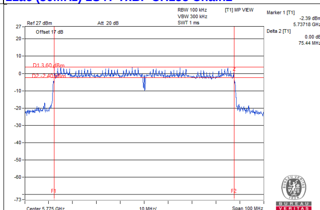
11ac (80MHz) 1S4T TxBF CH155 Chain3
