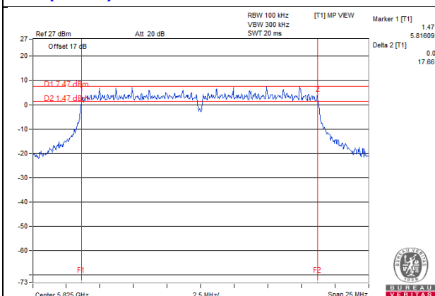
11ac (20MHz) 1S4T CDD CH165 Chain4
