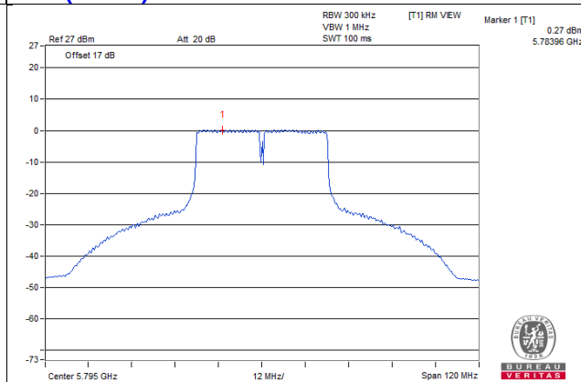
11ac (40MHz) 1S4T TXBF CH159
