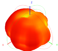
2400.0MHz H+V, Eff: 46.3%
