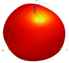
920.0MHz H+V, Eff: 1.7%
