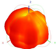
2430.0MHz H+V, Eff: 41.0%
