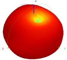
918.0MHz H+V, Eff: 1.9%
