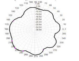
Total(H-XY), Max= 0.19dB, CirD=11.33
