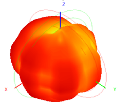
2420.0MHz H+V, Eff: 43.4%
