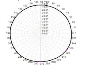
Total(H-XY), Max= -15.11dBi, CirD=1.38
