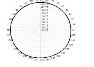
Total(H-XY), Max= -15.60dBi, CirD=1.37
