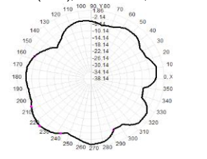
Total(H-XY), Max= 0.89dB, CirD=12.32
