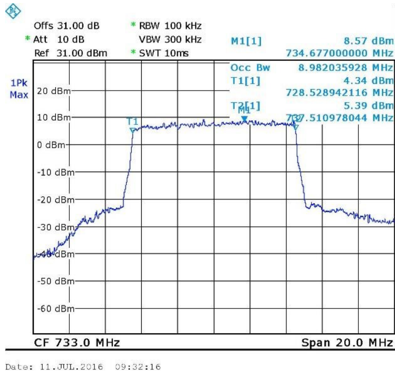
Figure 29. — 16QAM 733 MHz OUT
