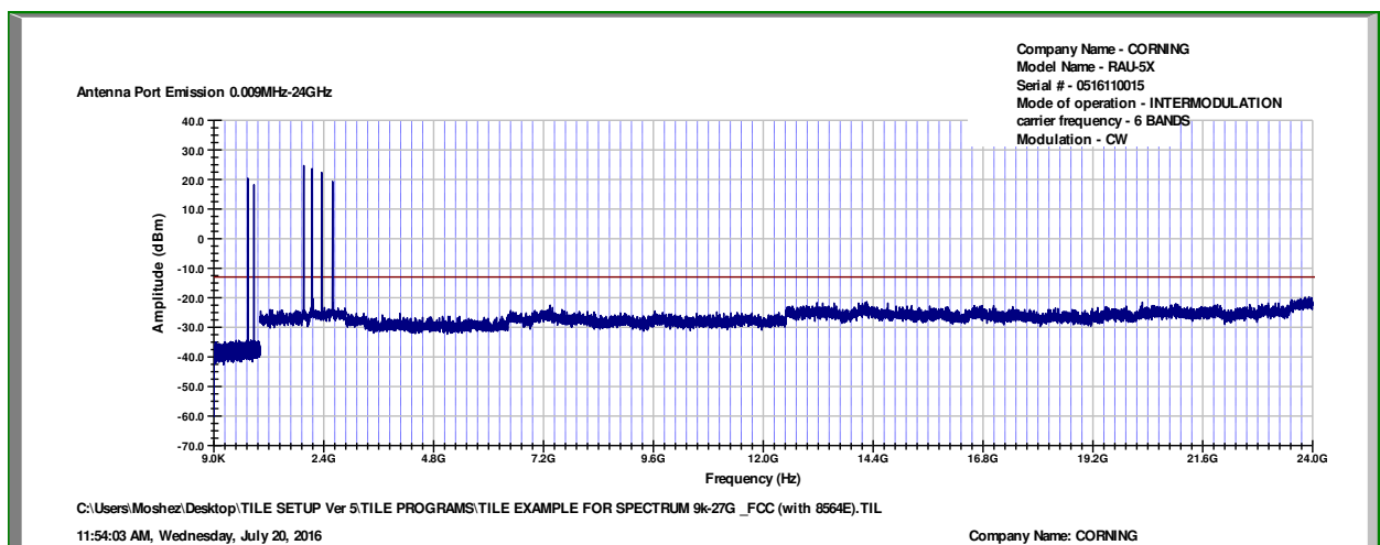
Figure 61 Intermodulation Conducted
