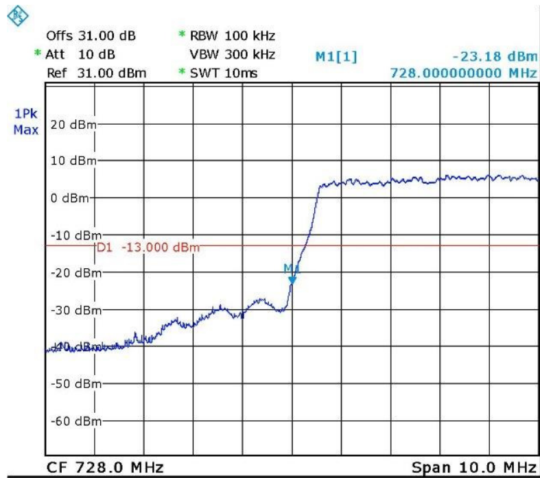
Figure 56. — QPSK 733.0 MHz
