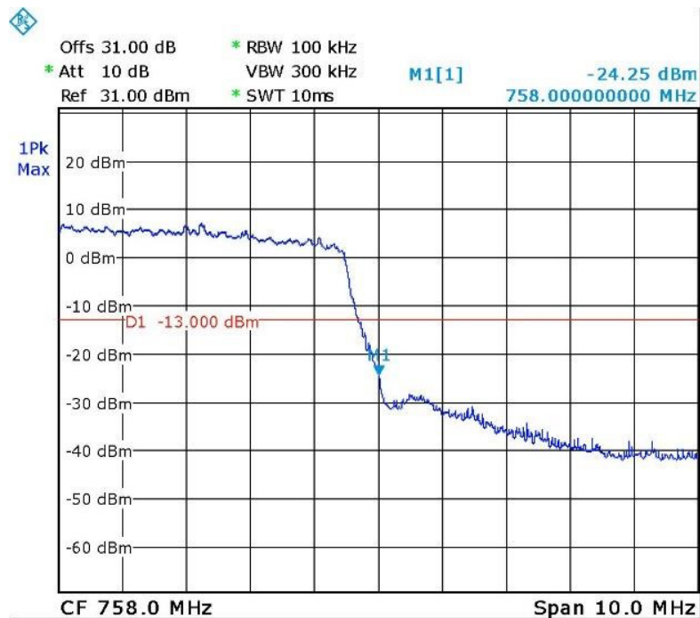
Figure 57. — QPSK 753.0 MHz
