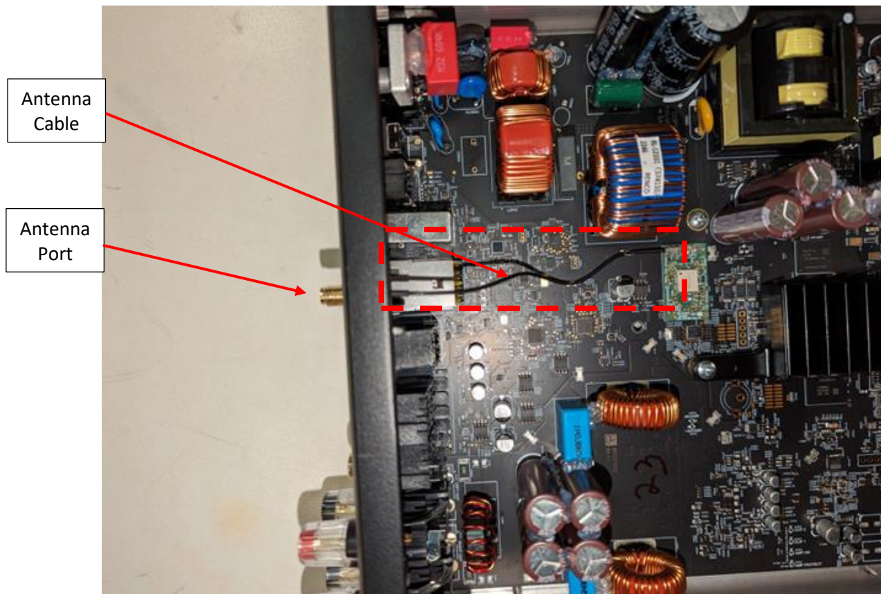
Photograph 4 – View of the Antenna Cable Routing
