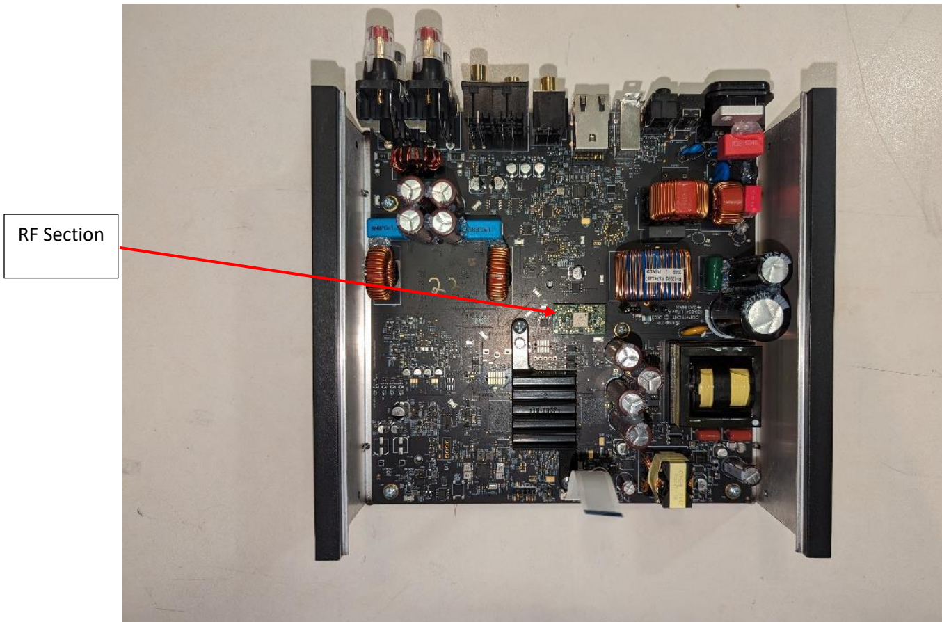
Photograph 2 – Top view of PCB in Housing
