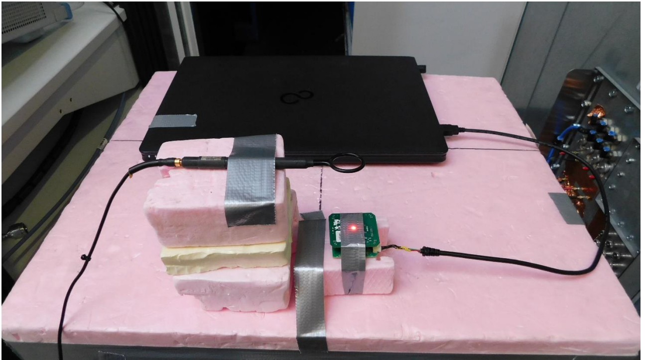
Picture 9: Bandwidth measurements
