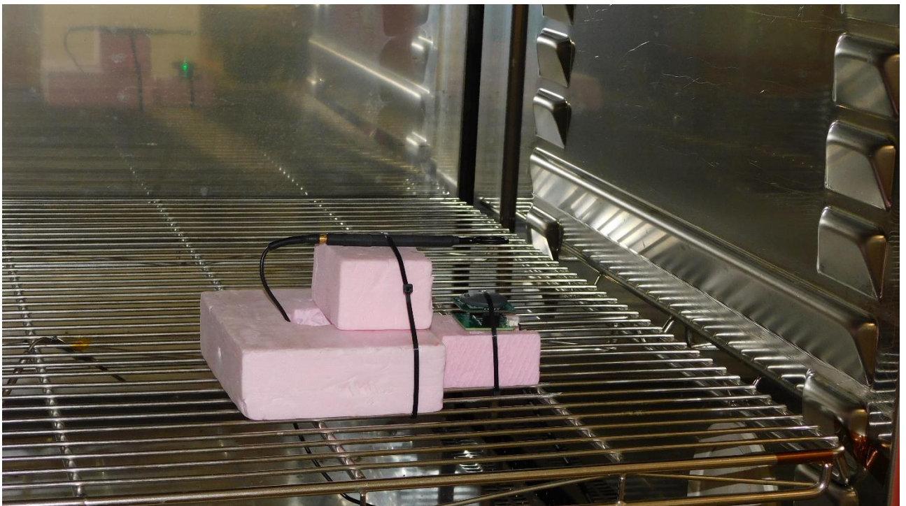
Picture 10: Carrier frequency stability test in climate chamber
