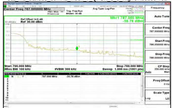
Cat M1_Band13 10MHz index 7 QPSK 6 0 HighCH23230-782
