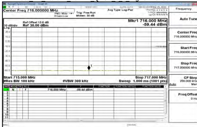
Cat M1 Band12 10MHz QPSK 6 0 HighCH23130-711
