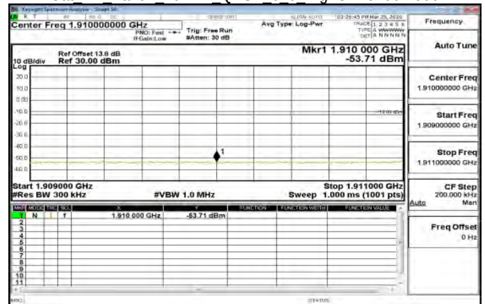
Cat M1 Band2 20MHz QPSK 6 0 HighCH19100-1900
