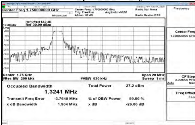
Cat M1 Band4 10MHz QPSK 6 0 Main HighCH20350-1750
