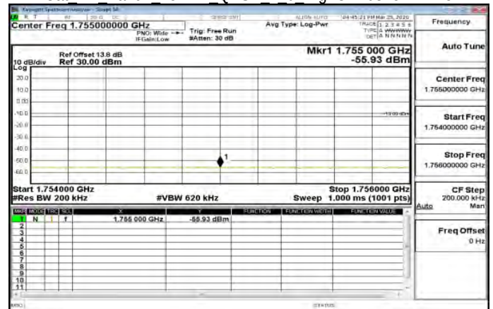
Cat M1 Band4 15MHz QPSK 1 0 HighCH20325-1747.5
