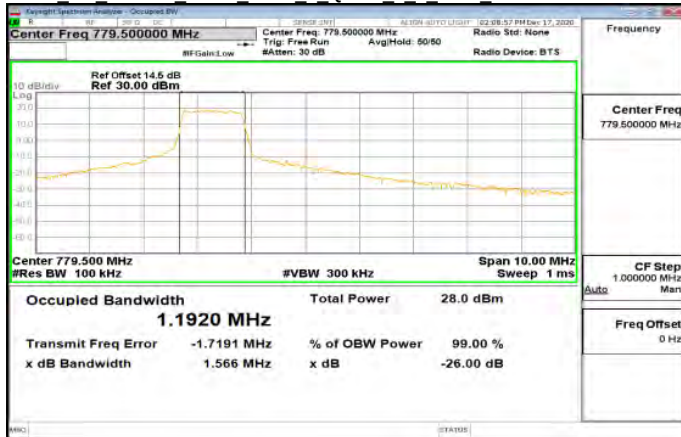
Cat M1 Band13 5MHz index 0 QPSK 6 0 Main LowCH23205-779.5
