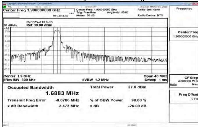
Cat M1 Band2 20MHz QPSK 6 0 Main HighCH19100-1900
