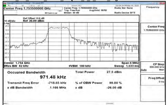
Cat M1 Band4 3MHz 16QAM 5 0 Main HighCH20385-1753.5
