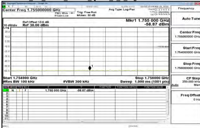
Cat M1 Band4 10MHz QPSK 1 0 HighCH20350-1750
