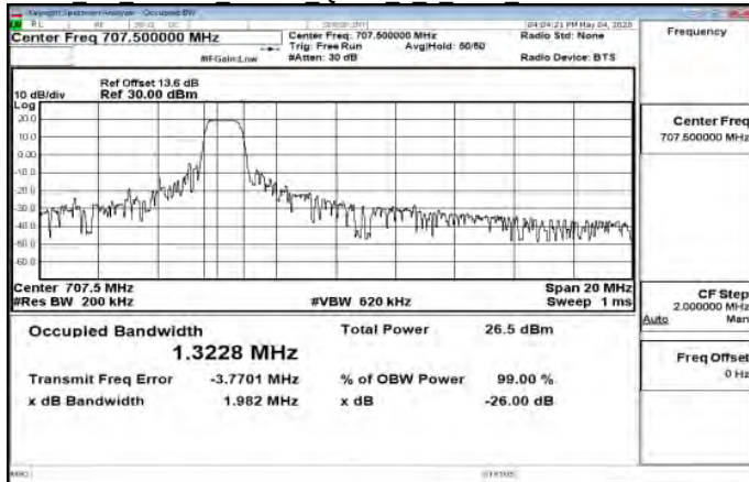
Cat M1 Band12 10MHz QPSK 6 0 Main HighCH23130-711
