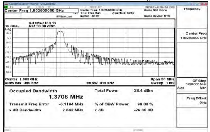
Cat M1 Band2 15MHz 16QAM 5 0 Main HighCH19125-1902.5
