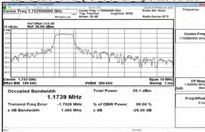
Cat M1 Band4 5MHz QPSK 6 0 Main HighCH20375-1752.5
