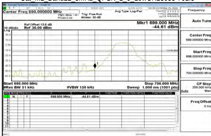
Cat M1 Band12 5MHz QPSK 1 0 LowCH23035-701.5
