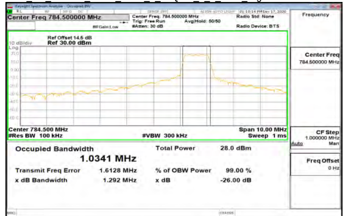
Cat M1 Band13 5MHz index 3 16QAM 5 0 Main HighCH23255-784.5
