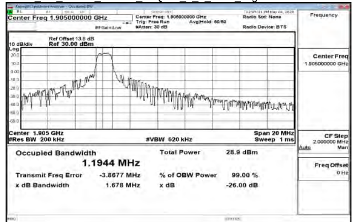
Cat M1 Band2 10MHz 16QAM 5 0 Main HighCH19150-1905
