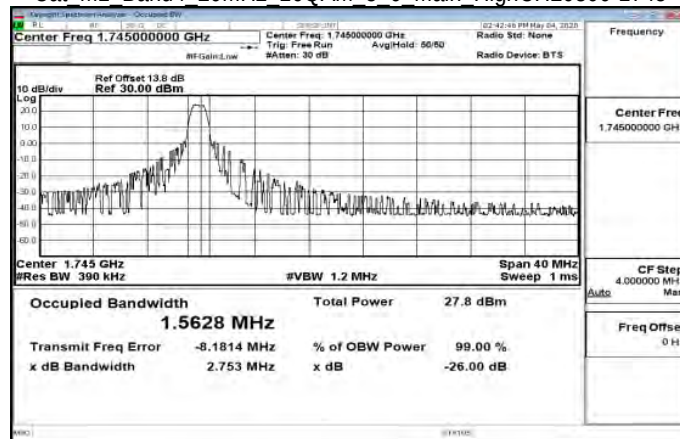
Cat M1 Band4 20MHz 16QAM 5 0 Main HighCH20300-1745
