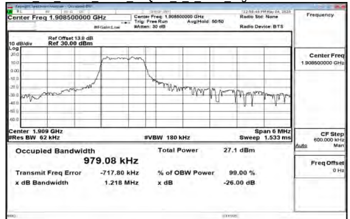
Cat M1 Band2 3MHz 16QAM 5 0 Main HighCH19185-1908.5
