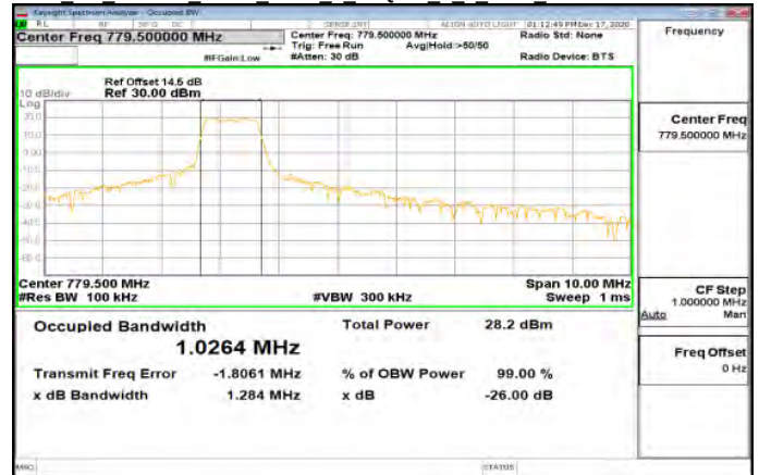
Cat M1 Band13 5MHz index 0 16QAM 5 0 Main LowCH23205-779.5
