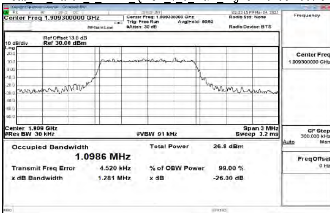
Cat M1 Band2 1 4MHz QPSK 6 0 Main HighCH19193-1909.3
