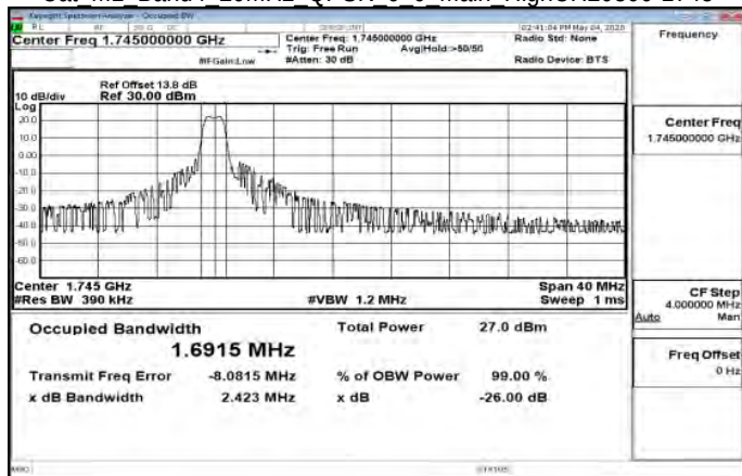
Cat M1 Band4 20MHz QPSK 6 0 Main HighCH20300-1745
