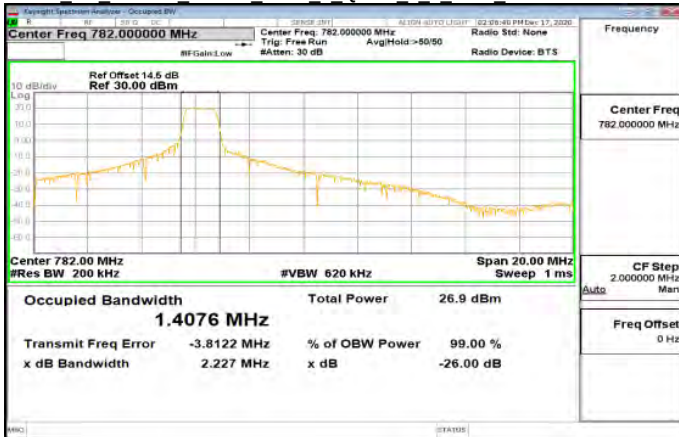
Cat M1 Band13 10MHz index 0 QPSK 6 0 Main MidCH23230-782
