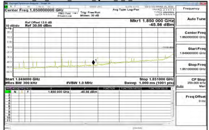
Cat M1 Band2 20MHz QPSK 6 0 LowCH18700-1860
