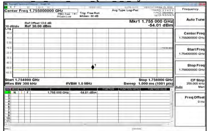
Cat M1 Band4 20MHz QPSK 6 0 HighCH20300-1745
