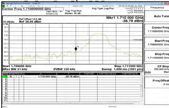
Cat M1 Band4 5MHz QPSK 1 0 LowCH19975-1712.5
