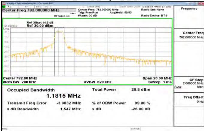
Cat M1 Band13 10MHz index 0 16QAM 5 0 Main MidCH23230-782
