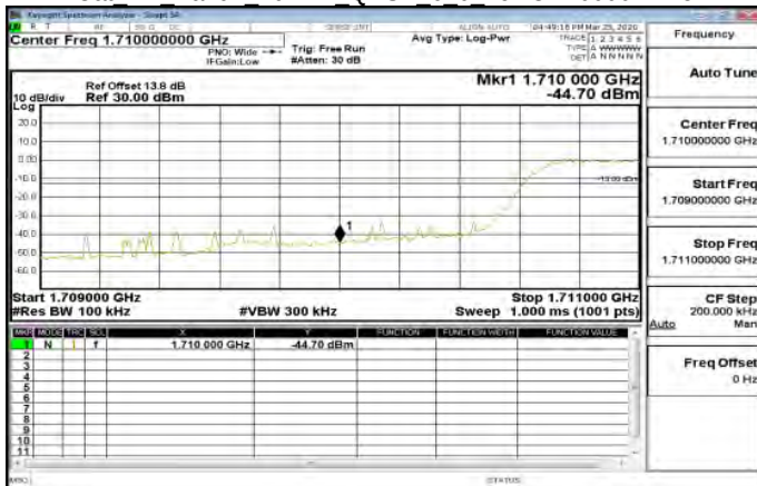
Cat M1 Band4 10MHz QPSK 6 0 LowCH20000-1715
