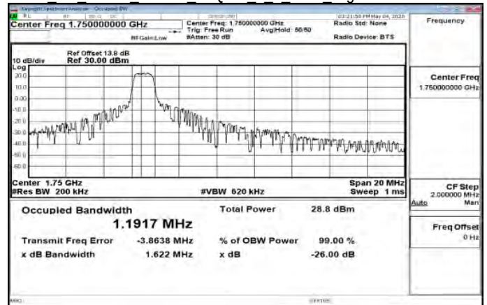
Cat M1 Band4 10MHz 16QAM 5 0 Main HighCH20350-1750
