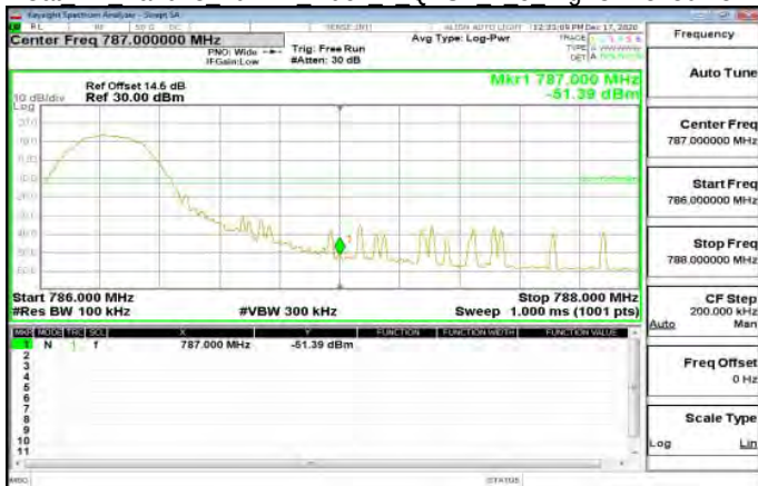
Cat M1_Band13 10MHz index 7 QPSK 1 5 HighCH23230-782
