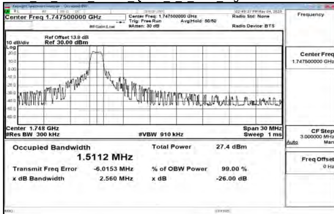
Cat M1 Band4 15MHz QPSK 6 0 Main HighCH20325-1747.5
