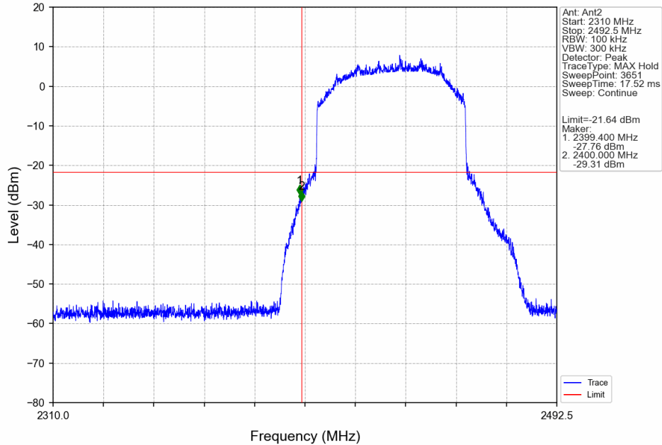
60M_LCH_2432.5MHz_Ant2_NTNV
