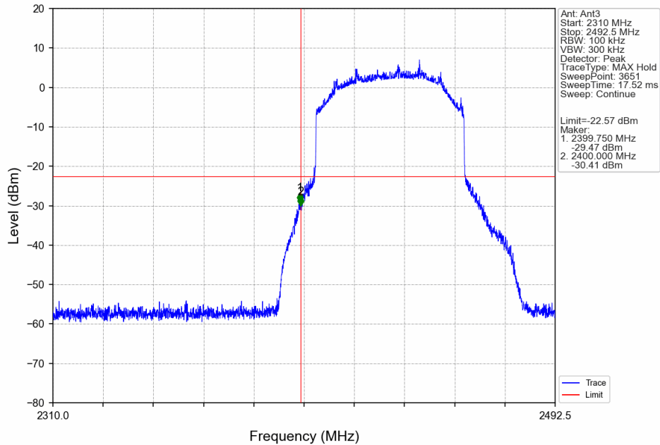
60M_LCH_2432.5MHz_Ant3_NTNV
