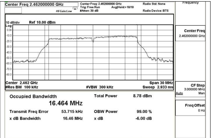
Channel 11 / 2462 MHz
