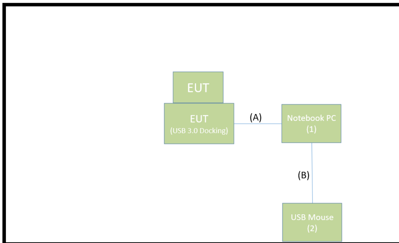
Connection Diagram
