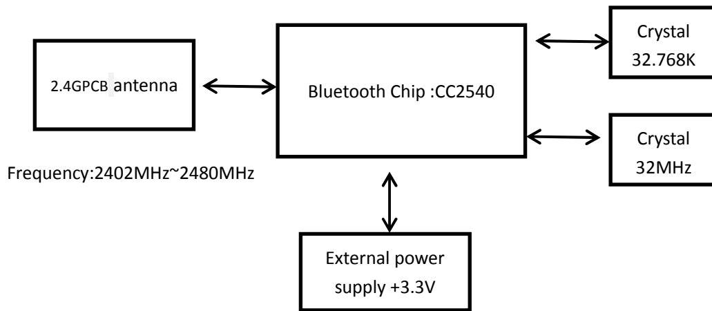
ZX_BLE_A3block diagram:
