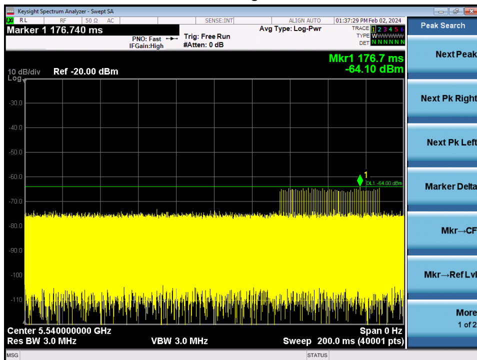
Radar Signal 1
