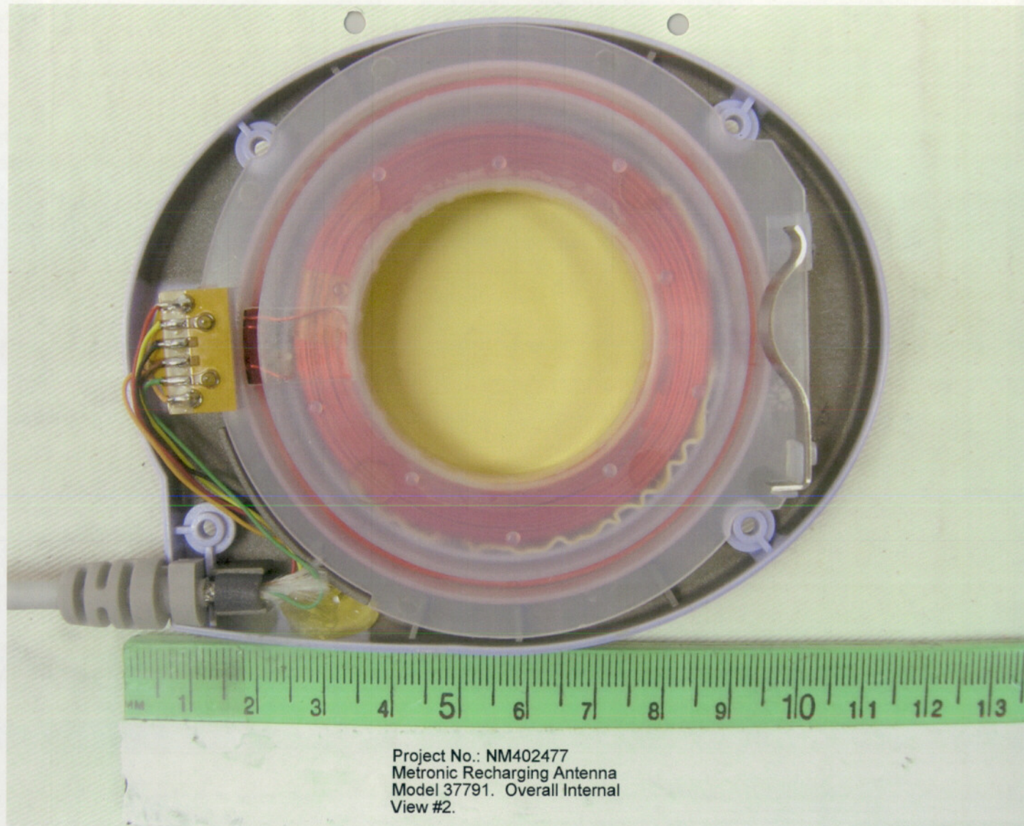
Medtronic INSR Programmer - Antenna Disassembly - View 2
