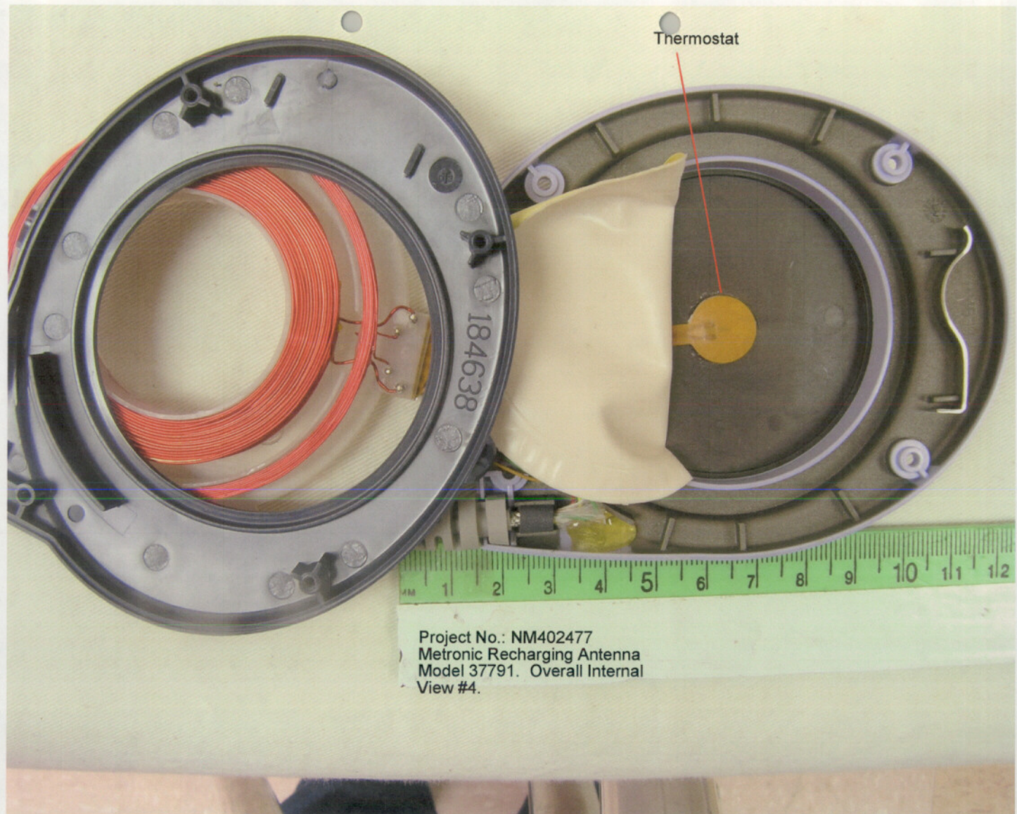
Medtronic INSR Programmer - Antenna Disassembly - View 4
