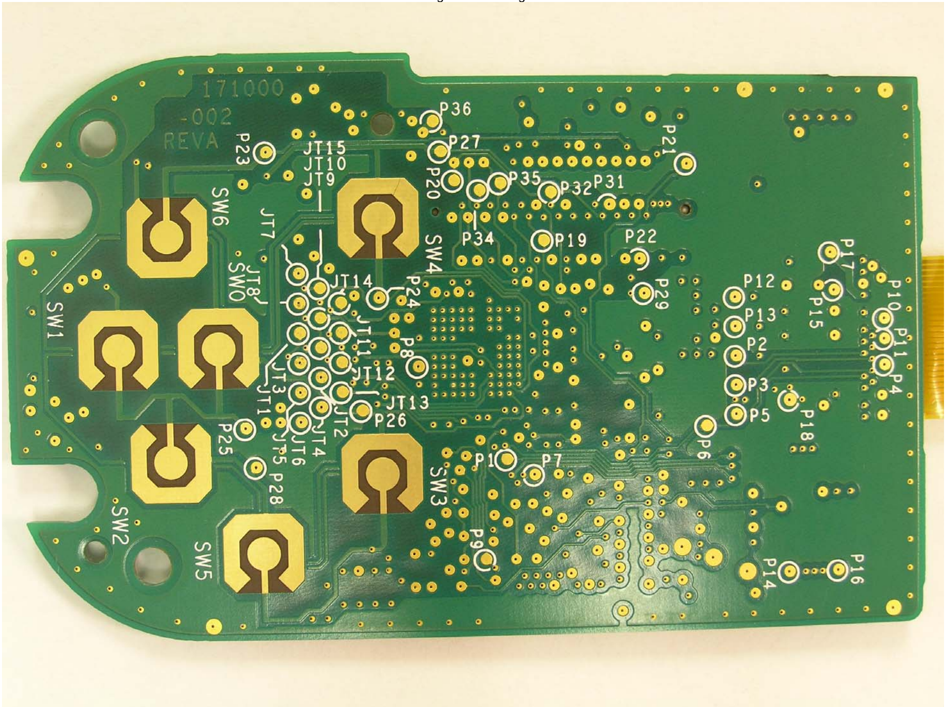
Medtronic INSR Programmer - Digital Board Bottom
