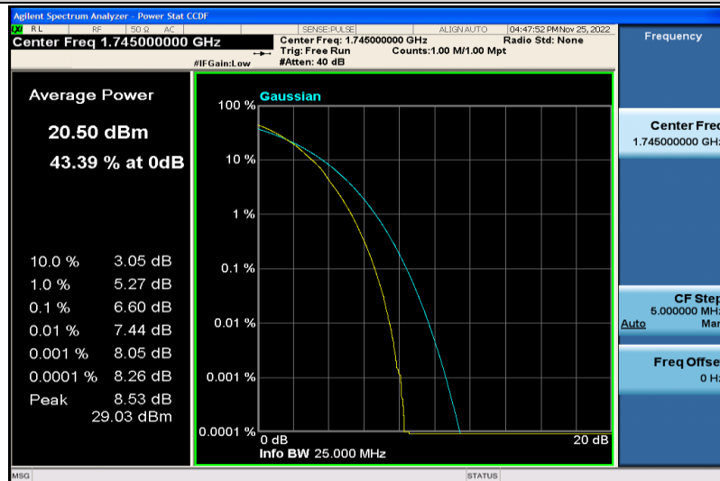
Band4-20MHz-64QAM-20300-100RB#0
