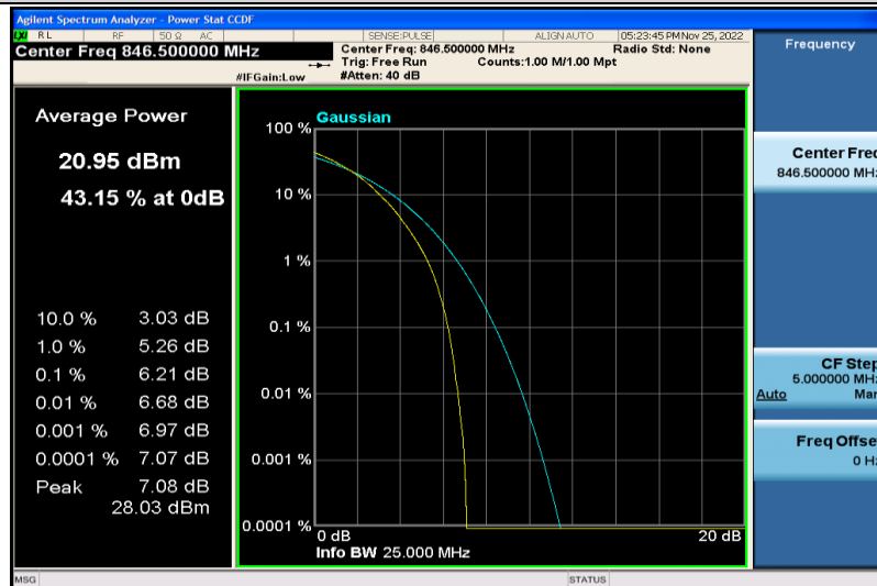
Band5-5MHz-64QAM-20625-25RB#0
