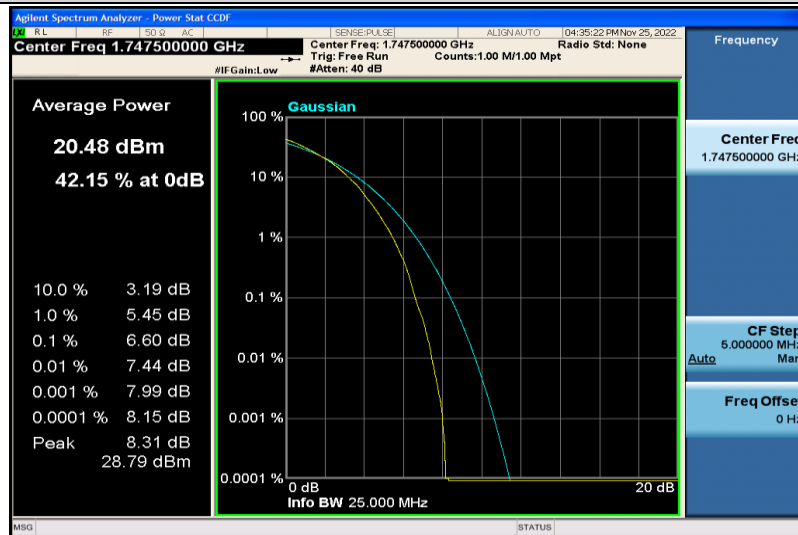
Band4-15MHz-64QAM-20325-75RB#0
