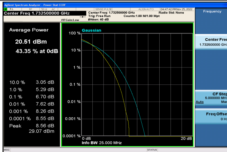
Band4-20MHz-64QAM-20175-100RB#0
