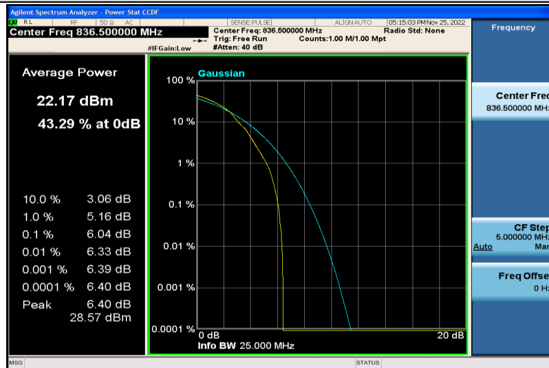
Band5-3MHz-64QAM-20525-1RB#0
