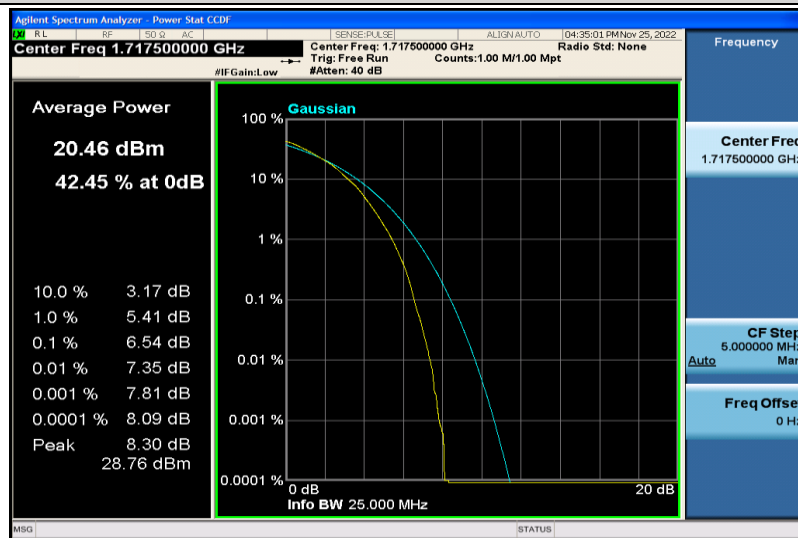
Band4-15MHz-64QAM-20025-75RB#0
