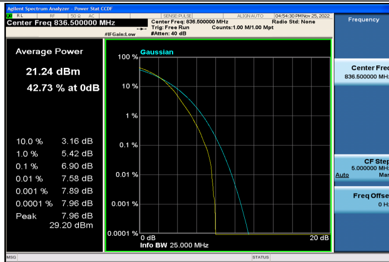
Band5-1.4MHz-64QAM-20525-6RB#0
