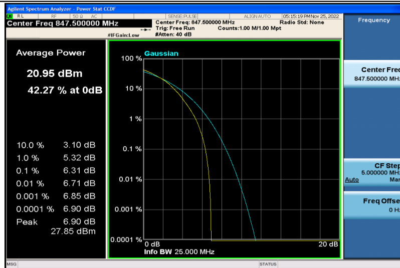
Band5-3MHz-64QAM-20635-15RB#0
