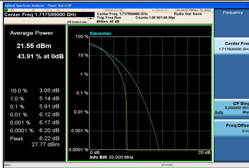
Band4-15MHz-64QAM-20025-1RB#0
