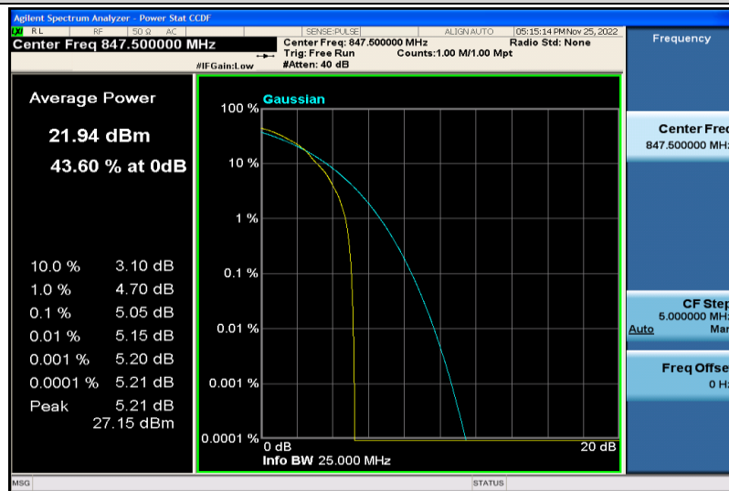
Band5-3MHz-64QAM-20635-1RB#0
