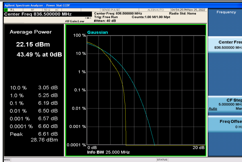
Band5-1.4MHz-64QAM-20525-1RB#0
