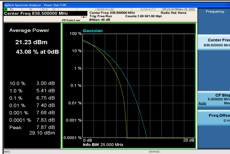
Band5-5MHz-64QAM-20525-25RB#0
