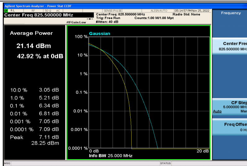
Band5-3MHz-64QAM-20415-15RB#0
