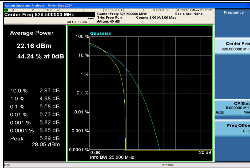
Band5-5MHz-64QAM-20425-1RB#0
