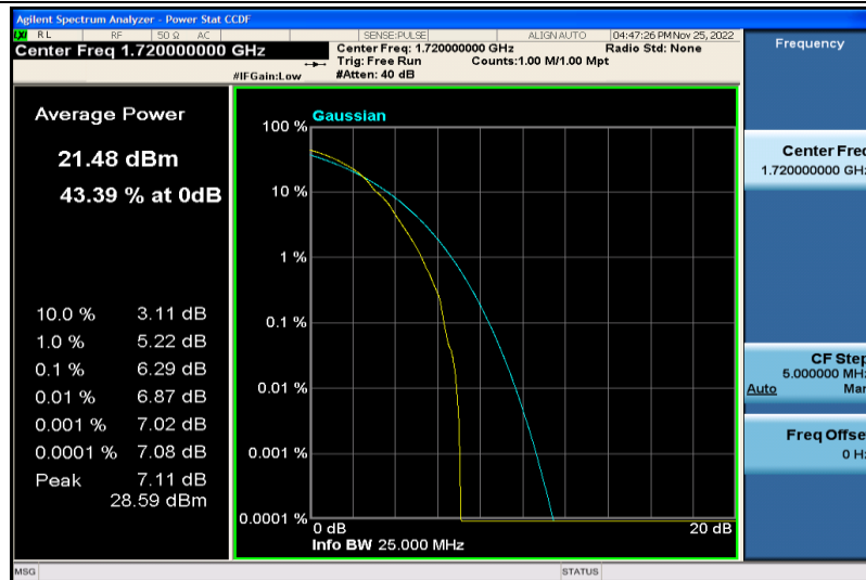
Band4-20MHz-64QAM-20050-1RB#0
