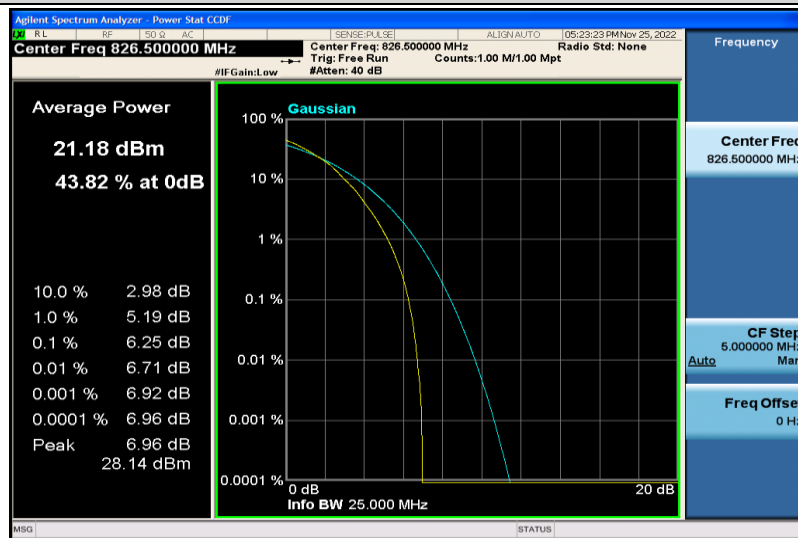
Band5-5MHz-64QAM-20425-25RB#0
