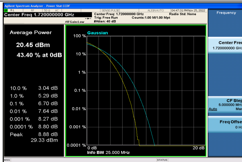
Band4-20MHz-64QAM-20050-100RB#0
