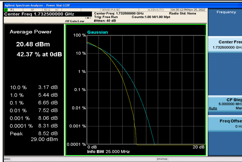
Band4-15MHz-64QAM-20175-75RB#0
