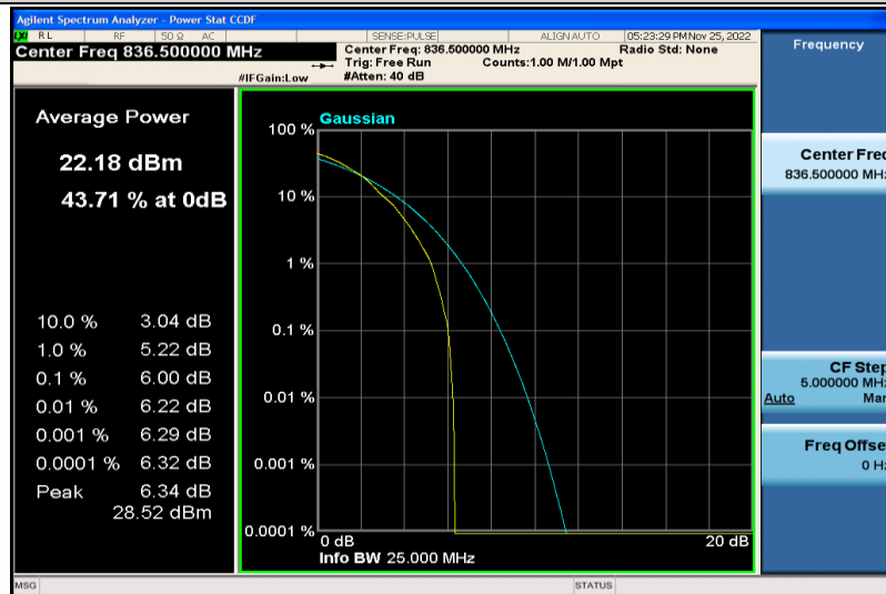
Band5-5MHz-64QAM-20525-1RB#0
