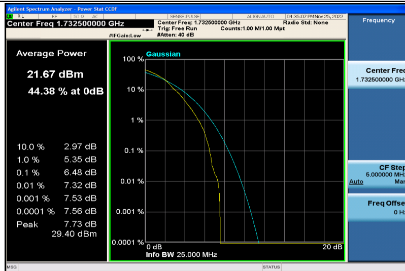
Band4-15MHz-64QAM-20175-1RB#0
