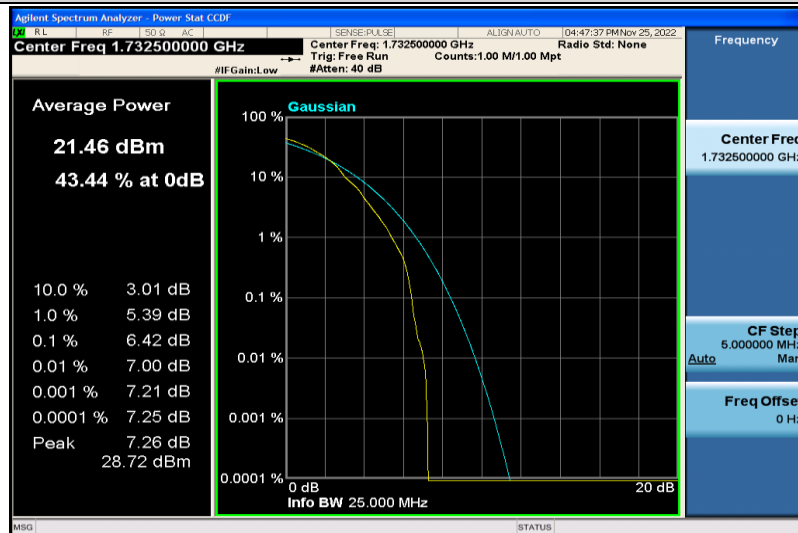
Band4-20MHz-64QAM-20175-1RB#0
