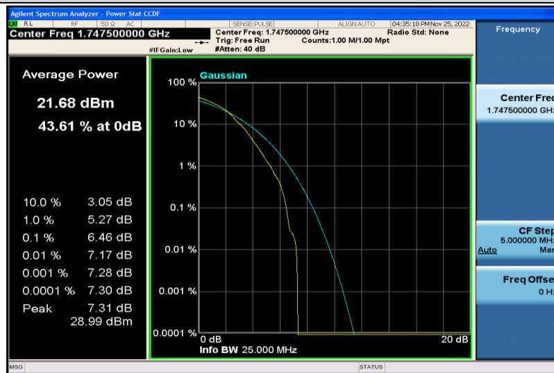
Band4-15MHz-64QAM-20325-1RB#0
