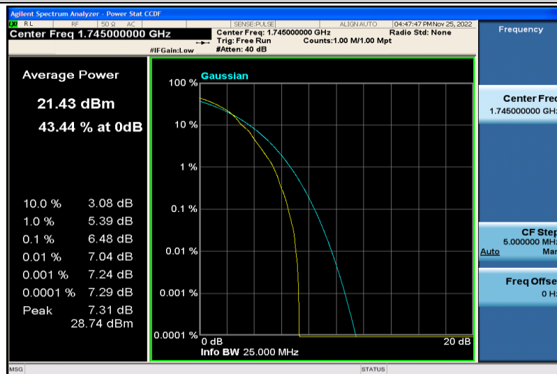
Band4-20MHz-64QAM-20300-1RB#0
