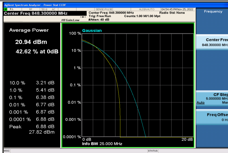
Band5-1.4MHz-64QAM-20643-6RB#0
