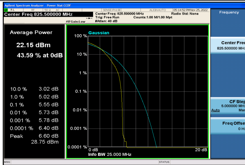
Band5-3MHz-64QAM-20415-1RB#0
