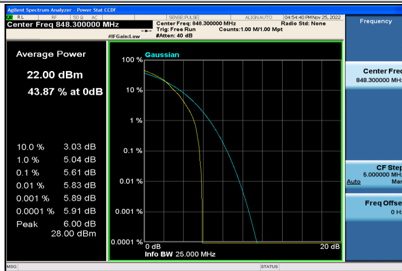
Band5-1.4MHz-64QAM-20643-1RB#0
