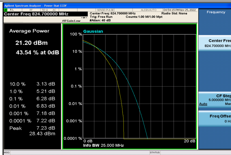
Band5-1.4MHz-64QAM-20407-6RB#0
