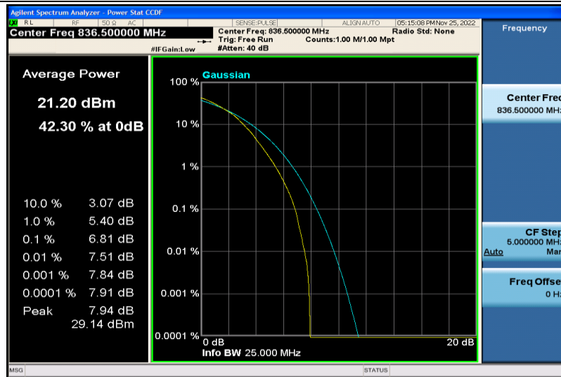
Band5-3MHz-64QAM-20525-15RB#0
