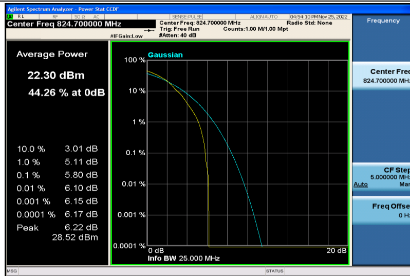
Band5-1.4MHz-64QAM-20407-1RB#0
