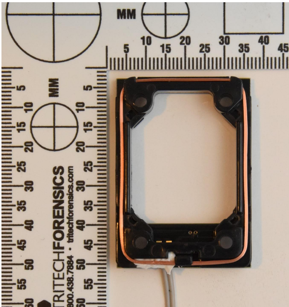
Combined LF/HF Antenna Back Side
