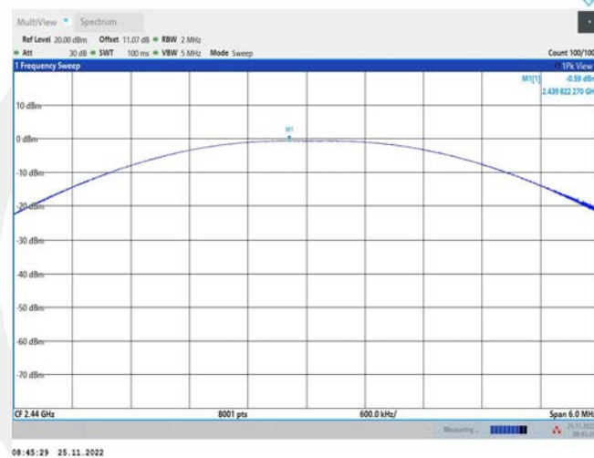
BLE_1M_Ant1_2440
