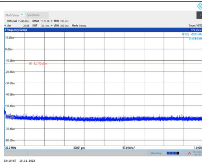
BLE_2M_Ant1_2402_30~1000
