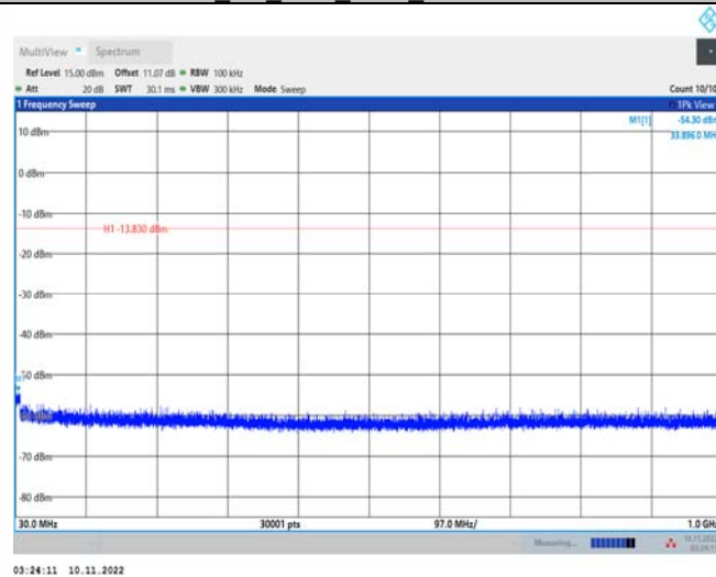
BLE_2M_Ant1_2440_30~1000
