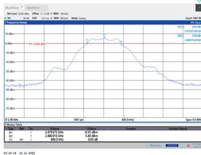
BLE_1M_Ant1_2480
