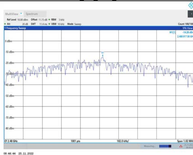
BLE_1M_Ant1_2480
