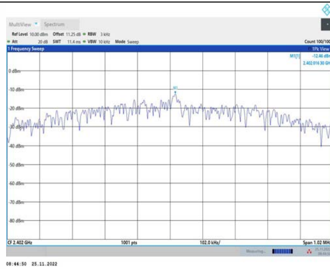
BLE_1M_Ant1_2402
