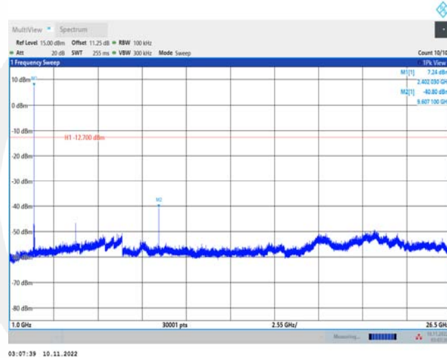
BLE_1M_Ant1_2402_1000~26500
