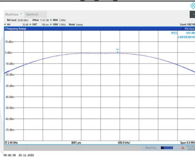
BLE_2M_Ant1_2440
