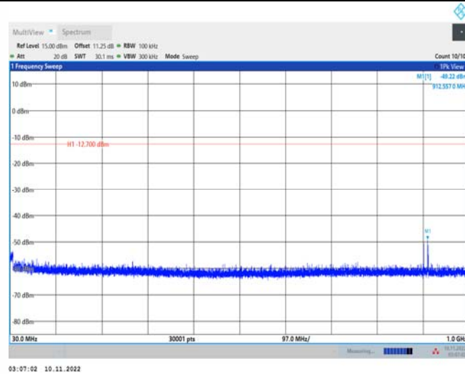
BLE_1M_Ant1_2402_30~1000
