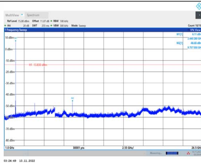
BLE_2M_Ant1_2440_1000~26500
