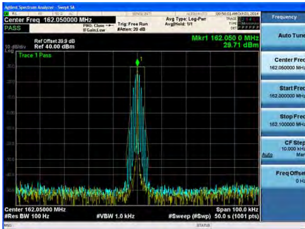
(4K00F2D _ 162.05 MHz)_Low
