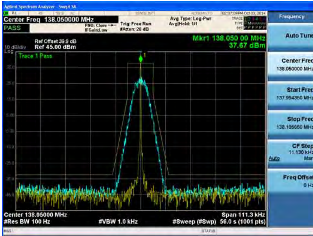
(8K10F1W _ 138.05 MHz)_High
