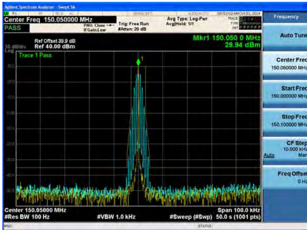
(4K00F2D _ 150.05 MHz)_Low
