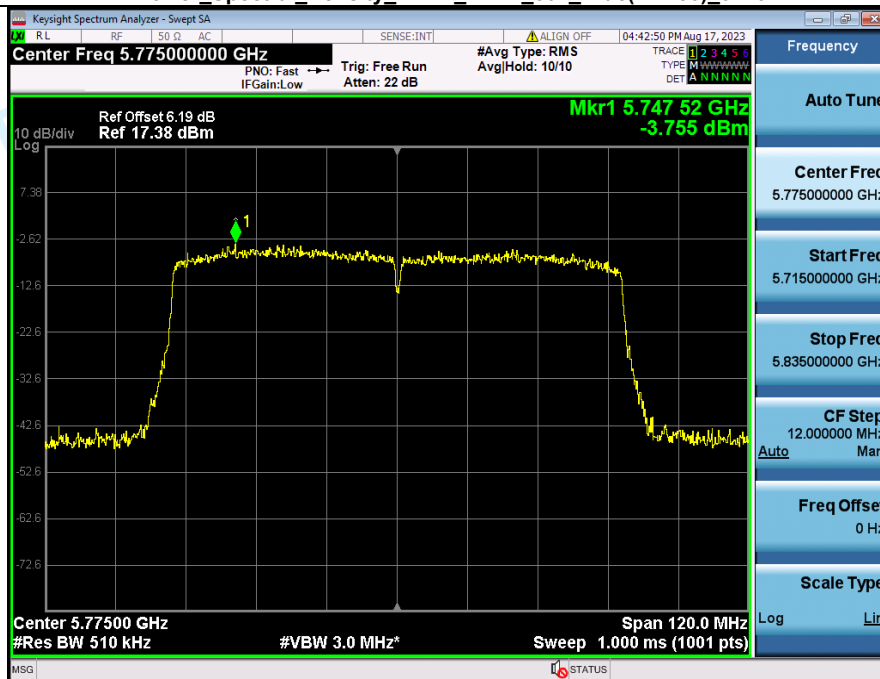
Power Spectral Density NVNT_ANT2_802_11ac(VHT80)_5775
