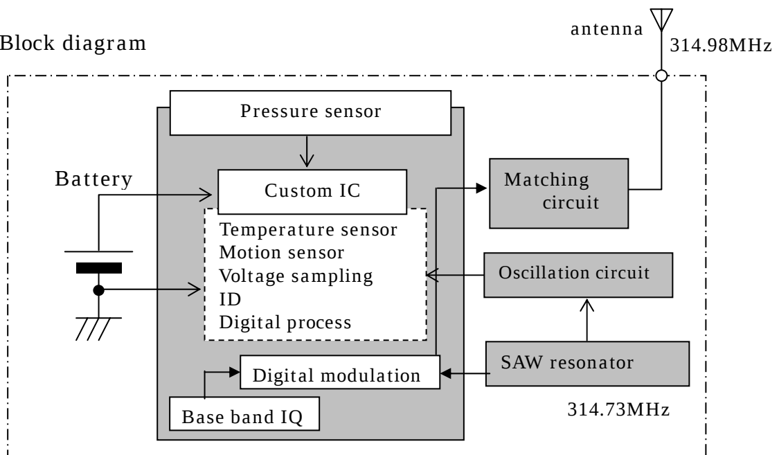
Fig 6, Block diagram of transmitter
