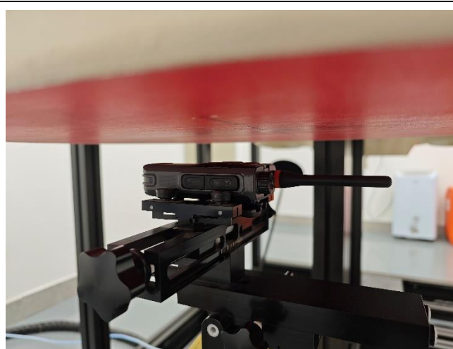
Front-of-face(25mm)
