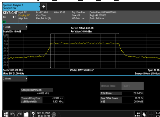
B7_N5(5M)_CP-OFDM_256 QAM_Outer_Full_Mid_CH
