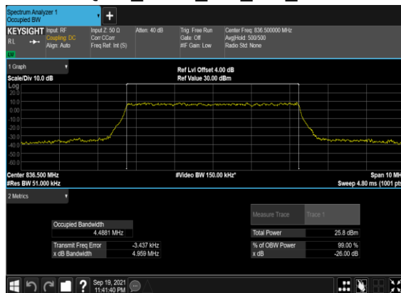
B7_N5(5M)_CP-OFDM_16 QAM_Outer_Full_Mid_CH
