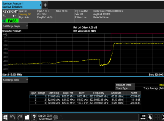
B7_N5(5M)_DFT-s- OFDM_BPSK_Outer_Full_Low_CH
