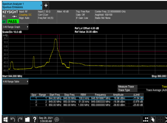
B7_N5(5M)_DFT-s- OFDM_BPSK_Edge_1RB_Right_High_CH
