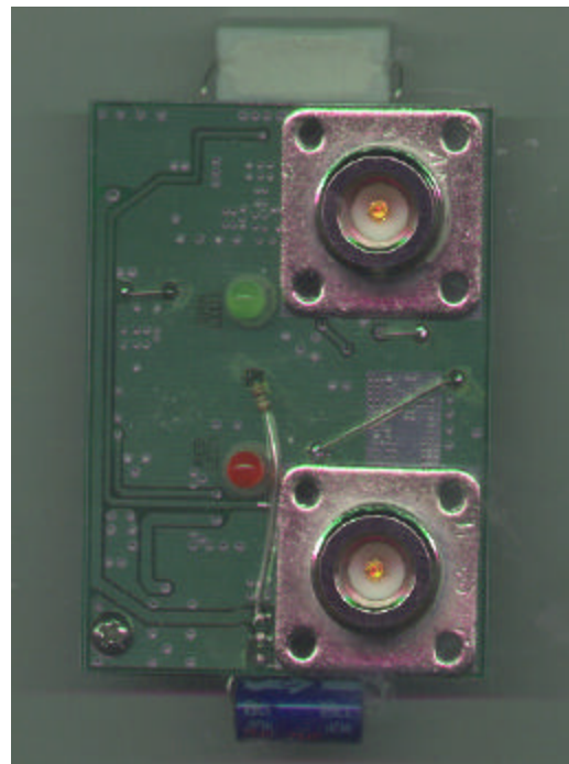
500mW Solder Side
