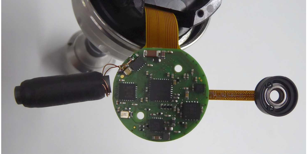
Wöhler VIS 700 - camera head 3
