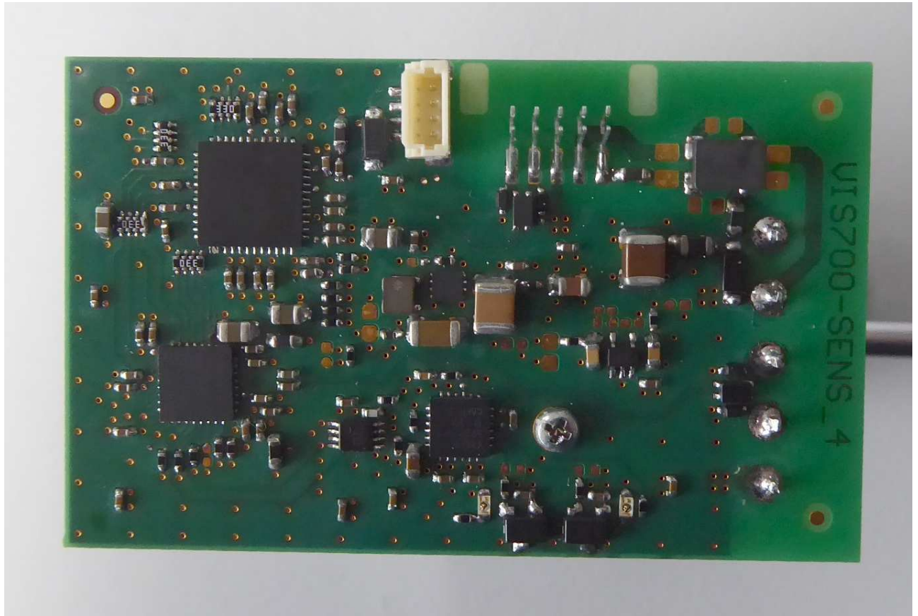
Wöhler VIS 700 - PCB top view
