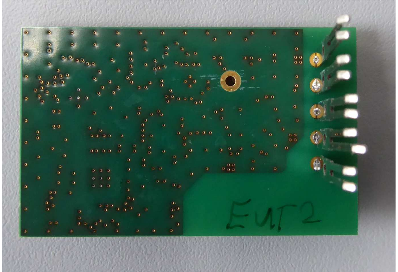
Wöhler VIS 700 - PCB bottom view
