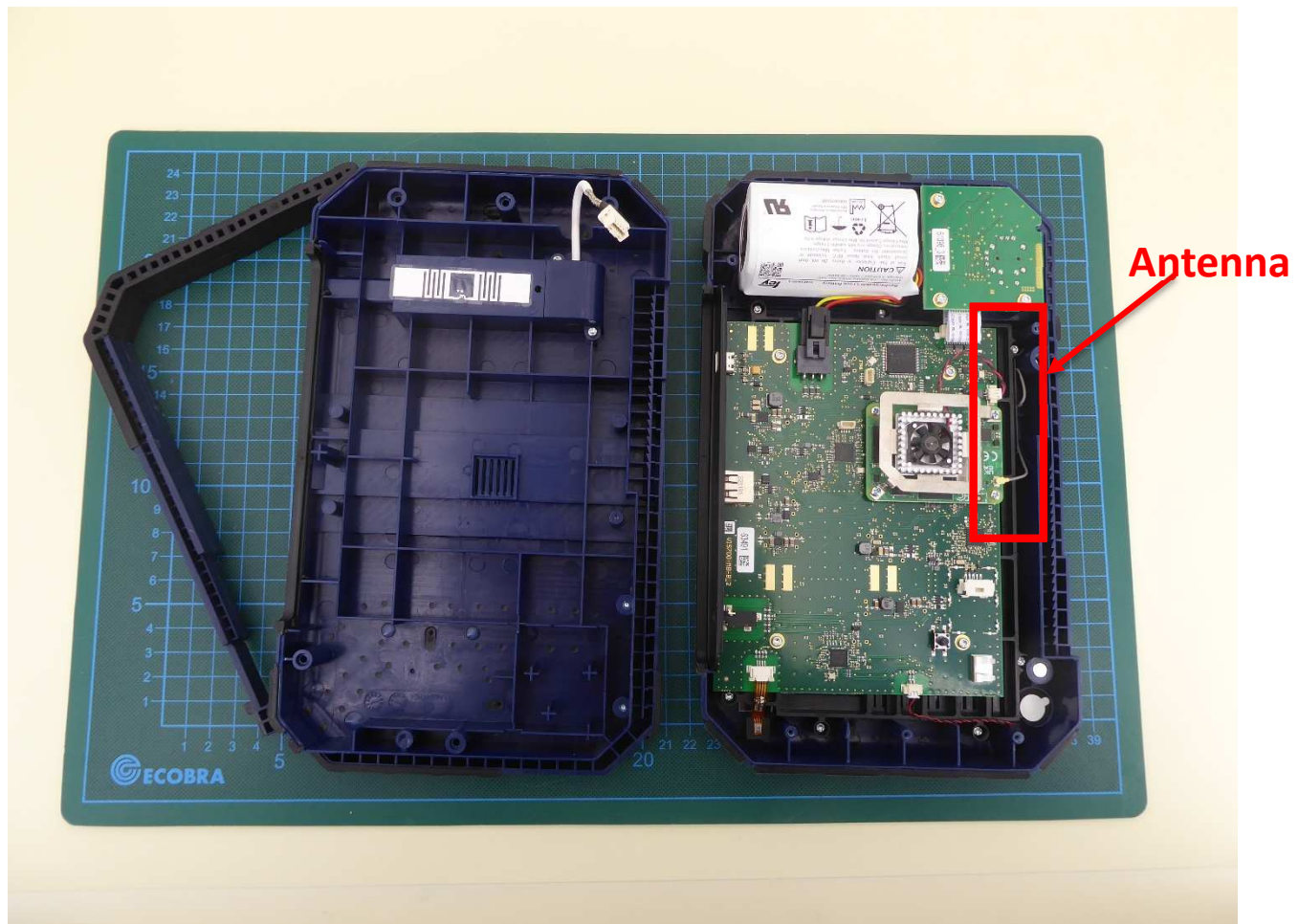
Wöhler VIS 700 – VIS 7 HD (monitor unit) disassembled - 2
