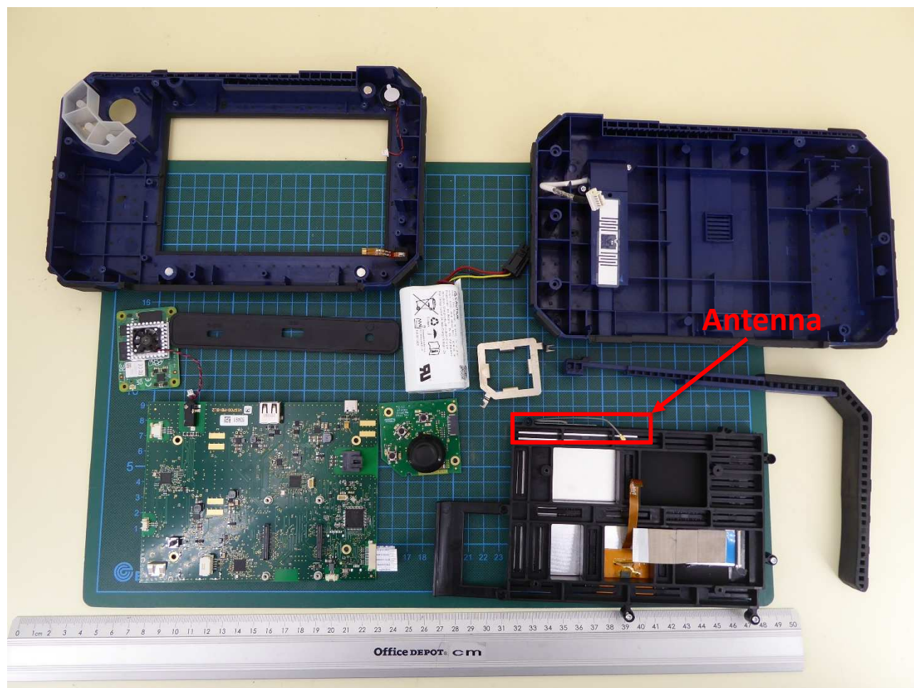
Wöhler VIS 700 – VIS 7 HD (monitor unit) disassembled - 1
