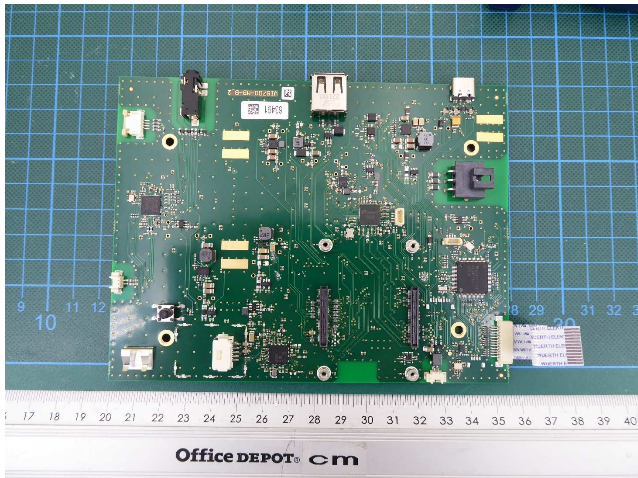
Wöhler VIS 700 – VIS 7 HD (monitor unit): main PCB top view
