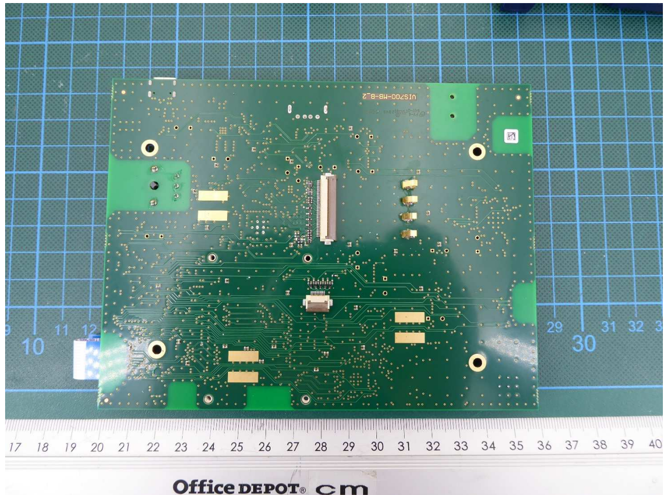
Wöhler VIS 700 – VIS 7 HD (monitor unit): main PCB bottom view
