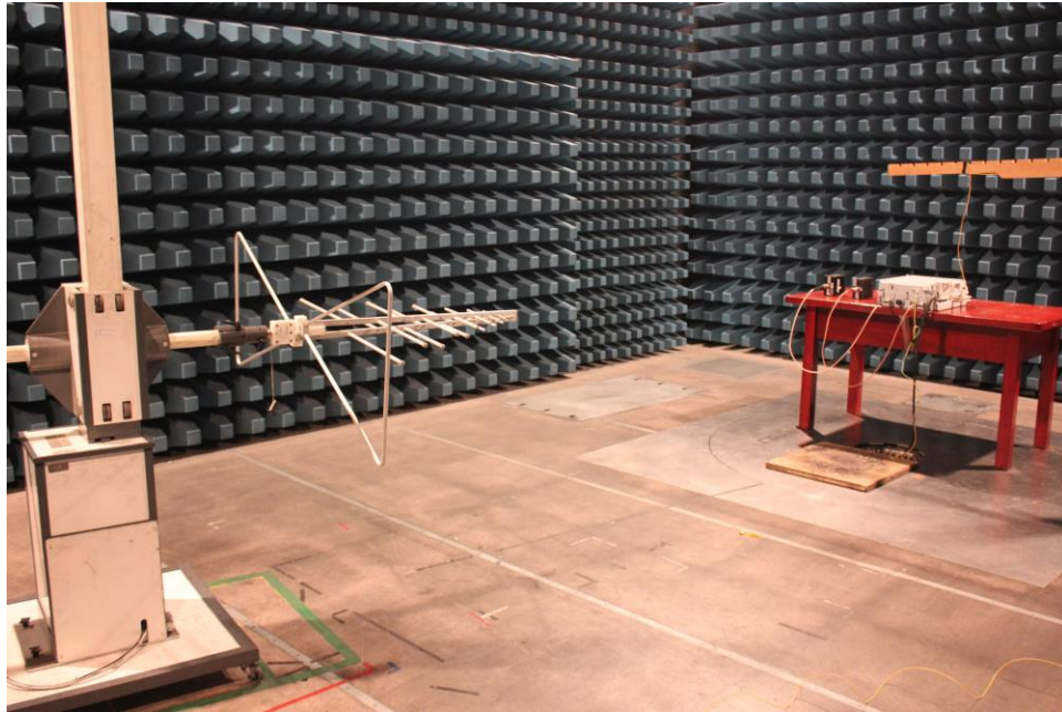
Test setup photos
