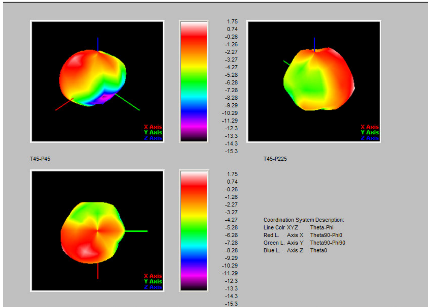
(2) 天线苹果图(Antenna Apple Chart) Passive -Freq2400.00MHZ
