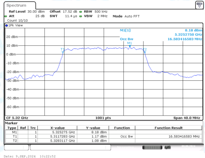
11A-Ant2-5320
