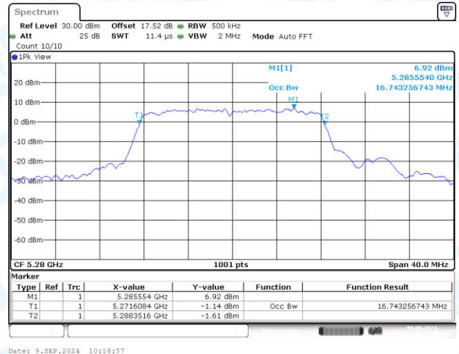
11A-Ant2-5280
