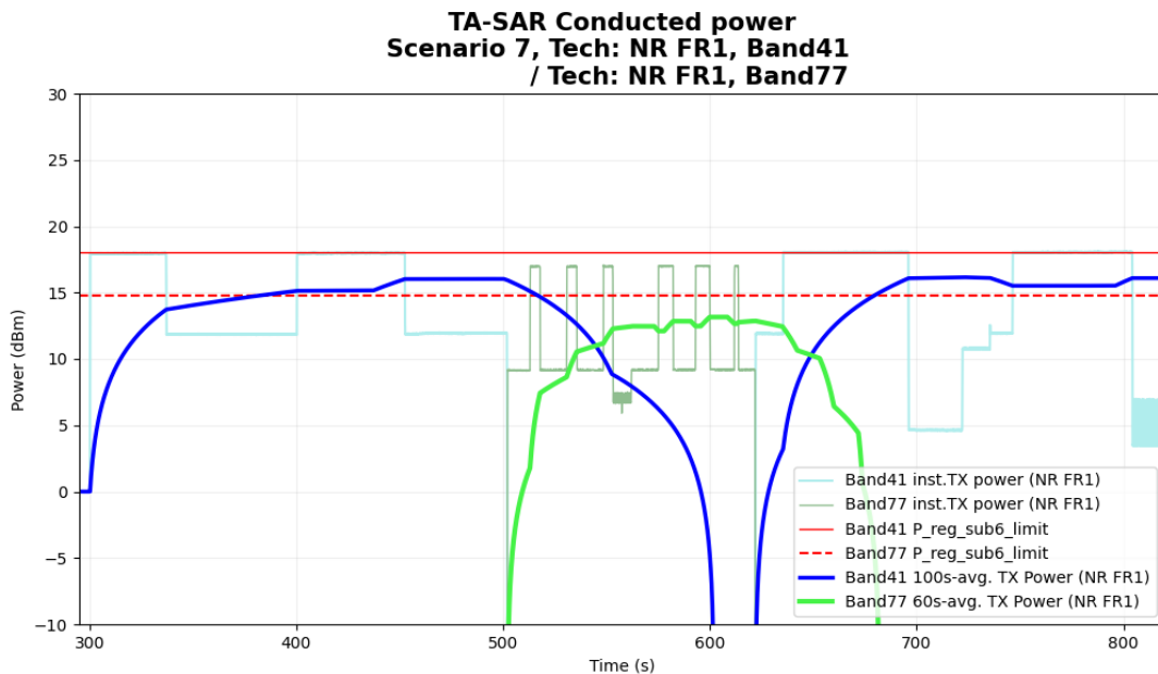
Figure 6- 40 Time-averaged conducted TX power over time
