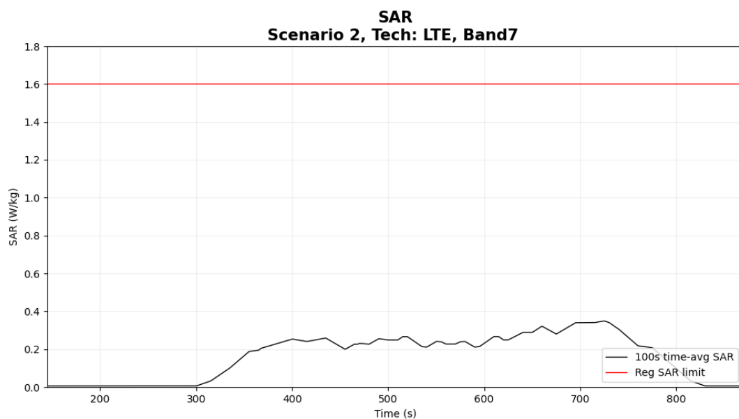
Figure 6- 20 Time-averaged SAR
