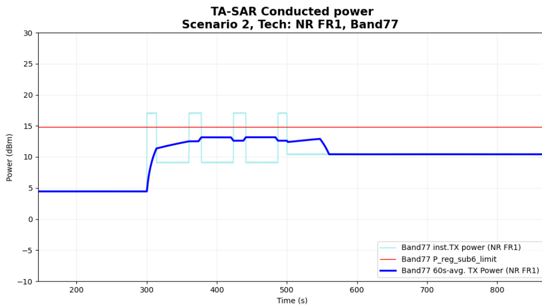
Figure 6- 29 Time-averaged conducted TX power over time
