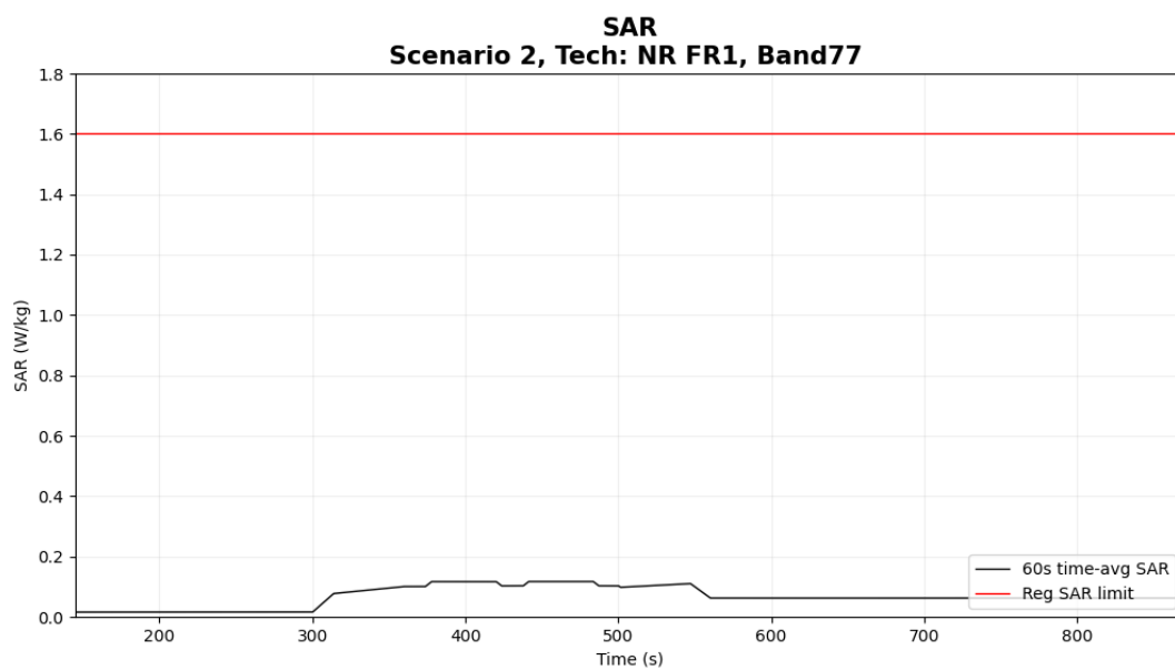
Figure 6- 30 Time-averaged SAR
