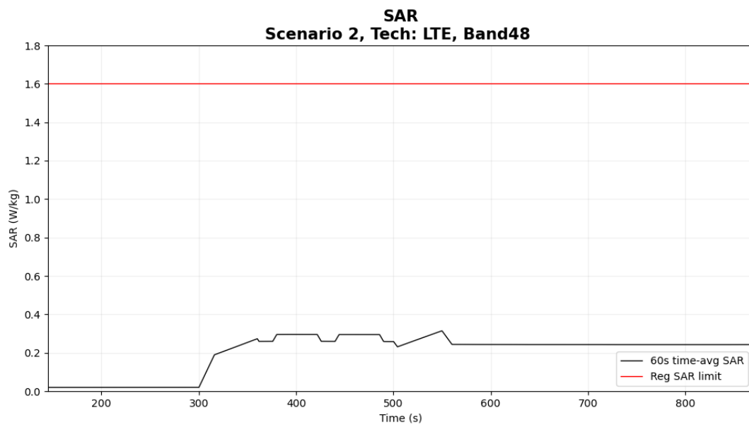
Figure 6- 22 Time-averaged SAR
