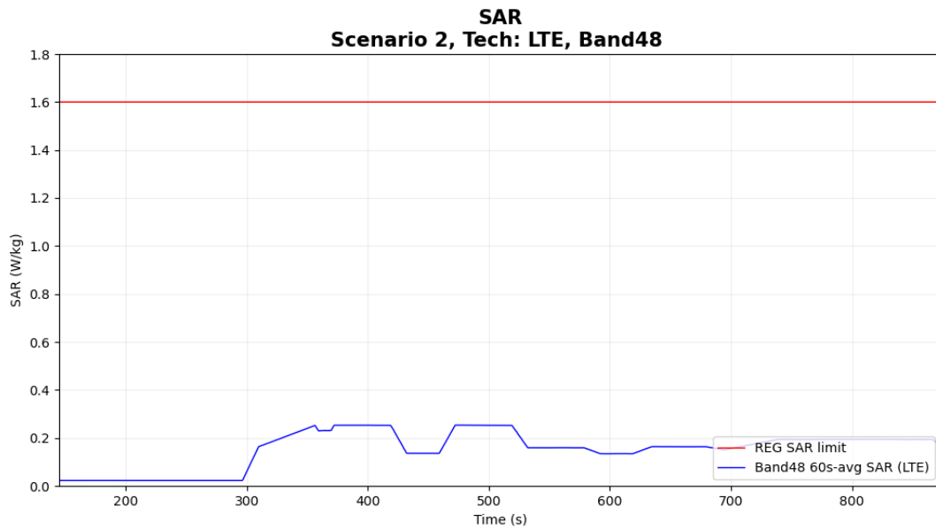
Figure 7-9 Time-averaged SAR
