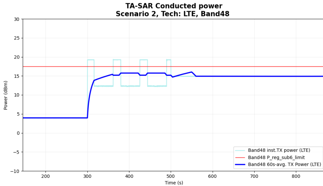
Figure 6- 21 Time-averaged conducted TX power over time
