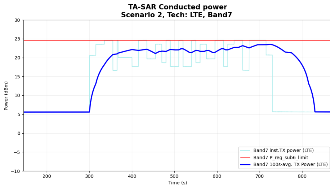
Figure 6- 20 Time-averaged conducted TX power over time
