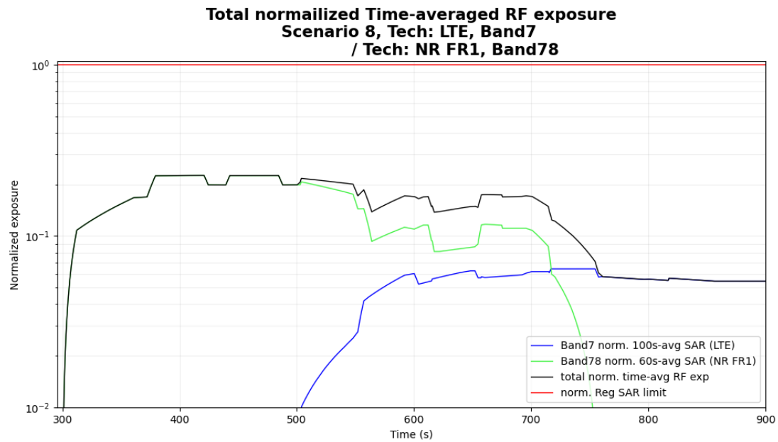
Figure 6- 43 Normalized time-averaged SAR
