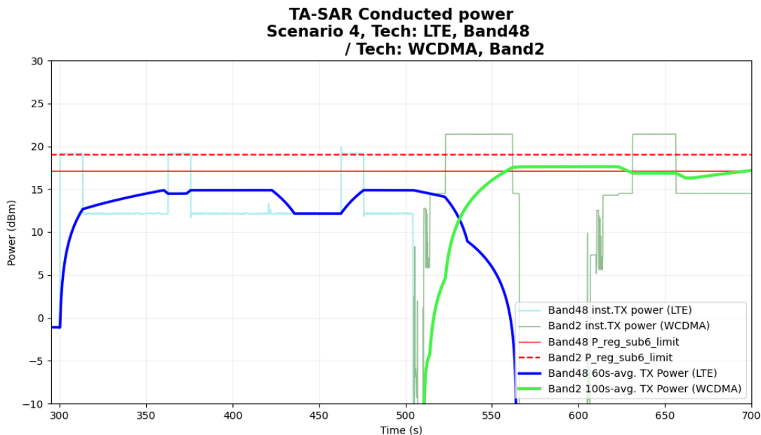
Figure 6- 34 Time-averaged conducted TX power over time
