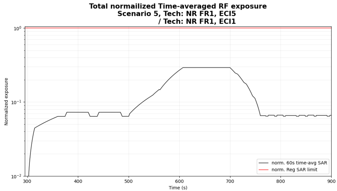
Figure 6- 37 Normalized time-averaged SAR
