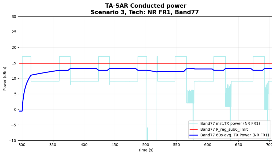
Figure 6- 42 Time-averaged conducted TX power over time
