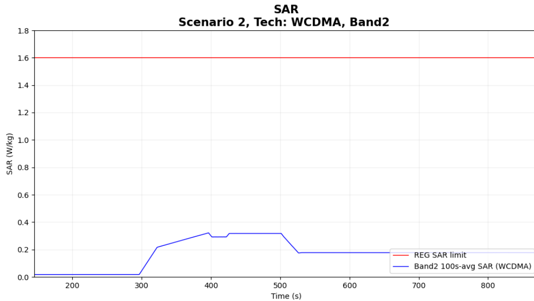
Figure 7-11 Time-averaged SAR
