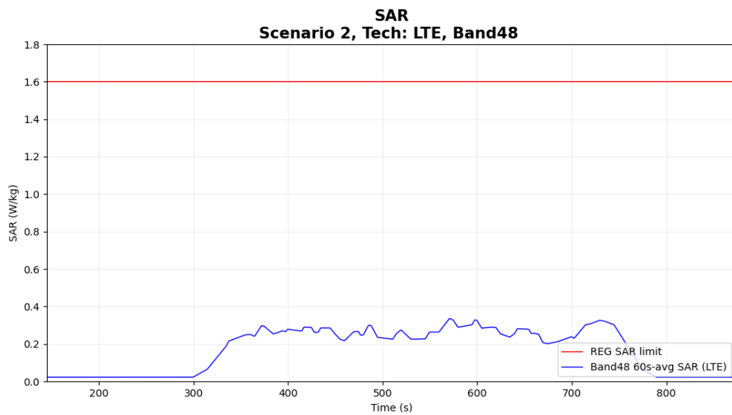
Figure 7-10 Time-averaged SAR
