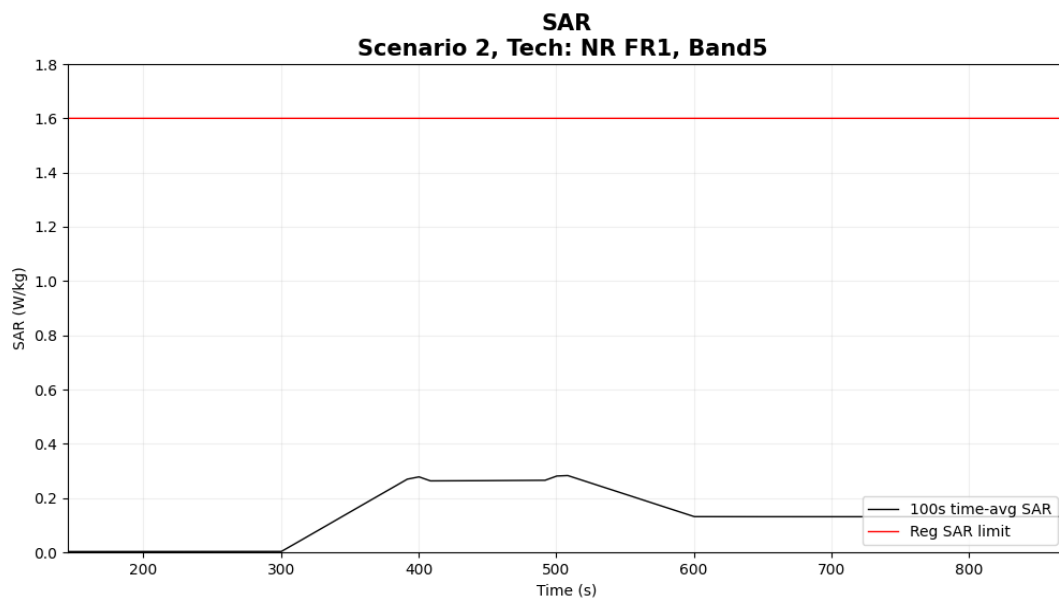
Figure 6- 26 Time-averaged SAR
