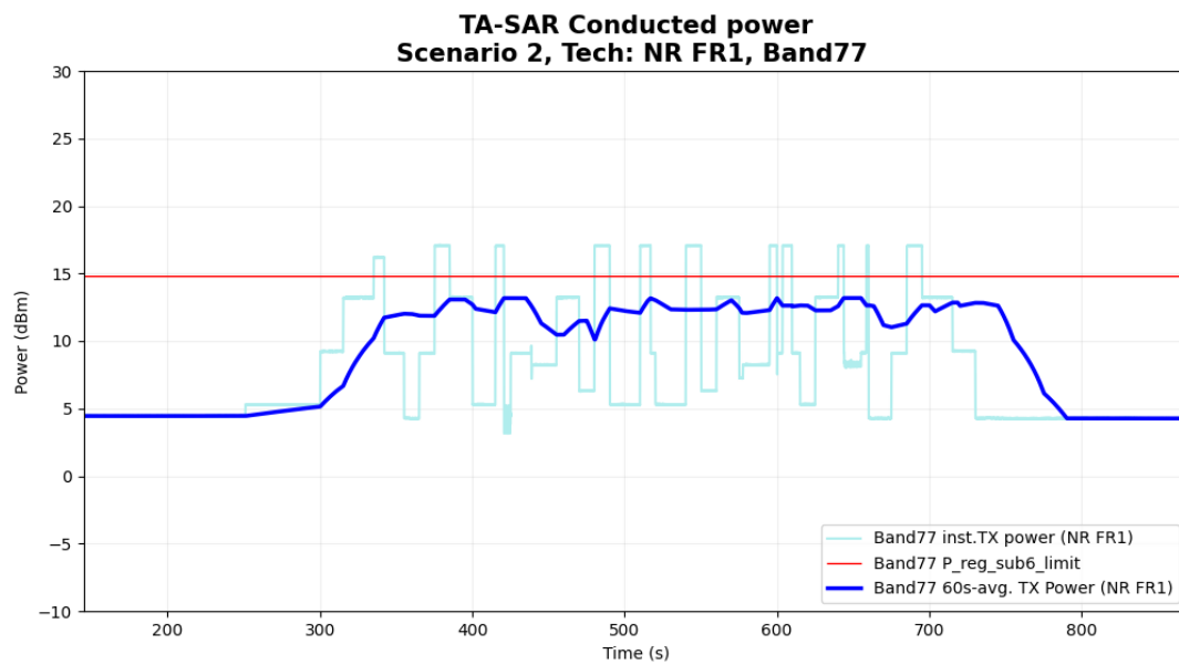
Figure 6- 31 Time-averaged conducted TX power over time
