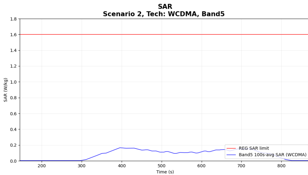
Figure 7-14 Time-averaged SAR
