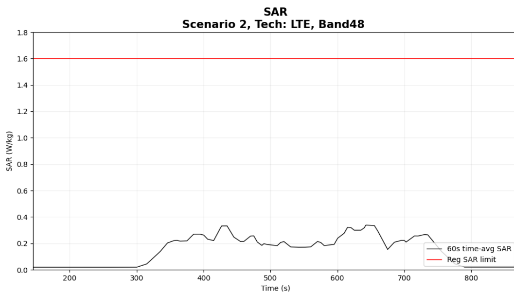
Figure 6- 24 Time-averaged SAR
