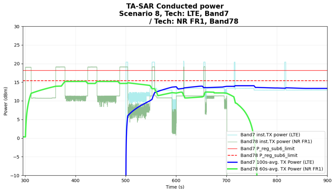
Figure 6- 42 Time-averaged conducted TX power over time
