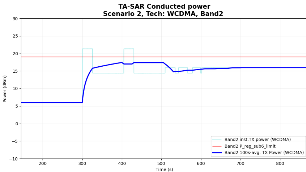
Figure 6- 11 Time-averaged conducted TX power over time
