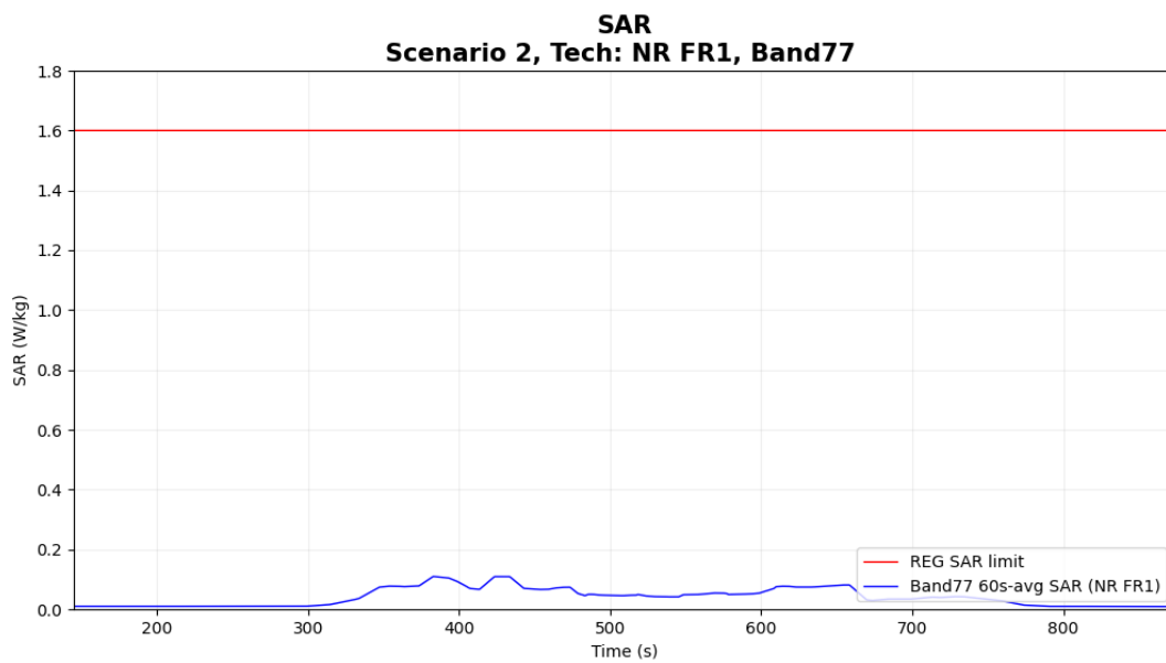
Figure 7-6 Time-averaged SAR for case
