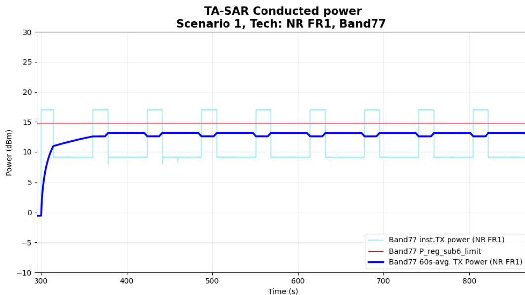
Figure 6- 5 Time-averaged conducted TX power over time
