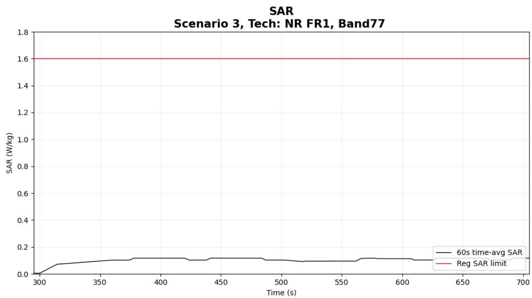
Figure 6- 33 Time-averaged SAR
