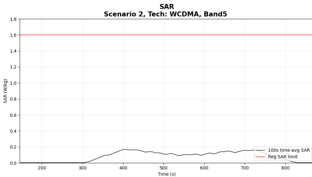
Figure 6- 17 Time-averaged SAR
