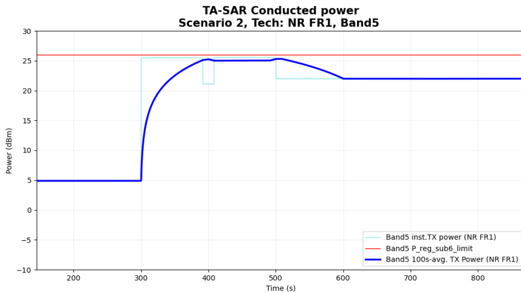
Figure 6- 25 Time-averaged conducted TX power over time
