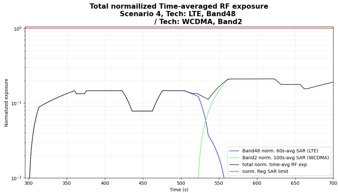
Figure 6- 35 Normalized time-averaged SAR
