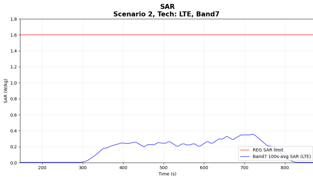
Figure 7-8 Time-averaged SAR
