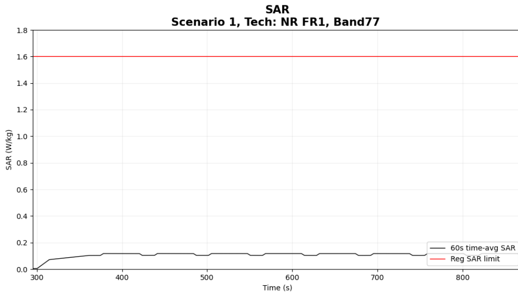
Figure 6- 6 Time-averaged SAR
