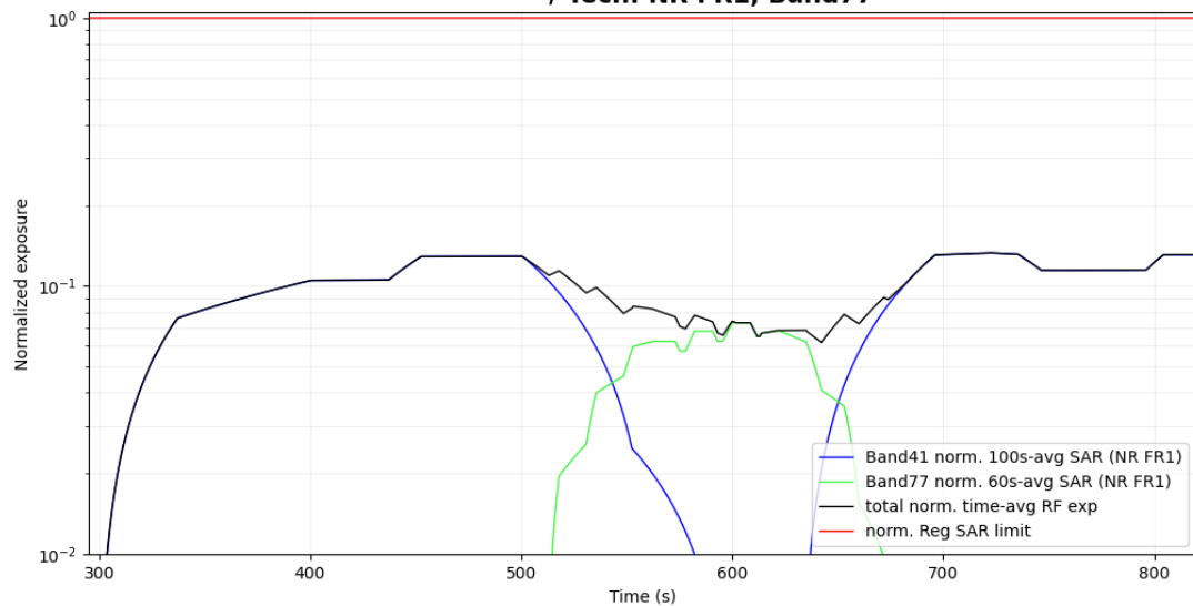
Figure 6- 41 Normalized time-averaged SAR
