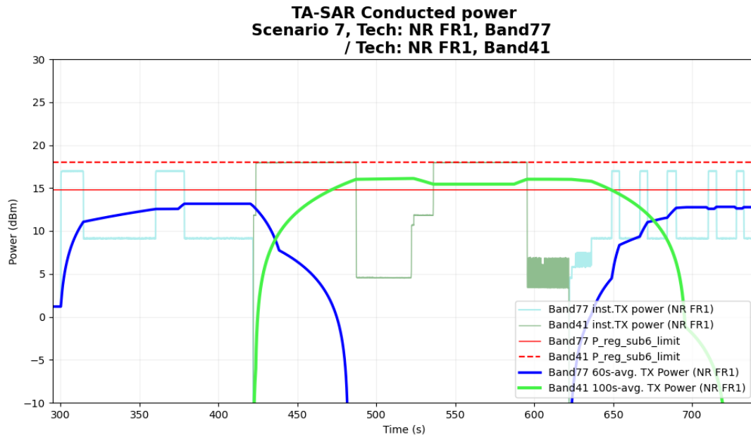
Figure 6- 38 Time-averaged conducted TX power over time
