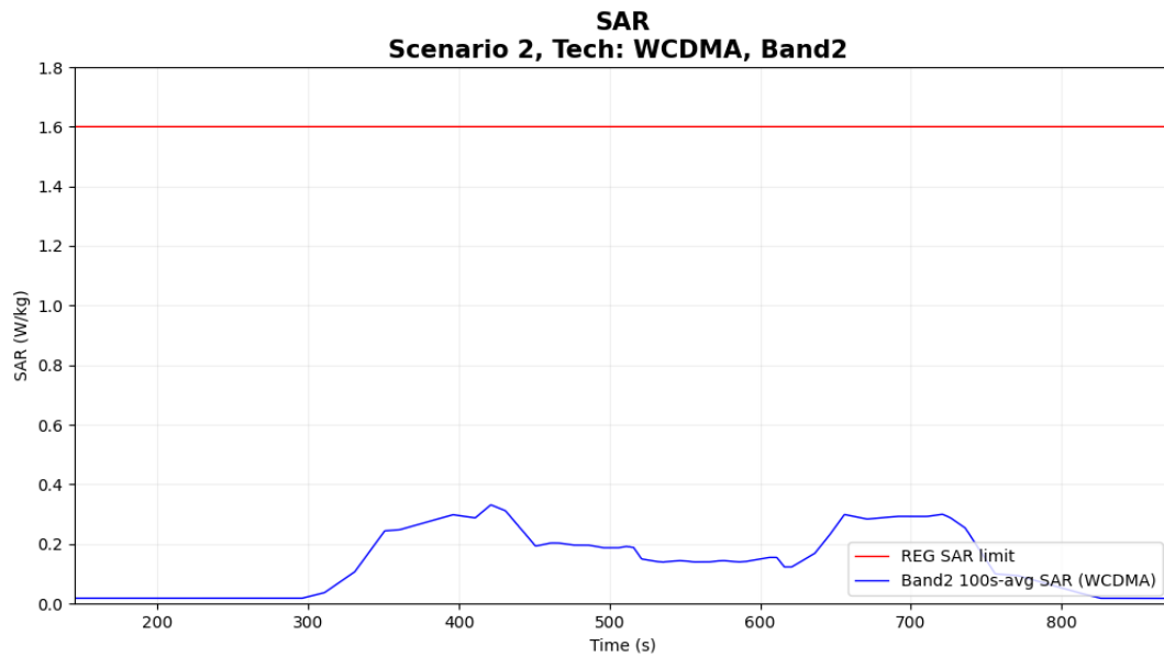
Figure 7-12 Time-averaged SAR
