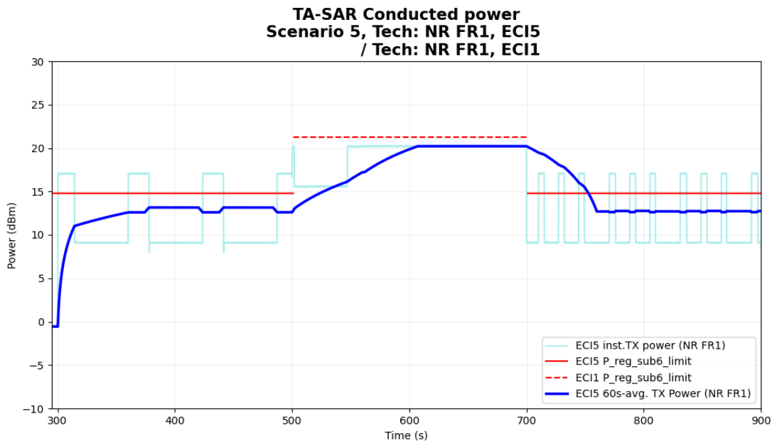
Figure 6- 36 Time-averaged conducted TX power over time
