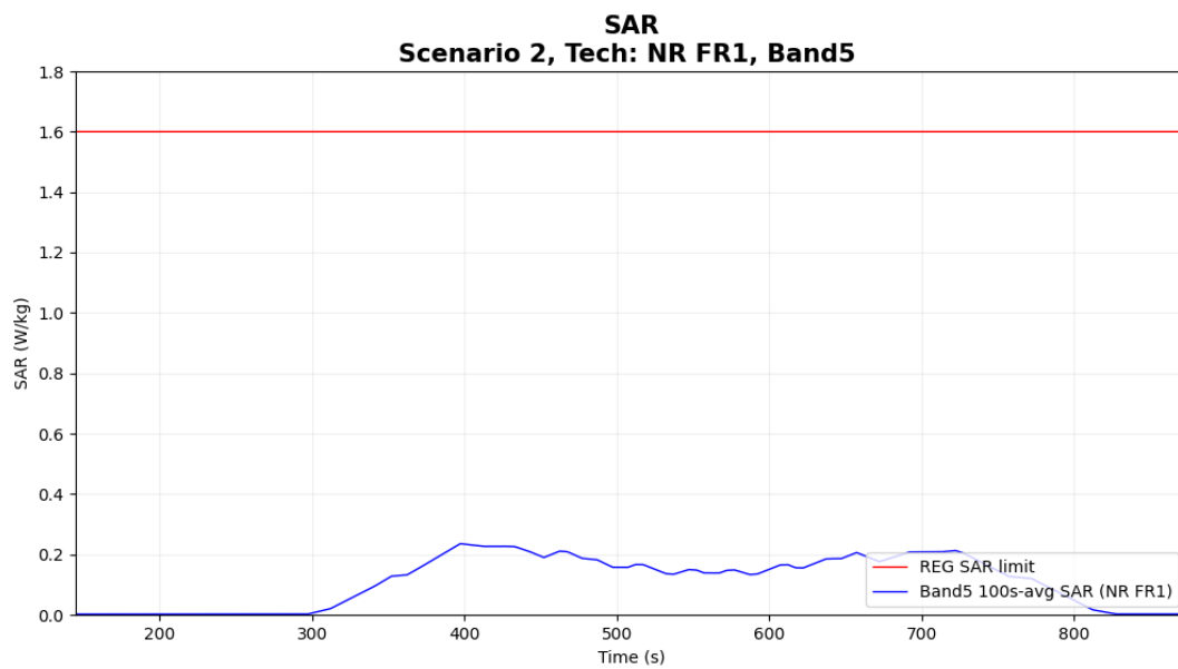
Figure 7-4 Time-averaged SAR
