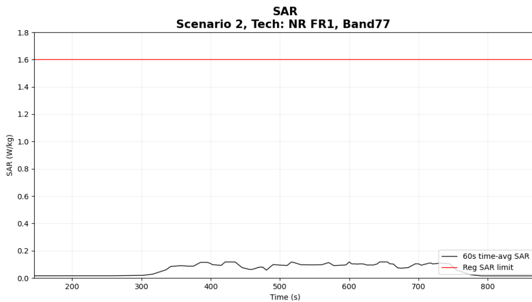
Figure 6- 32 Time-averaged SAR
