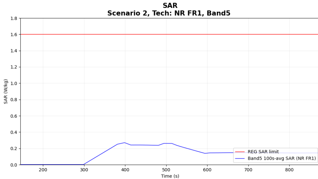
Figure 7-3 Time-averaged SAR
