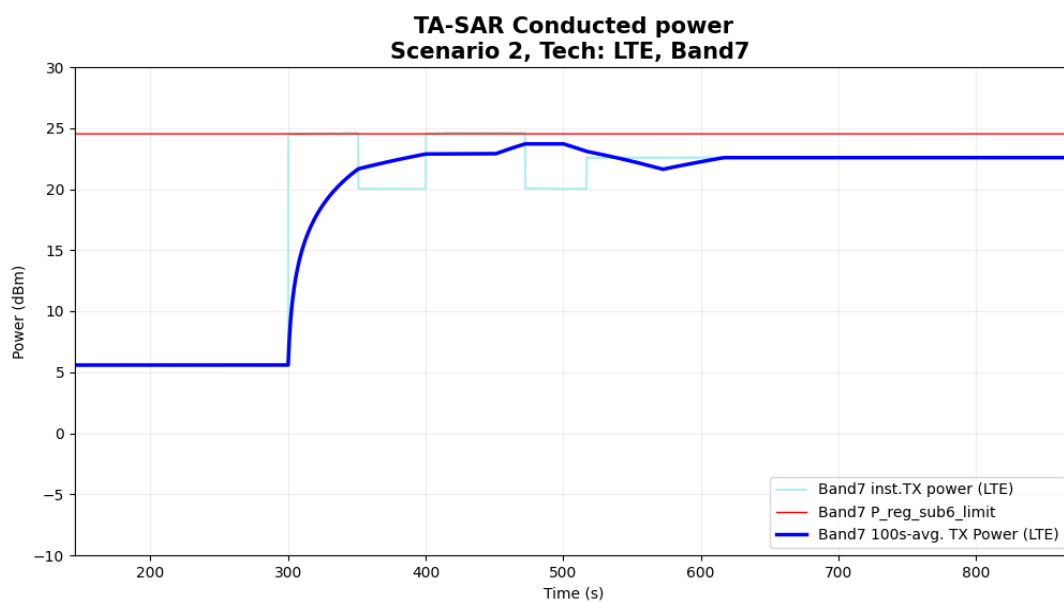
Figure 6- 18 Time-averaged conducted TX power over time
