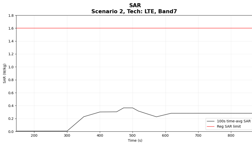
Figure 6- 19 Time-averaged SAR
