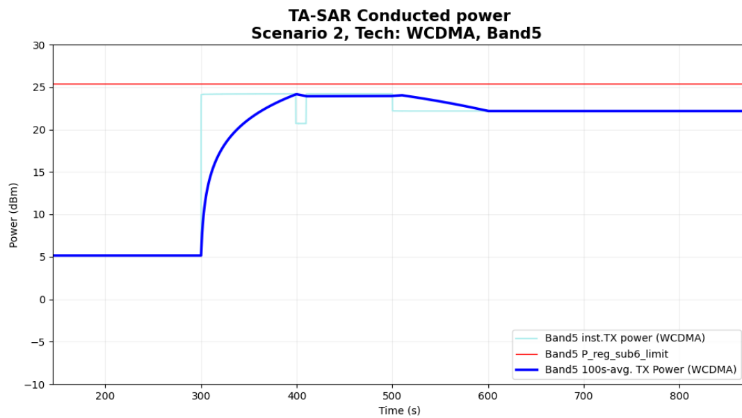
Figure 6- 14 Time-averaged conducted TX power over time
