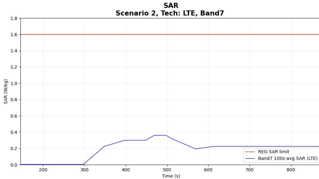
Figure 7-7 Time-averaged SAR
