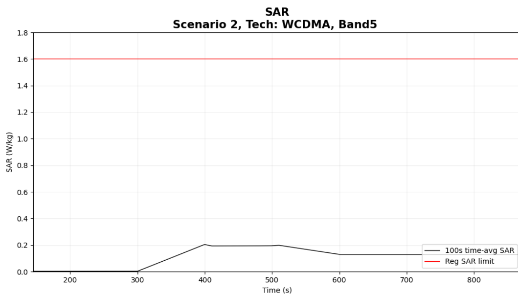
Figure 6- 15 Time-averaged SAR
