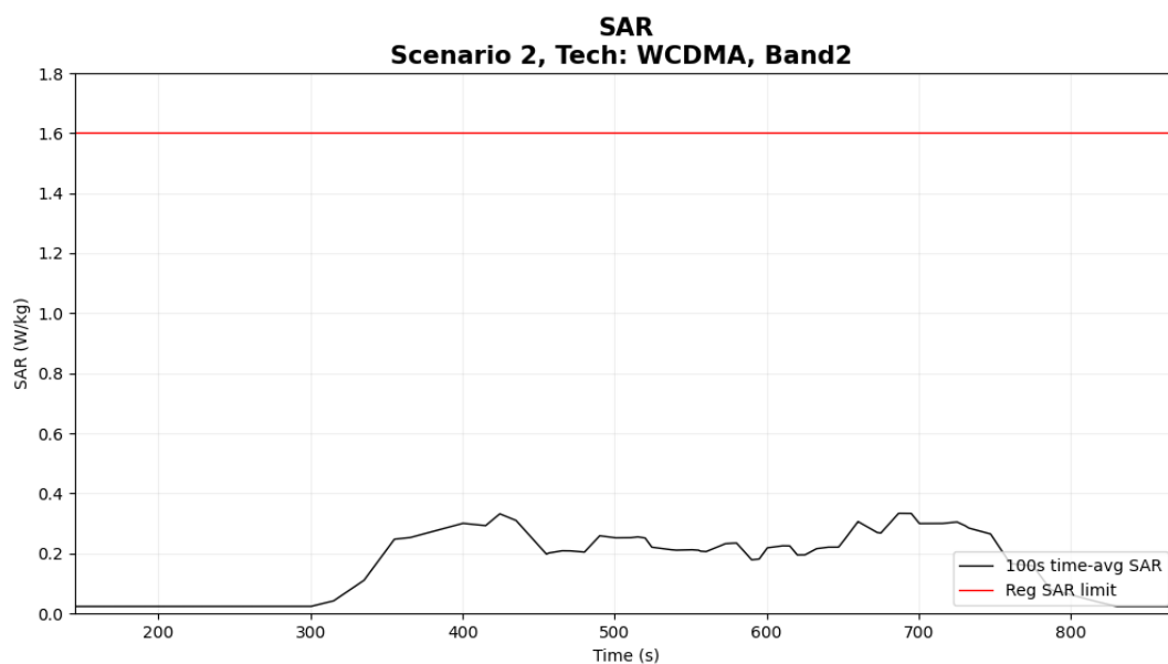
Figure 6- 13 Time-averaged SAR
