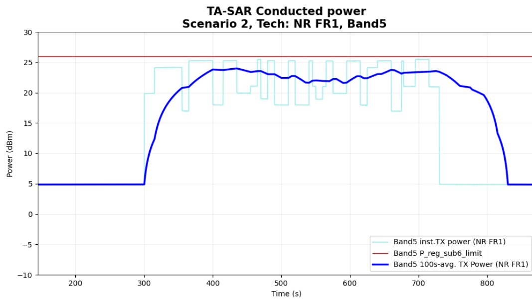
Figure 6- 27 Time-averaged conducted TX power over time
