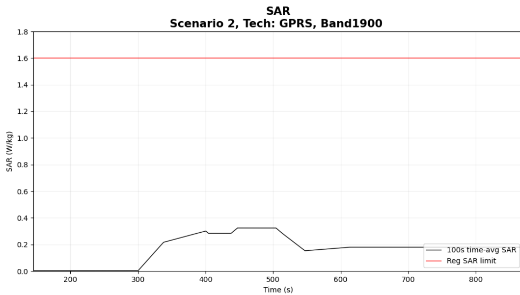
Figure 6- 8 Time-averaged SAR
