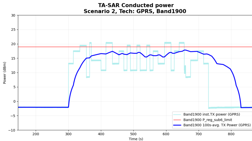
Figure 6- 9 Time-averaged conducted TX power over time
