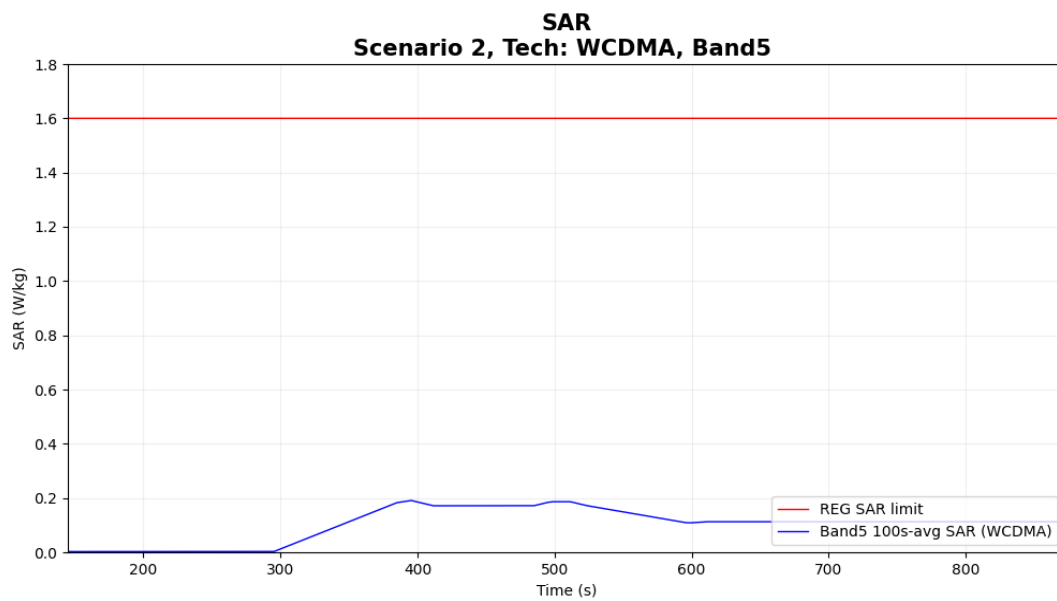
Figure 7-13 Time-averaged SAR
