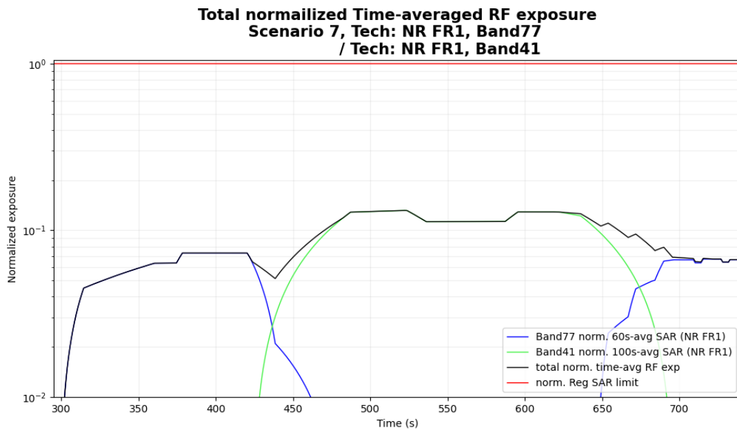
Figure 6- 39 Normalized time-averaged SAR
