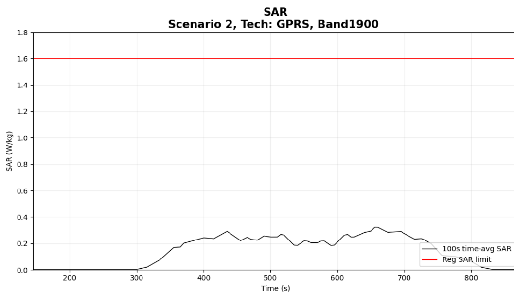
Figure 6- 10 Time-averaged SAR
