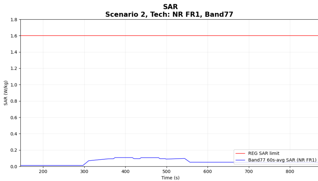
Figure 7-5 Time-averaged SAR
