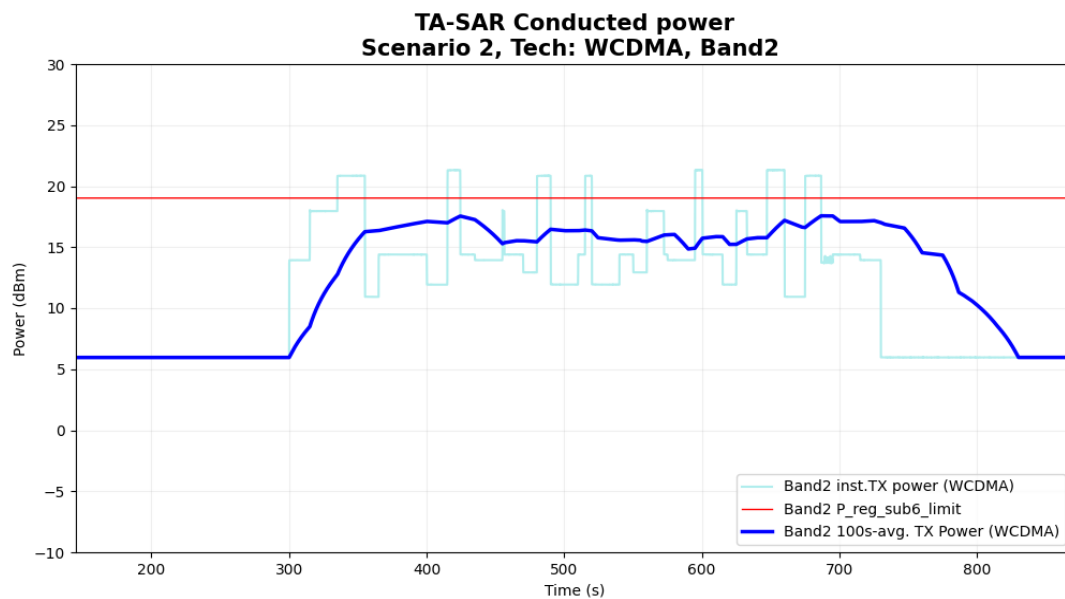
Figure 6- 28 Time-averaged conducted TX power over time
