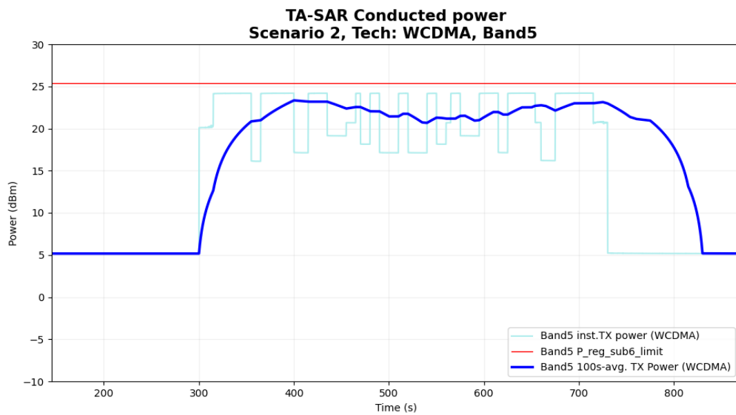
Figure 6- 16 Time-averaged conducted TX power over time
