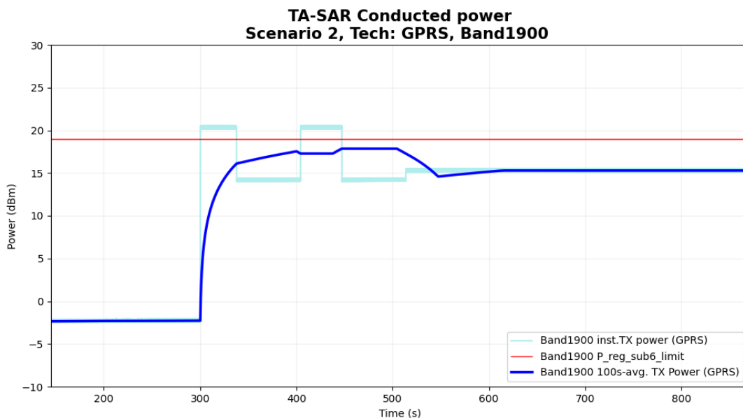
Figure 6- 7 Time-averaged conducted TX power over time
