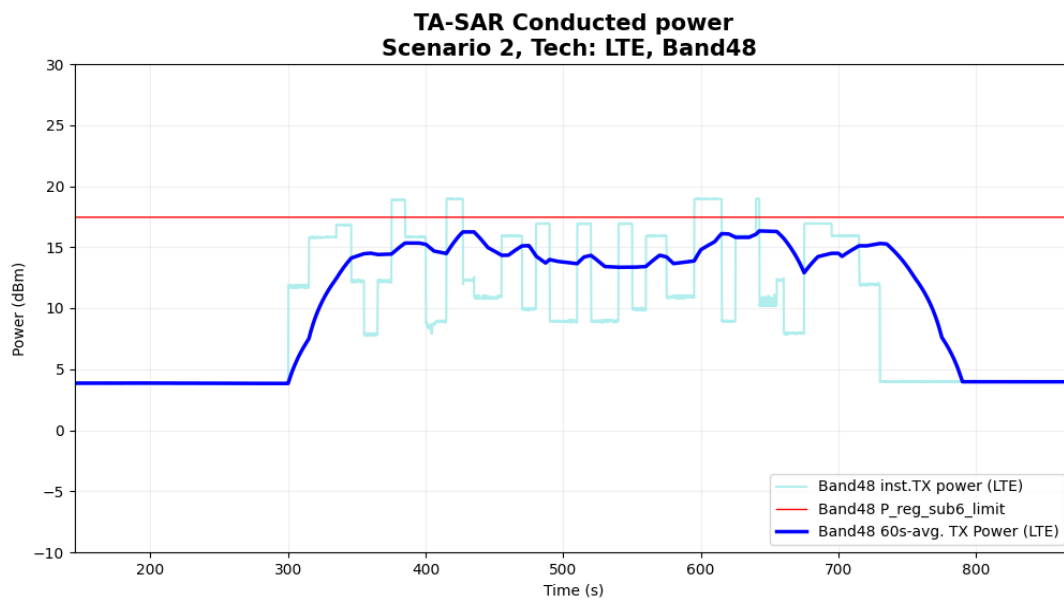
Figure 6- 23 Time-averaged conducted TX power over time
