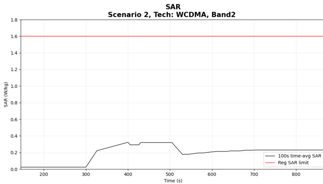
figure 6- 12 Time-averaged SAR
