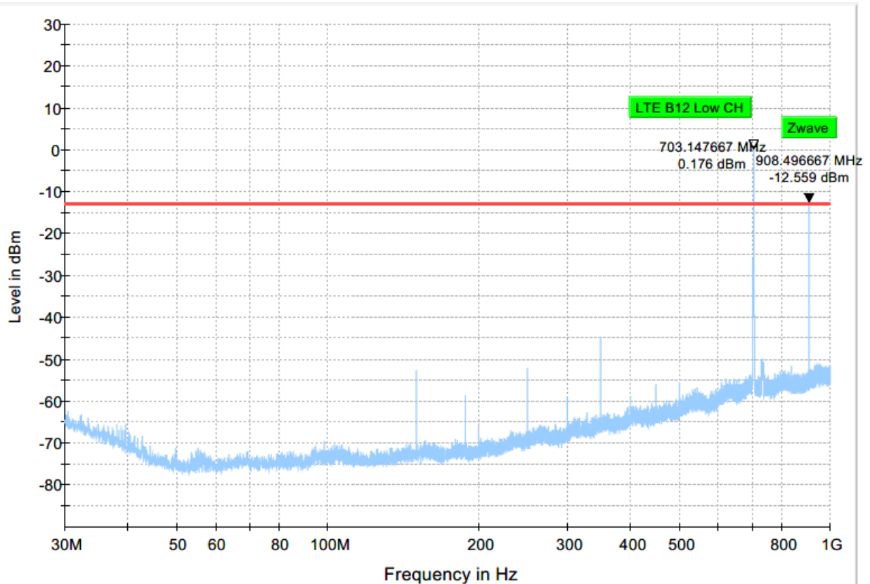
Plot #32 Radiated Emissions: 30 MHz – 1GHz
