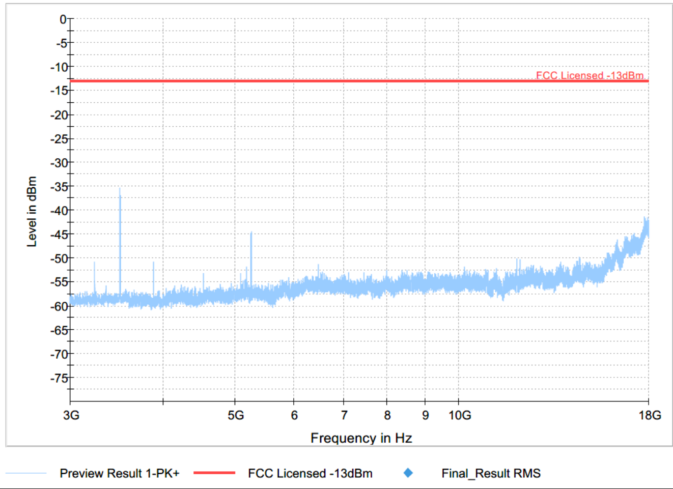
Plot #62 Radiated Emissions: 3-18 GHz
