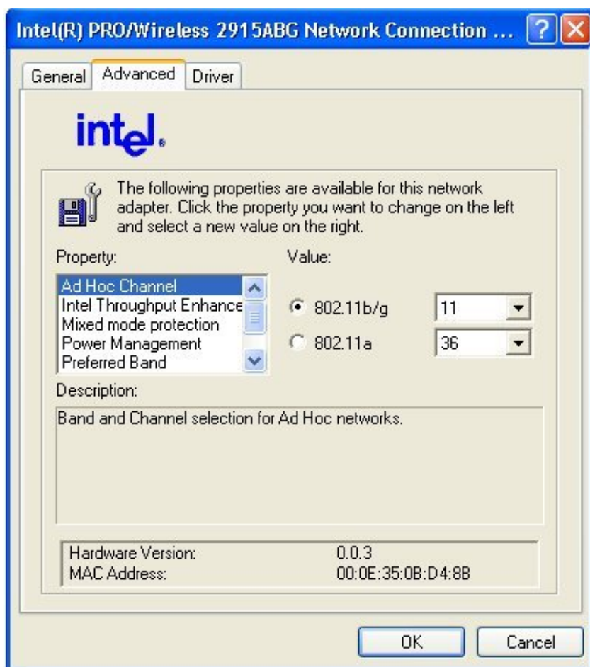
Adapter Settings displays the Device Properties for the Intel® PRO/Wireless 2915ABG Network Connection.
