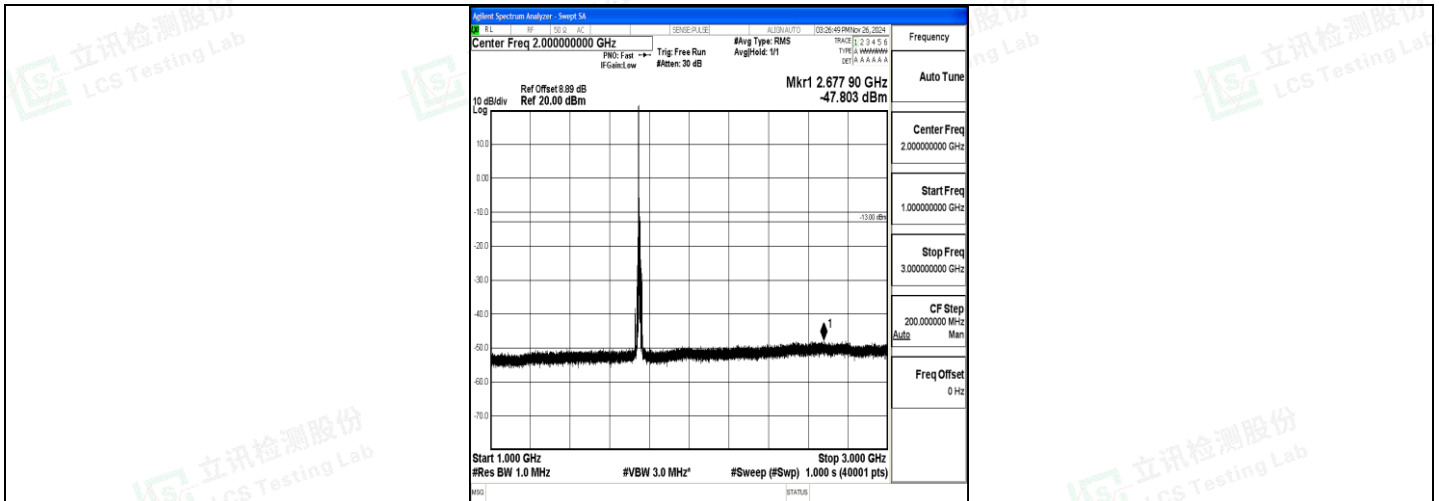
Band4_10MHz_16QAM_20350_1RB#0_1000~3000_1000~3000
