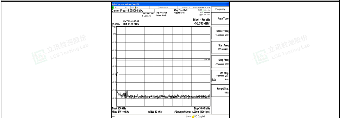
Band4_15MHz_16QAM_20025_1RB#0_0.15~30_0.15~30
