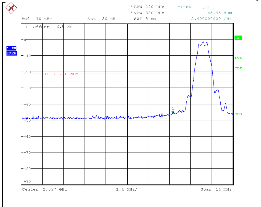
Bandedge
