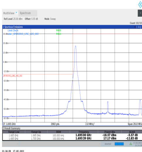
1-N70-15-10-L-4-CP-QPSK-Edge_1RB_Left-1@0-Ant1-seegraph-PASS-see graph
