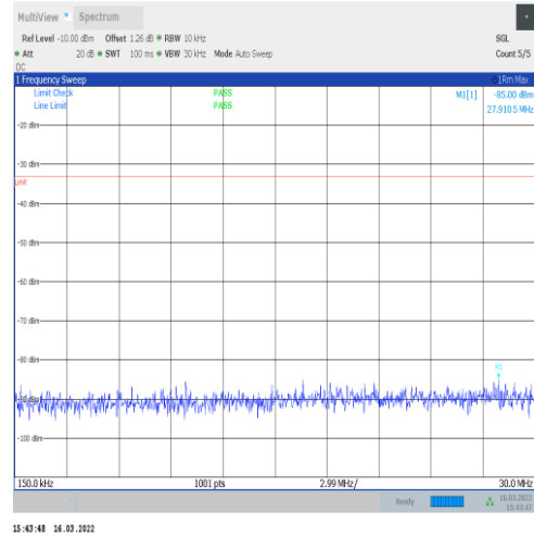
1-N70-15-15-M-1-DFT-PI2BPSK-Inner_1RB_Left-1 @1-0.15-30-Ant1--85.00--33-PASS
