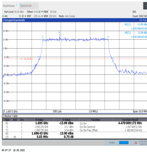
1-N70-15-5-L-1-DFT-QPSK-Outer_Full-25@0-Ant1-4 4.79-5.030-≤5-PASS
