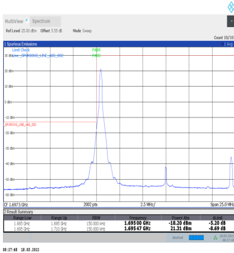
1-N70-15-15-M-1-DFT-PI2BPSK-Edge_1RB_Left-1@0-Ant1-seegraph-PASS-see graph
