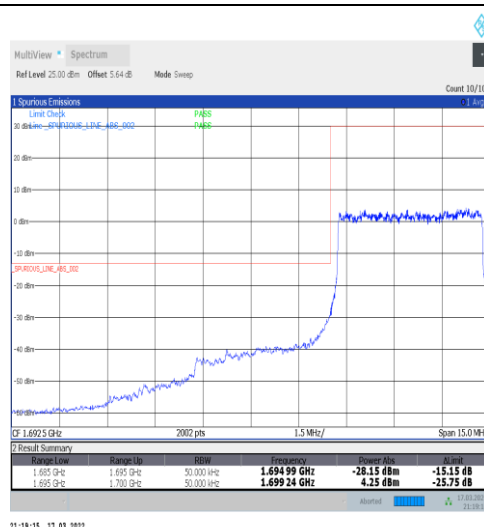
1-N70-15-5-L-3-DFT-PI2BPSK-Outer_Full-25@0-Ant1-seegraph-PASS-see graph
