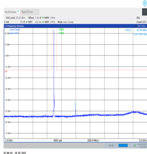
1-N70-15-15-M-1-DFT-PI2BPSK-Inner_1RB_Left-1 @1-1000-3000-Ant1--47.09--13-PASS
