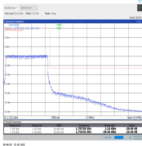
1-N70-15-5-H-6-CP-QPSK-Outer_Full-25@0-Ant1-seegraph-PASS-see graph
