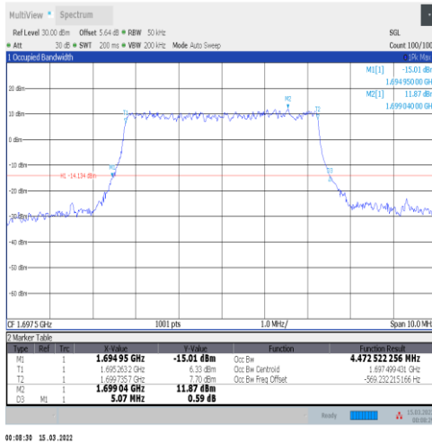
1-N70-15-5-L-3-DFT-16QAM-Outer_Full-25@0-Ant1- 4.473-5.070-≤5-PASS
