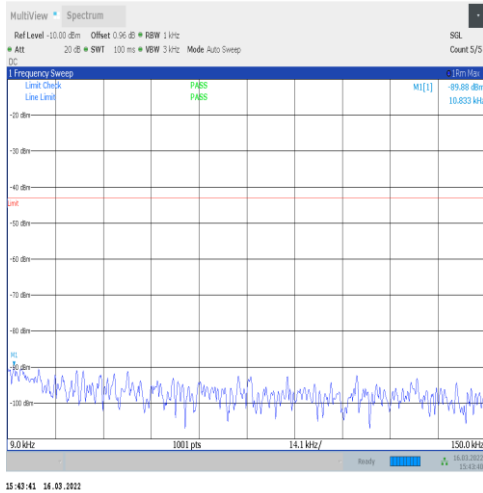
1-N70-15-15-M-1-DFT-PI2BPSK-Inner_1RB_Left-1@ 1-0.009-0.15-Ant1--89.88--43-PASS
