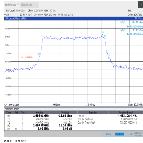
1-N70-15-5-L-4-DFT-64QAM-Outer_Full-25@0-Ant1 -4.483-5.020-≤5-PASS
