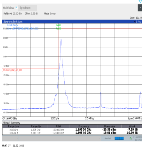
1-N70-15-15-M-4-CP-QPSK-Edge_1RB_Left-1@0-Ant1-seegraph-PASS-see graph
