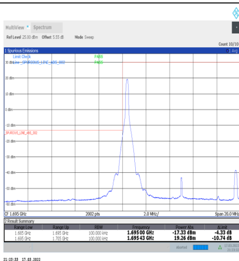
1-N70-15-10-L-1-DFT-PI2BPSK-Edge_1RB_Left-1@0-Ant1-seegraph-PASS-see graph
