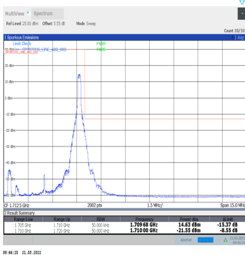
1-N70-15-5-H-5-CP-QPSK-Edge_1RB_Right-1@24-Ant1-seegraph-PASS-see graph
