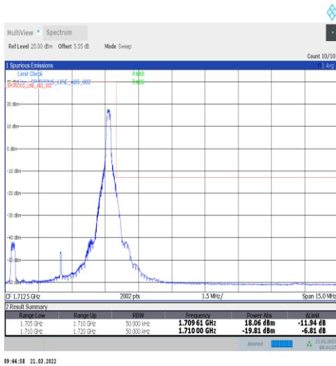
1-N70-15-5-H-2-DFT-PI2BPSK-Edge_1RB_Right-1@24-Ant1-seegraph-PASS-see graph
