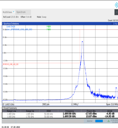
1-N70-15-5-L-4-CP-QPSK-Edge_1RB_Left-1@0-Ant1-seegraph-PASS-see graph
