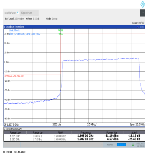
1-N70-15-15-M-3-DFT-PI2BPSK-Outer_Full-75@0-Ant1-seegraph-PASS-see graph
