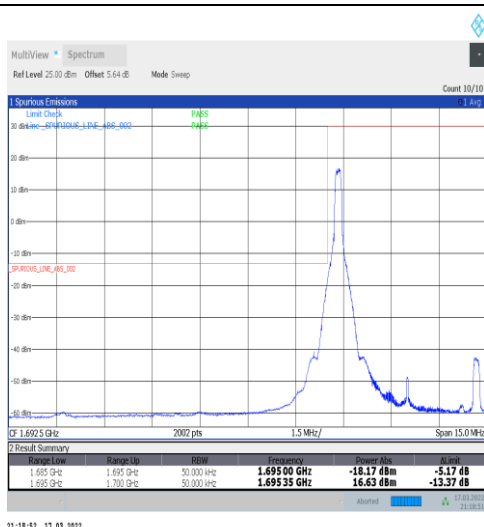
1-N70-15-5-L-1-DFT-PI2BPSK-Edge_1RB_Left-1@0-Ant1-seegraph-PASS-see graph
