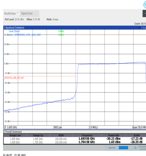
1-N70-15-10-L-6-CP-QPSK-Outer_Full-52@0-Ant1-seegraph-PASS-see graph
