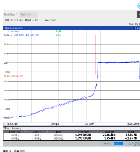
1-N70-15-5-L-6-CP-QPSK-Outer_Full-25@0-Ant1-seegraph-PASS-see graph
