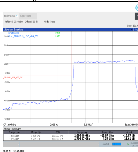
1-N70-15-10-L-3-DFT-PI2BPSK-Outer_Full-50@0-Ant1-seegraph-PASS-see graph
