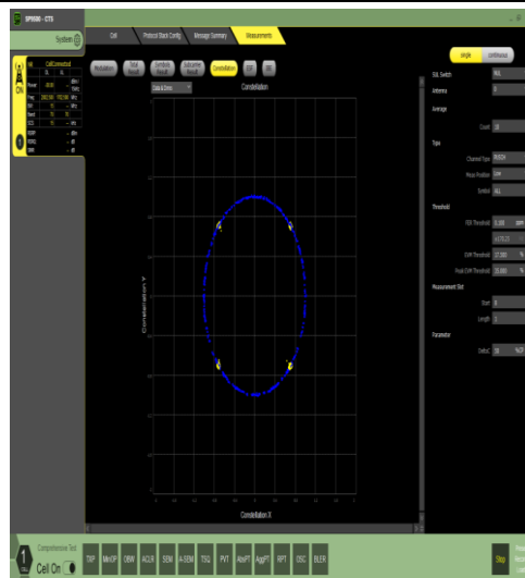
1-N70-15-15-M-2-DFT-QPSK-Outer_Full-75@0-Ant 1-see graph-PASS
