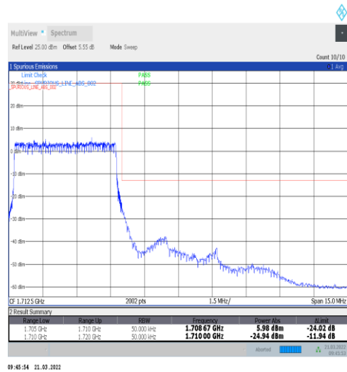
1-N70-15-5-H-3-DFT-PI2BPSK-Outer_Full-25@0-Ant1-seegraph-PASS-see graph
