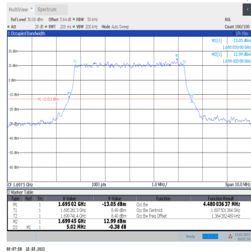
1-N70-15-5-L-2-DFT-PI2BPSK-Outer_Full-25@0-An t1-4.48-5.020-≤5-PASS
