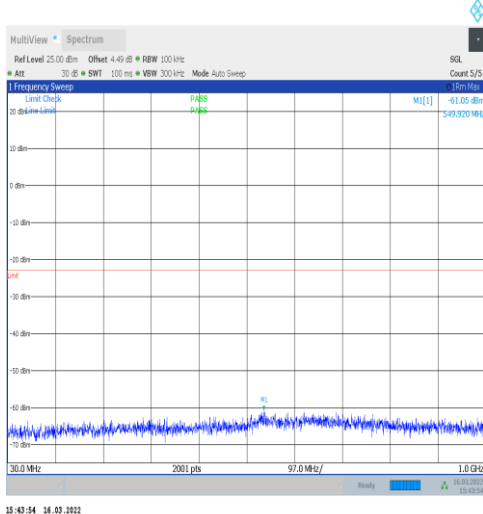
1-N70-15-15-M-1-DFT-PI2BPSK-Inner_1RB_Left-1@ 1-30-1000-Ant1--61.05--23-PASS
