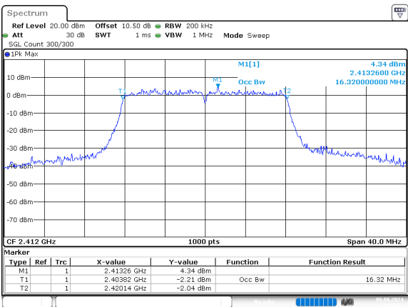
g_2412MHz
