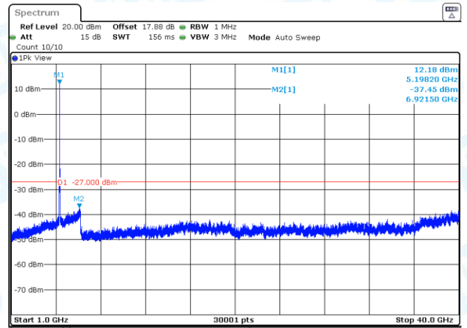
11N20SISO-Ant2-5180-1000~40000-PASS
