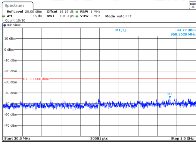
11N20SISO-Ant2-5745-30~1000-PASS
