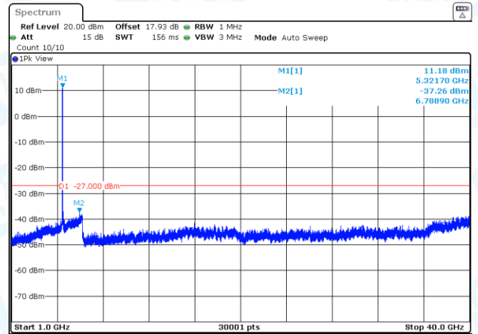
11N20SISO-Ant2-5280-1000~40000-PASS
