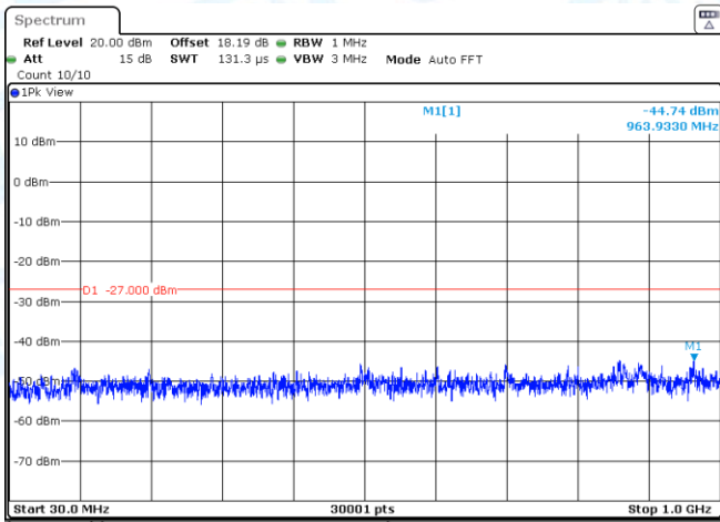
11A-Ant2-5745-30~1000-PASS
