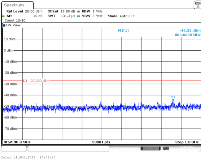
11A-Ant2-5200-30~1000-PASS
