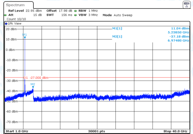
11AC20SISO-Ant2-5200-1000~40000-PASS
