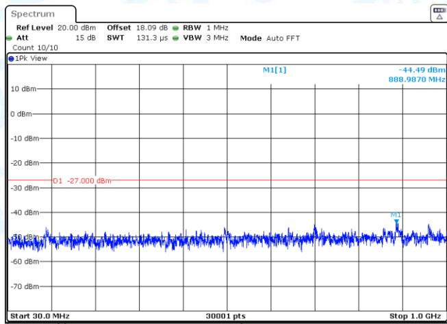
11N20SISO-Ant2-5500-30~1000-PASS
