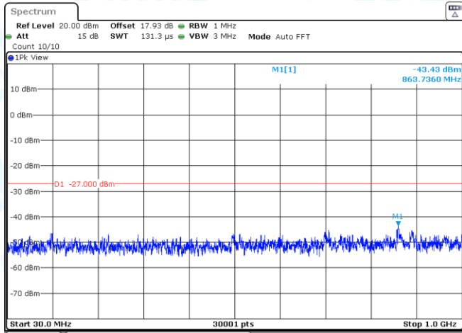
11N40SISO-Ant2-5310-30~1000-PASS
