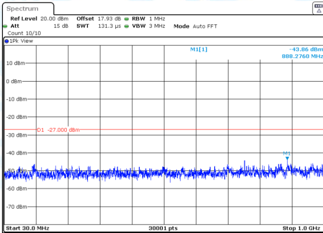
11AC20SISO-Ant2-5280-30~1000-PASS
