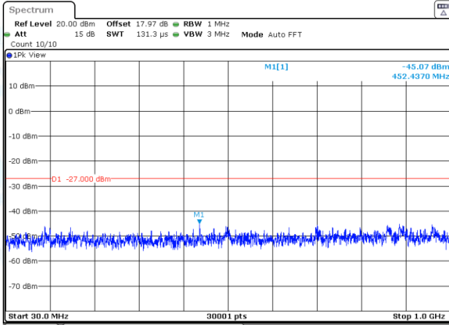
11AC20SISO-Ant2-5260-30~1000-PASS
