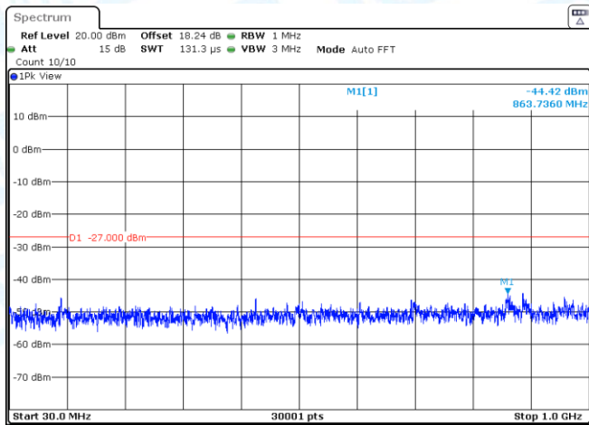
11N20SISO-Ant2-5785-30~1000-PASS
