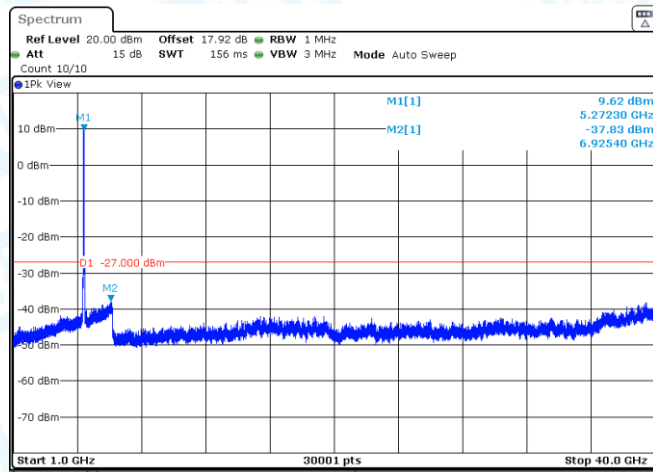
11N40SISO-Ant2-5230-1000~40000-PASS
