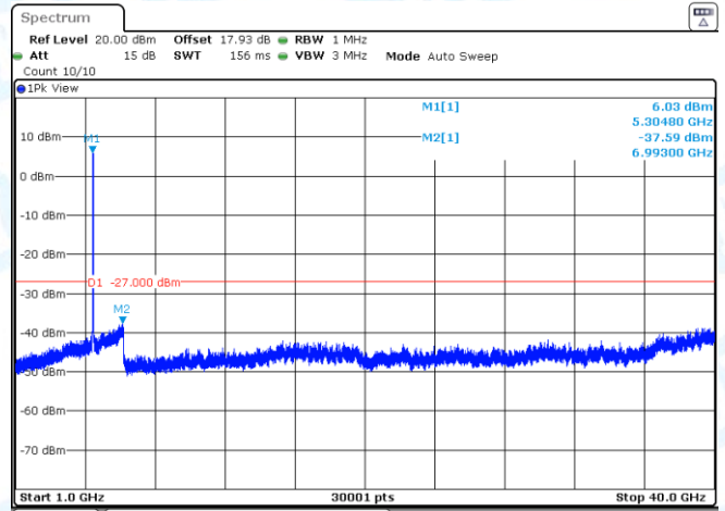
11N40SISO-Ant2-5310-1000~40000-PASS
