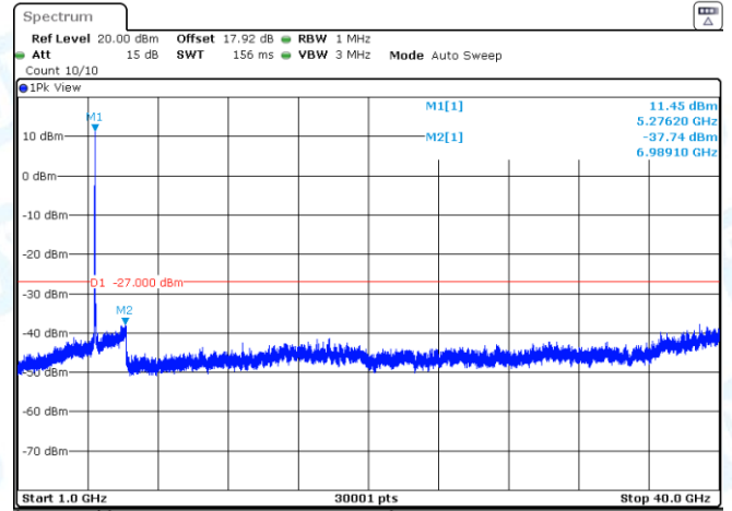
11AC20SISO-Ant2-5260-1000~40000-PASS
