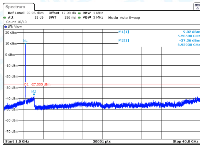
11N40SISO-Ant2-5190-1000~40000-PASS
