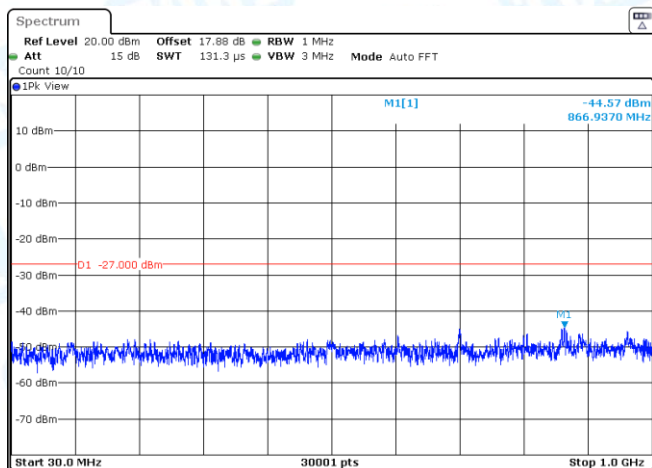
11N40SISO-Ant2-5190-30~1000-PASS
