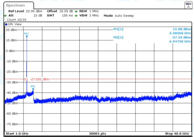
11AC20SISO-Ant2-5500-1000~40000-PASS
