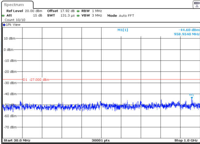
11N20SISO-Ant2-5260-30~1000-PASS
