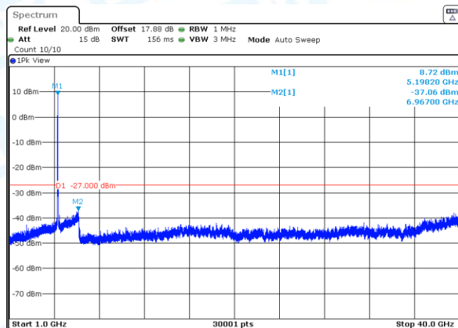
11N40SISO-Ant2-5190-1000~40000-PASS
