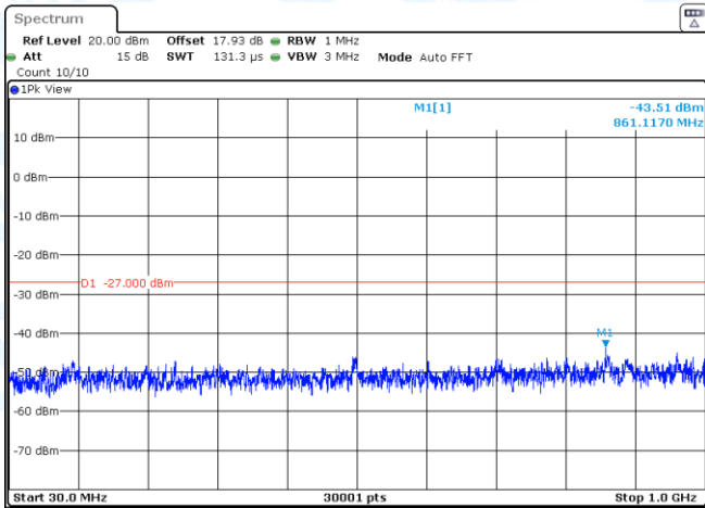
11N20SISO-Ant2-5280-30~1000-PASS
