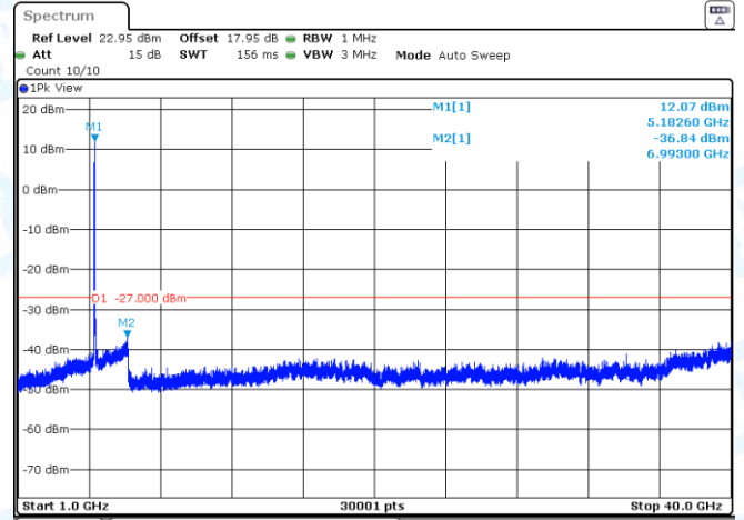
11AC20SISO-Ant2-5180-1000~40000-PASS
