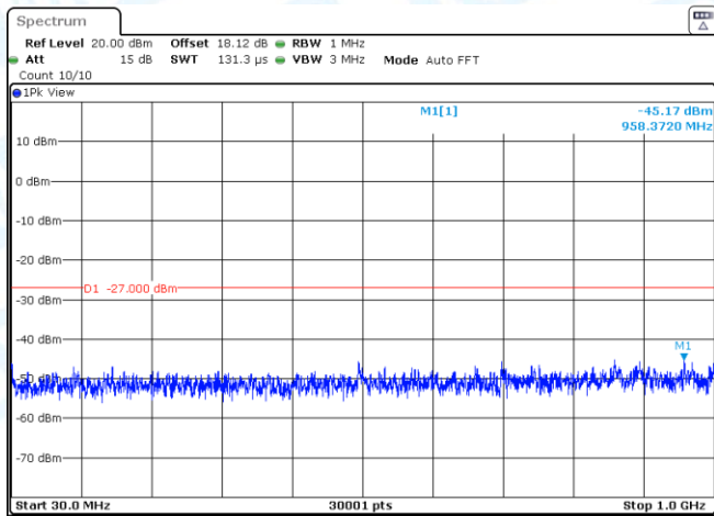
11N40SISO-Ant2-5510-30~1000-PASS
