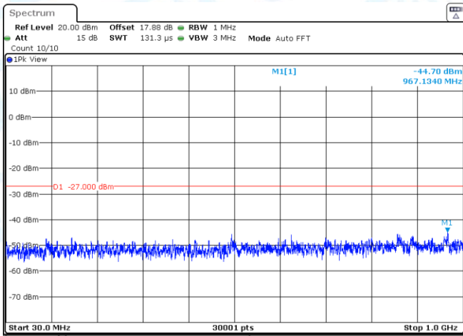
11N20SISO-Ant2-5180-30~1000-PASS
