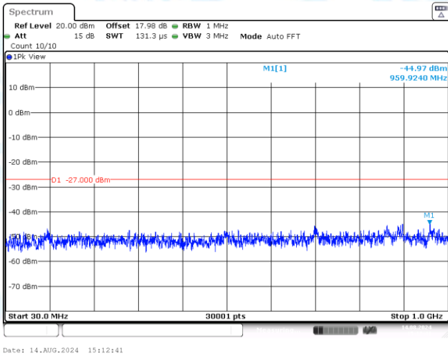
11A-Ant2-5240-30~1000-PASS
