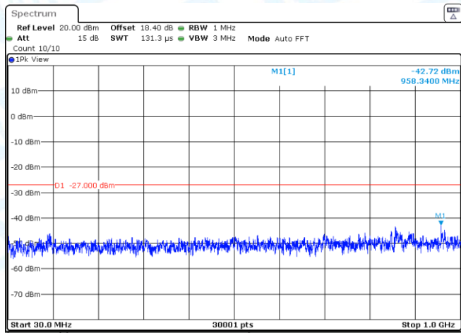
11N20SISO-Ant2-5580-30~1000-PASS
