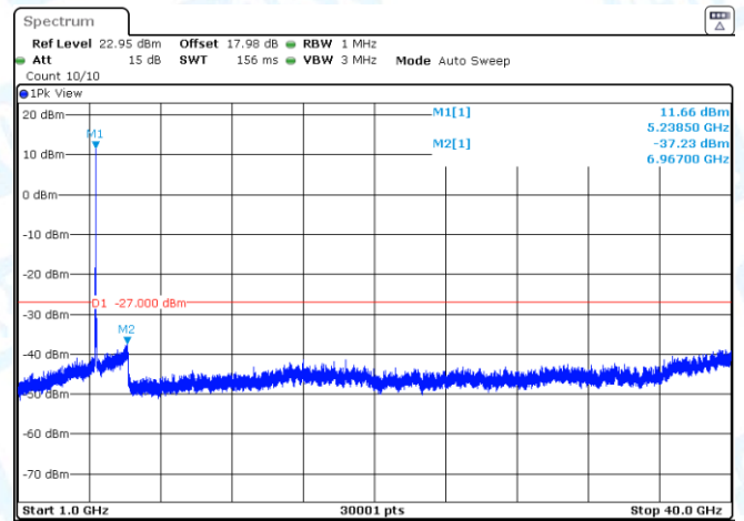
11N20SISO-Ant2-5200-1000~40000-PASS
