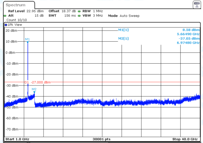
11N40SISO-Ant2-5670-1000~40000-PASS
