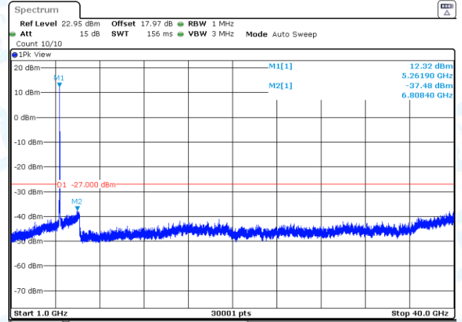
11N20SISO-Ant2-5260-1000~40000-PASS
