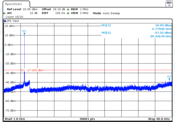
11AC20SISO-Ant2-5745-1000~40000-PASS
