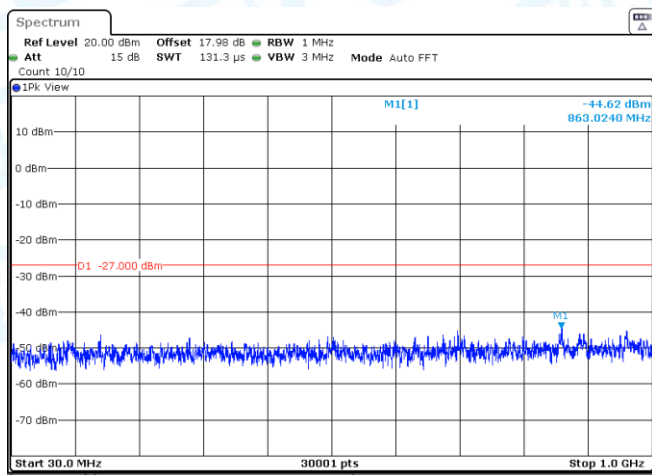
11N40SISO-Ant2-5190-30~1000-PASS
