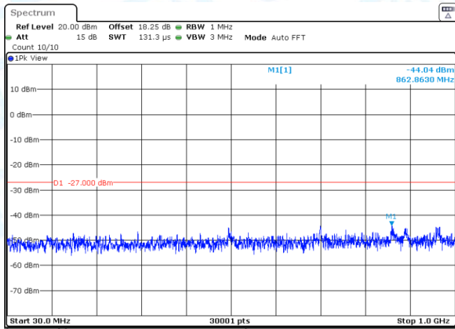
11N40SISO-Ant2-5670-30~1000-PASS
