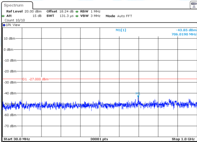
11AC20SISO-Ant2-5785-30~1000-PASS
