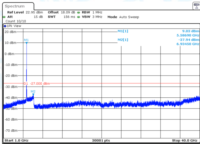
11N20SISO-Ant2-5500-1000~40000-PASS
