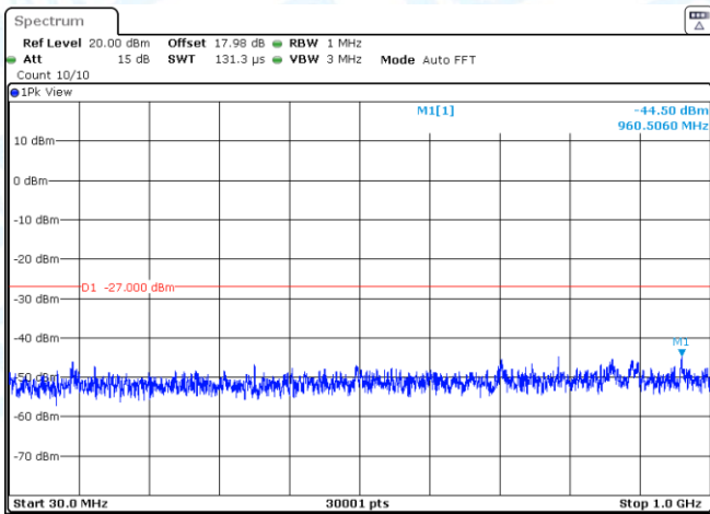
11N20SISO-Ant2-5200-30~1000-PASS
