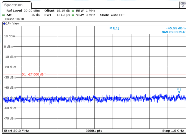
11N40SISO-Ant2-5755-30~1000-PASS
