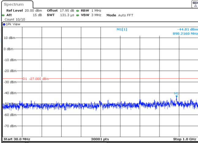
11AC20SISO-Ant2-5180-30~1000-PASS
