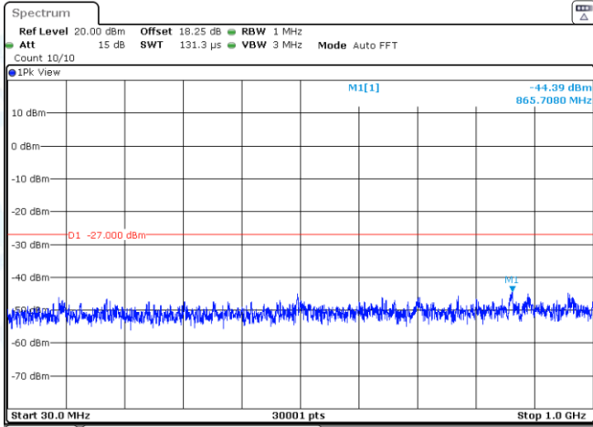
11AC20SISO-Ant2-5745-30~1000-PASS
