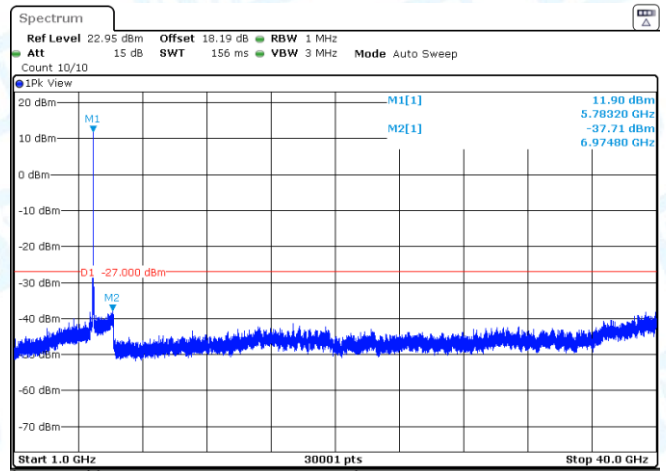
11N20SISO-Ant2-5745-1000~40000-PASS
