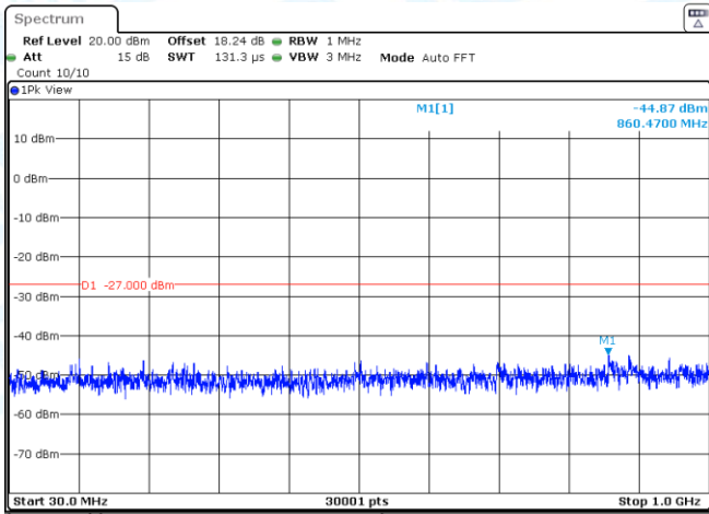
11A-Ant2-5785-30~1000-PASS
